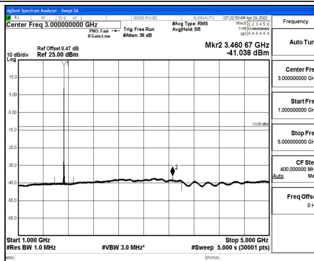
Band4-5MHz-QPSK-20175-1-0-Low-1000-5000--41.04-PASS
