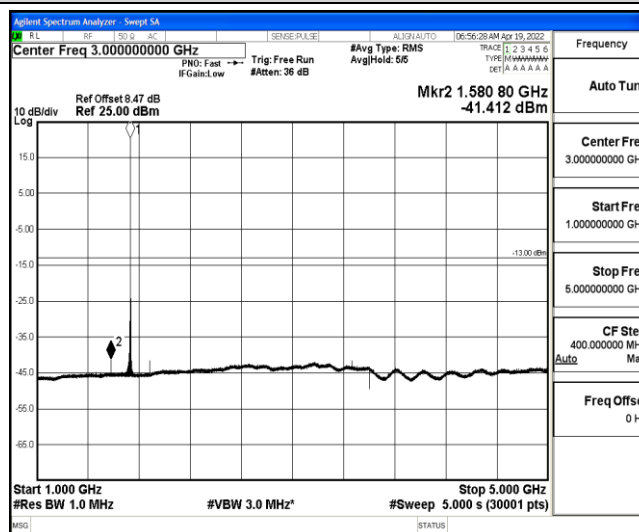
Band4-3MHz-16QAM-20175-1-0-Low-1000-5000--41.41-PASS
