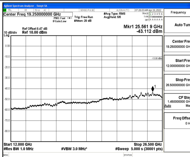
Band4-5MHz-16QAM-20175-1-0-Low-12000-26500--43.11-PASS
