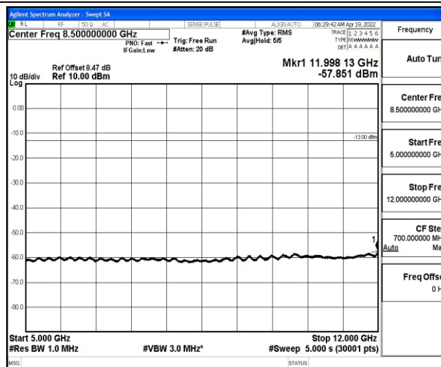
Band4-1.4MHz-16QAM-20175-1-0-Low-5000-12000--57.85-PASS
