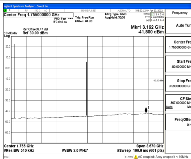
Band4-20MHz-QPSK-20300-6-0-Low--41.80-PASS
