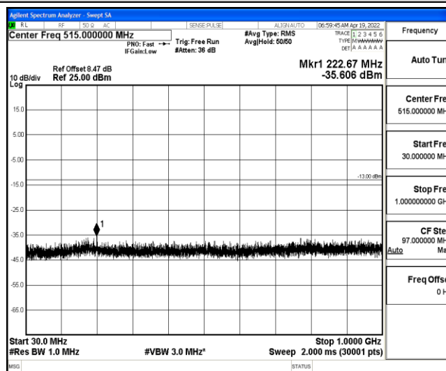
Band4-3MHz-16QAM-20385-1-0-High-30-1000--35.61-PASS
