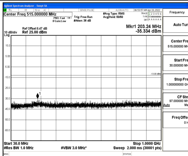
Band4-3MHz-QPSK-20175-1-0-Low-30-1000--35.33-PASS
