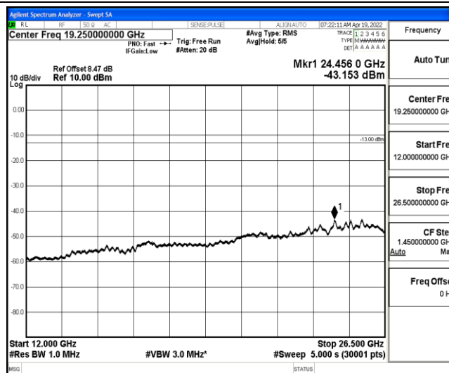
Band4-5MHz-16QAM-19975-1-0-Low-12000-26500--43.15-PASS
