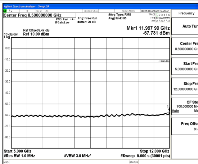
Band4-3MHz-QPSK-20175-1-0-Low-5000-12000--57.73-PASS
