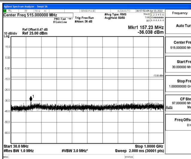
Band4-3MHz-QPSK-20385-1-0-High-30-1000--36.04-PASS
