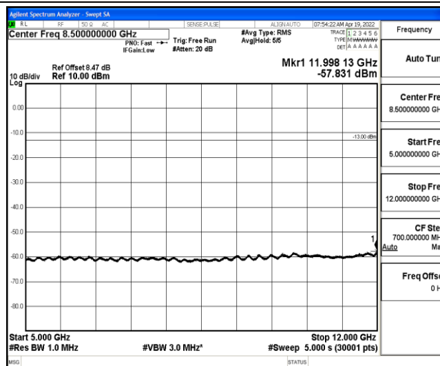
Band4-10MHz-QPSK-20175-1-0-Low-5000-12000--57.83-PASS
