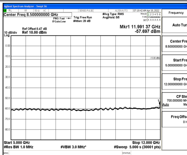
Band4-5MHz-QPSK-19975-1-0-Low-5000-12000--57.7-PASS
