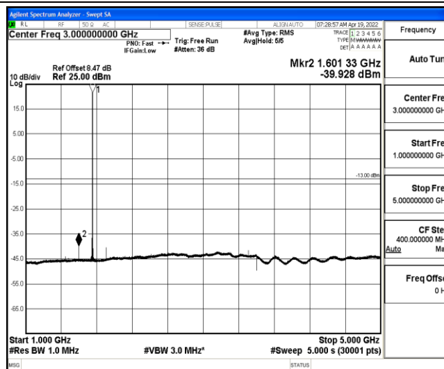
Band4-5MHz-16QAM-20375-1-0-High-1000-5000--39.93-PASS
