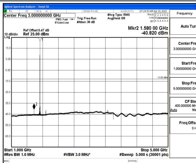
Band4-5MHz-16QAM-20175-1-0-Low-1000-5000--40.82-PASS
