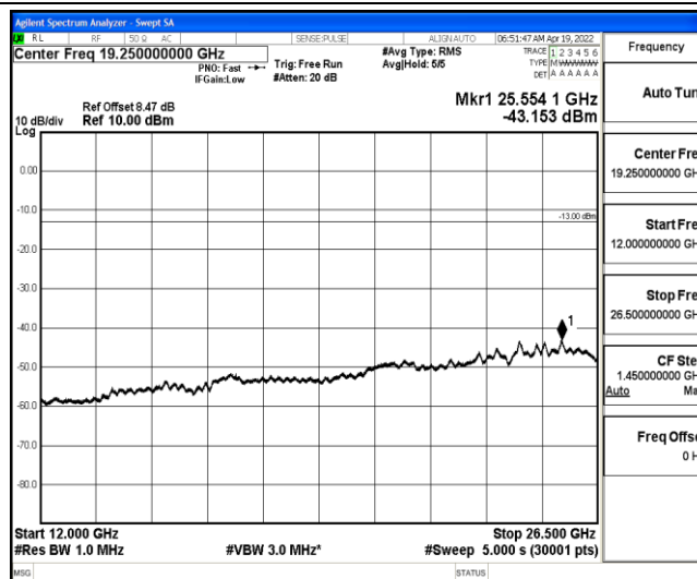
Band4-3MHz-QPSK-19965-1-0-Low-12000-26500--43.15-PASS
