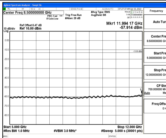
Band4-5MHz-QPSK-20375-1-0-High-5000-12000--57.91-PASS
