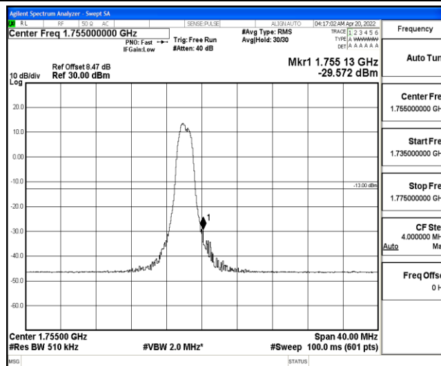
Band4-20MHz-QPSK-20300-6-0-High--29.57-PASS
