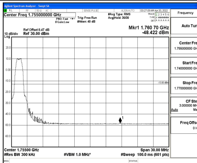
Band4-15MHz-16QAM-20325-6-0-Low--48.42-PASS
