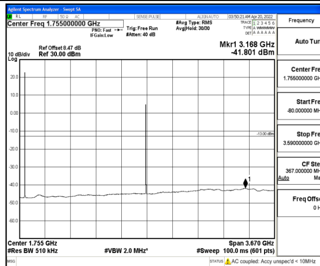
Band4-20MHz-16QAM-20300-6-0-Low--41.80-PASS
