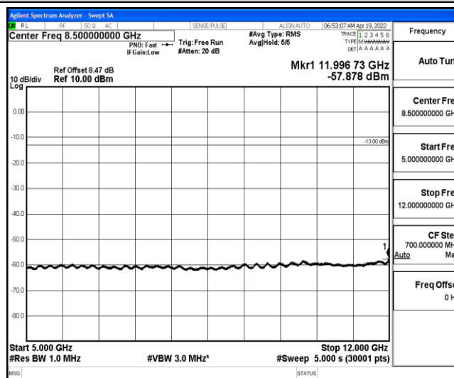
Band4-3MHz-16QAM-19965-1-0-Low-5000-12000--57.88-PASS
