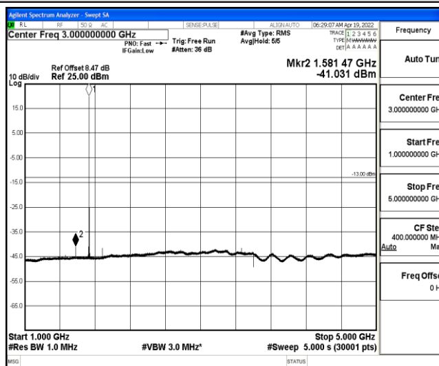
Band4-1.4MHz-16QAM-20175-1-0-Low-1000-5000--41.03-PASS
