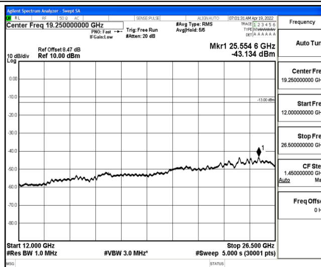
Band4-3MHz-16QAM-20385-1-0-High-12000-26500--43.13-PASS
