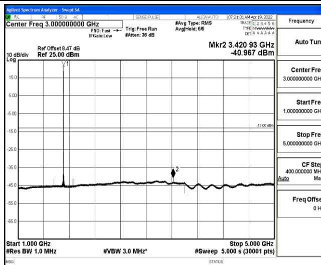
Band4-5MHz-16QAM-19975-1-0-Low-1000-5000--40.97-PASS
