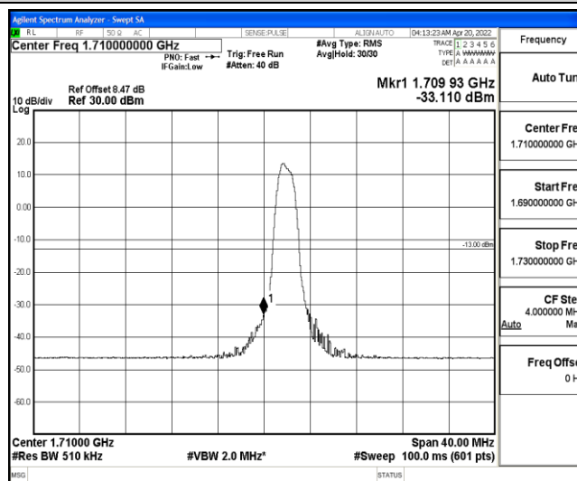
Band4-20MHz-16QAM-20050-6-0-Low--33.11-PASS
