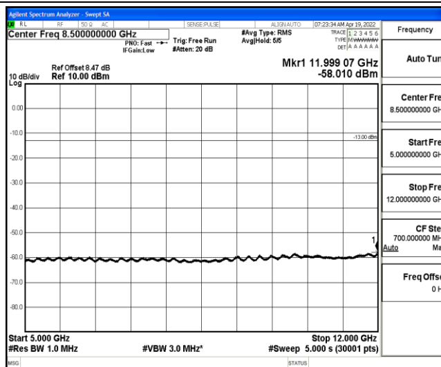
Band4-5MHz-QPSK-20175-1-0-Low-5000-12000--58.01-PASS
