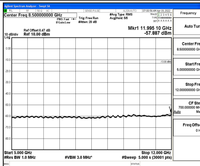
Band4-3MHz-16QAM-20385-1-0-High-5000-12000--57.89-PASS
