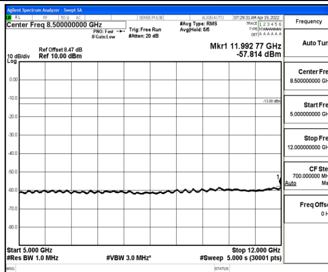
Band4-5MHz-16QAM-20375-1-0-High-5000-12000--57.81-PASS
