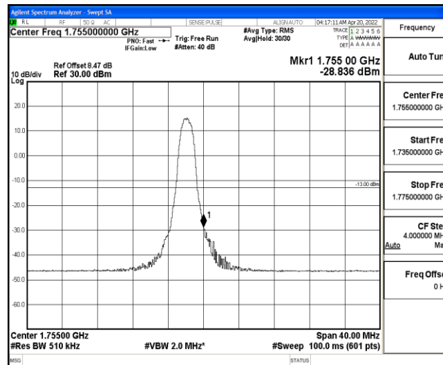
Band4-20MHz-16QAM-20300-6-0-High--28.84-PASS
