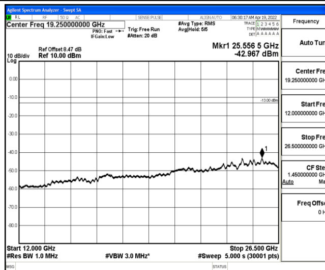
Band4-1.4MHz-16QAM-20175-1-0-Low-12000-26500--42.97-PASS
