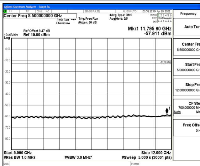
Band4-3MHz-QPSK-19965-1-0-Low-5000-12000--57.91-PASS
