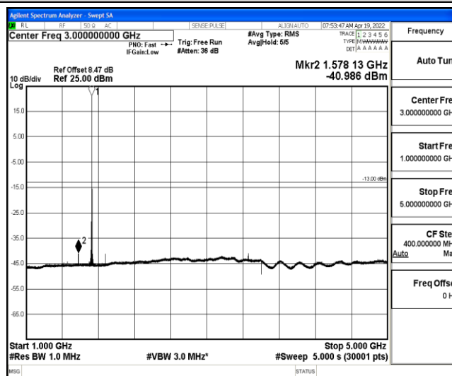
Band4-10MHz-QPSK-20175-1-0-Low-1000-5000--40.99-PASS
