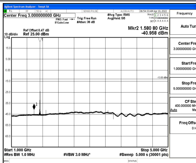
Band4-3MHz-QPSK-20175-1-0-Low-1000-5000--40.96-PASS
