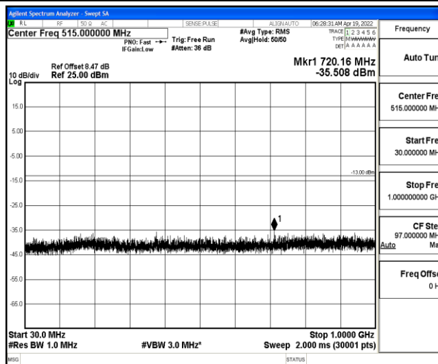
Band4-1.4MHz-16QAM-20175-1-0-Low-30-1000--35.51-PASS
