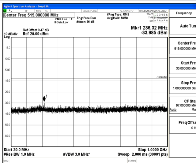
Band4-5MHz-16QAM-19975-1-0-Low-30-1000--33.99-PASS
