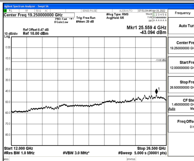
Band4-10MHz-QPSK-20000-1-0-Low-12000-26500--43.09-PASS
