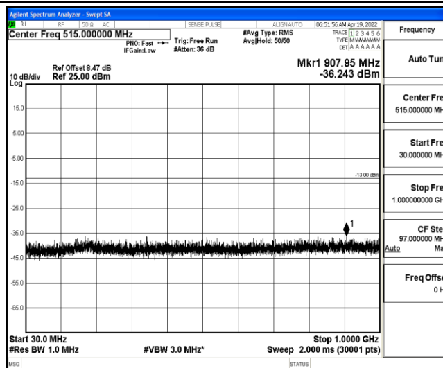
Band4-3MHz-16QAM-19965-1-0-Low-30-1000--36.24-PASS
