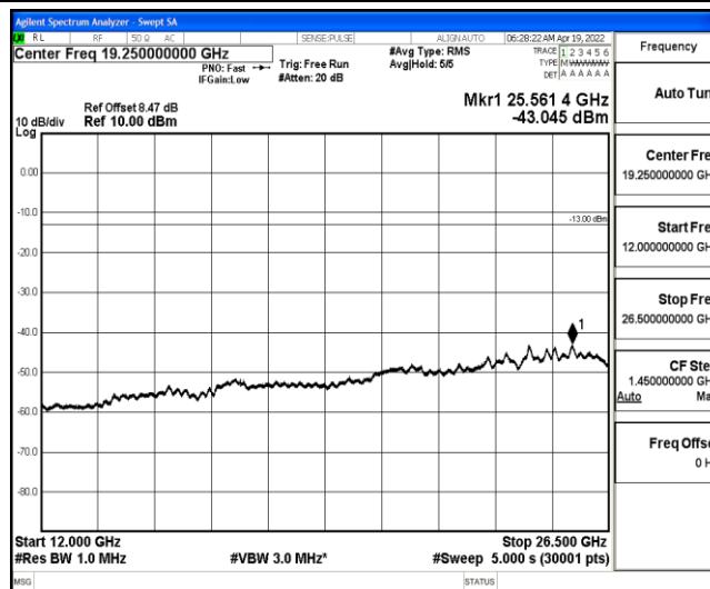
Band4-1.4MHz-QPSK-20175-1-0-Low-12000-26500--43.05-PASS
