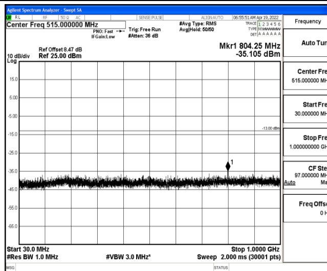
Band4-3MHz-16QAM-20175-1-0-Low-30-1000--35.11-PASS
