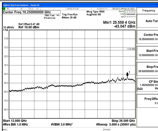
Band4-1.4MHz-16QAM-19957-1-0-Low-12000-26500--43.05-PASS
