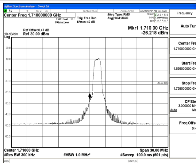
Band4-15MHz-16QAM-20025-6-0-Low--26.22-PASS
