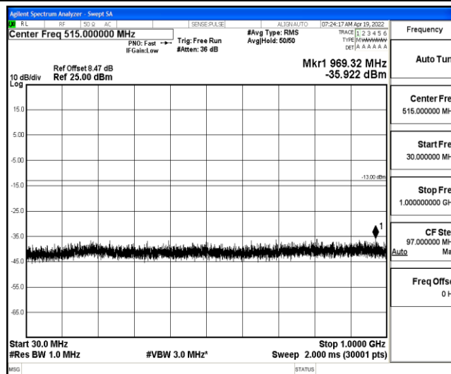
Band4-5MHz-16QAM-20175-1-0-Low-30-1000--35.92-PASS
