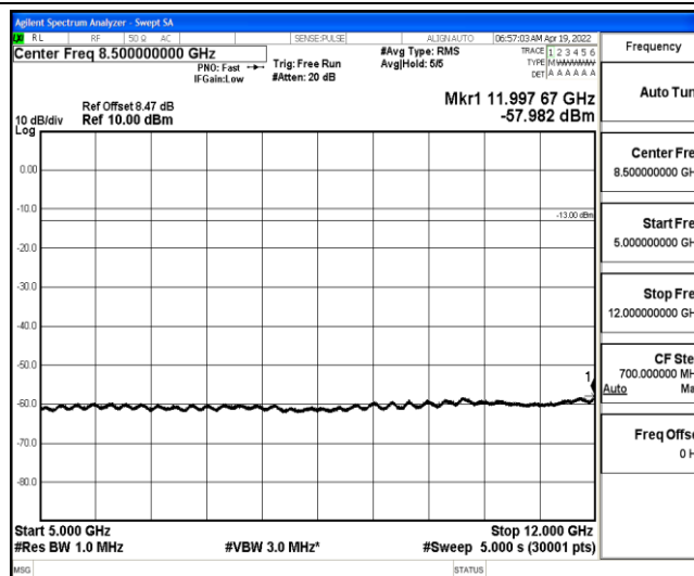
Band4-3MHz-16QAM-20175-1-0-Low-5000-12000--57.98-PASS
