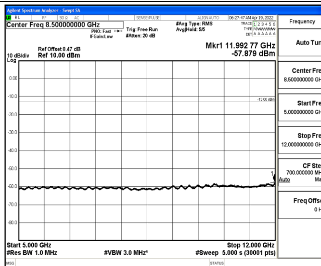
Band4-1.4MHz-QPSK-20175-1-0-Low-5000-12000--57.88-PASS
