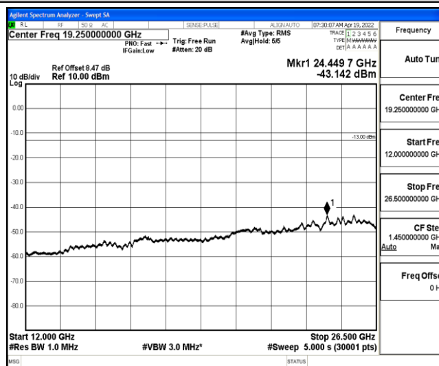
Band4-5MHz-16QAM-20375-1-0-High-12000-26500--43.14-PASS
