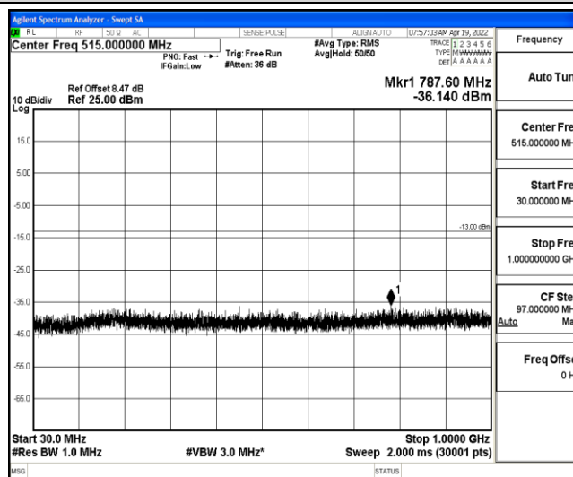
Band4-10MHz-QPSK-20350-1-0-High-30-1000--36.14-PASS
