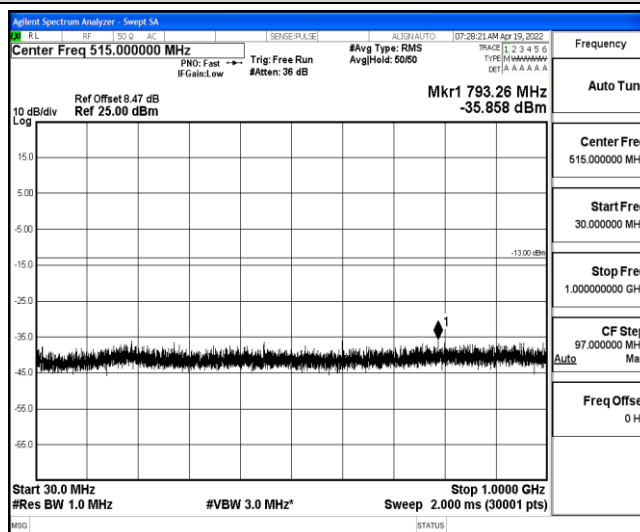
Band4-5MHz-16QAM-20375-1-0-High-30-1000--35.86-PASS
