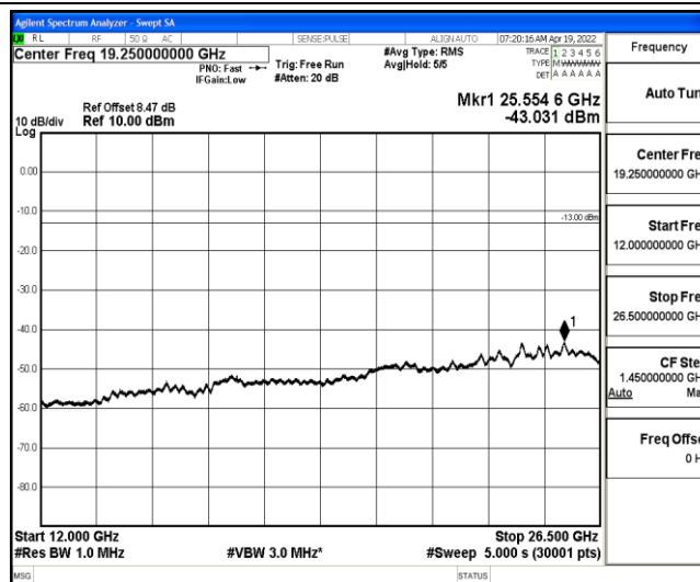
Band4-5MHz-QPSK-19975-1-0-Low-12000-26500--43.03-PASS
