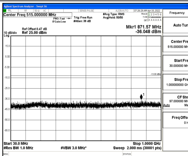
Band4-5MHz-QPSK-20375-1-0-High-30-1000--36.05-PASS
