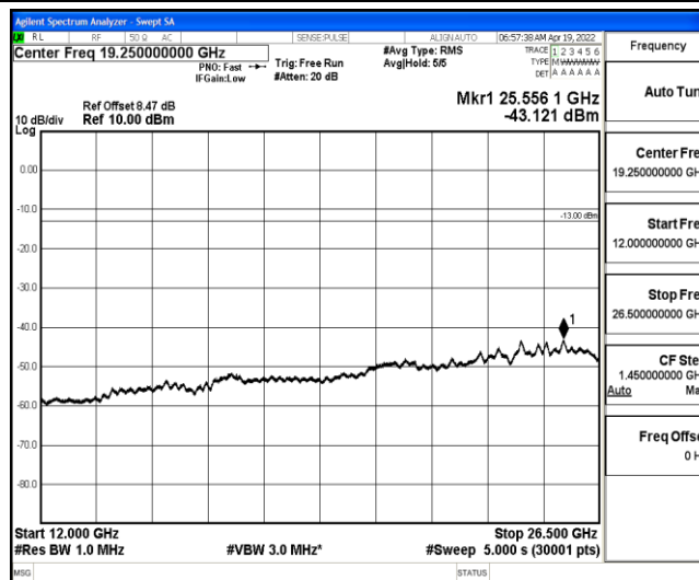
Band4-3MHz-16QAM-20175-1-0-Low-12000-26500--43.12-PASS
