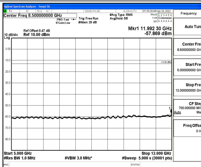
Band4-5MHz-16QAM-20175-1-0-Low-5000-12000--57.87-PASS
