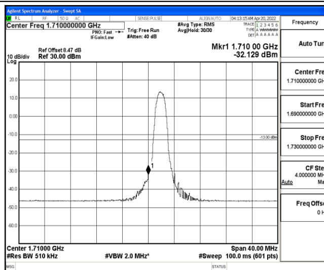
Band4-20MHz-QPSK-20050-6-0-Low--32.13-PASS
