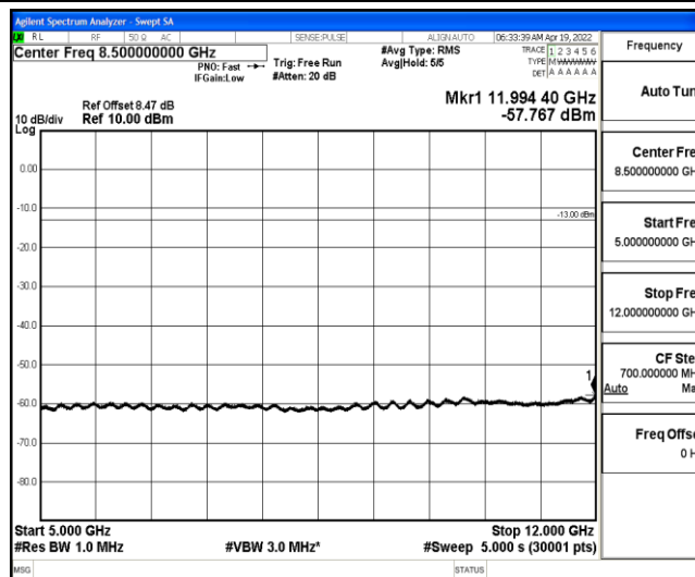
Band4-1.4MHz-16QAM-20393-1-0-High-5000-12000--57.77-PASS
