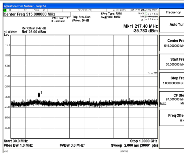
Band4-5MHz-QPSK-19975-1-0-Low-30-1000--35.78-PASS
