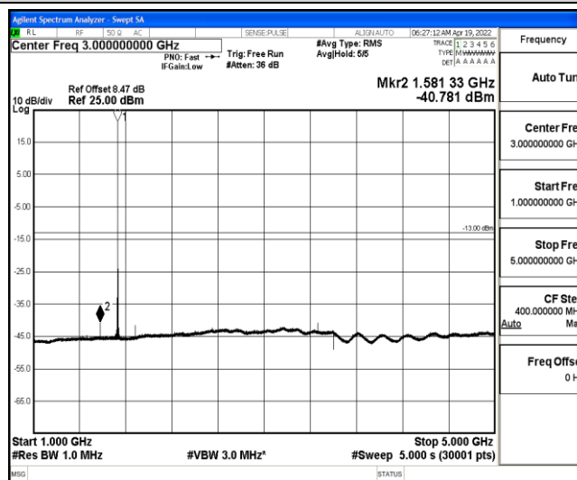
Band4-1.4MHz-QPSK-20175-1-0-Low-1000-5000--40.78-PASS
