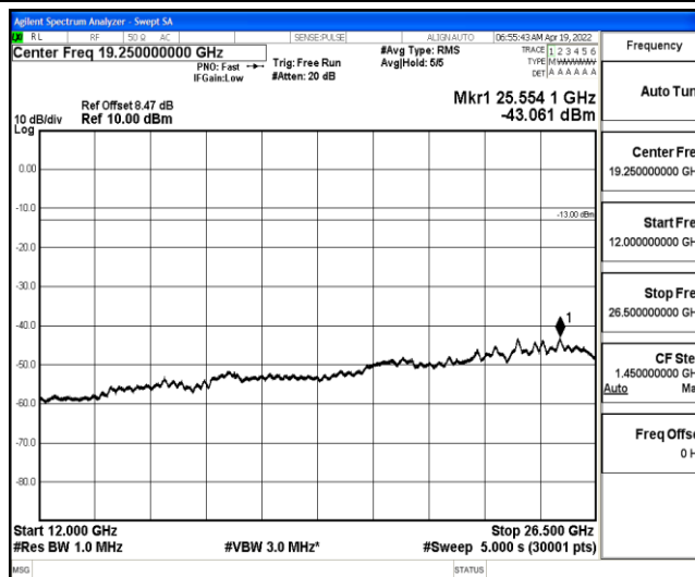
Band4-3MHz-QPSK-20175-1-0-Low-12000-26500--43.06-PASS
