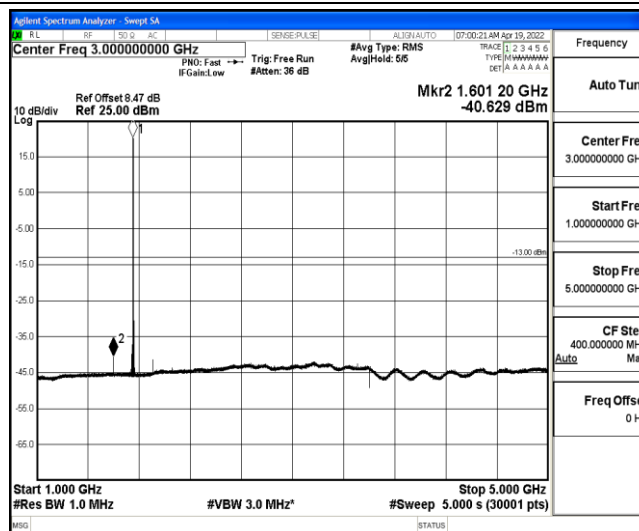
Band4-3MHz-16QAM-20385-1-0-High-1000-5000--40.63-PASS
