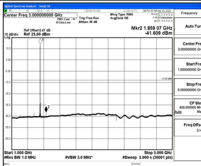
Band4-3MHz-16QAM-19965-1-0-Low-1000-5000--41.61-PASS
