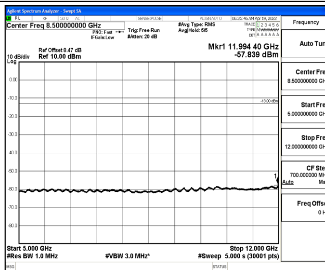
Band4-1.4MHz-16QAM-19957-1-0-Low-5000-12000--57.84-PASS
