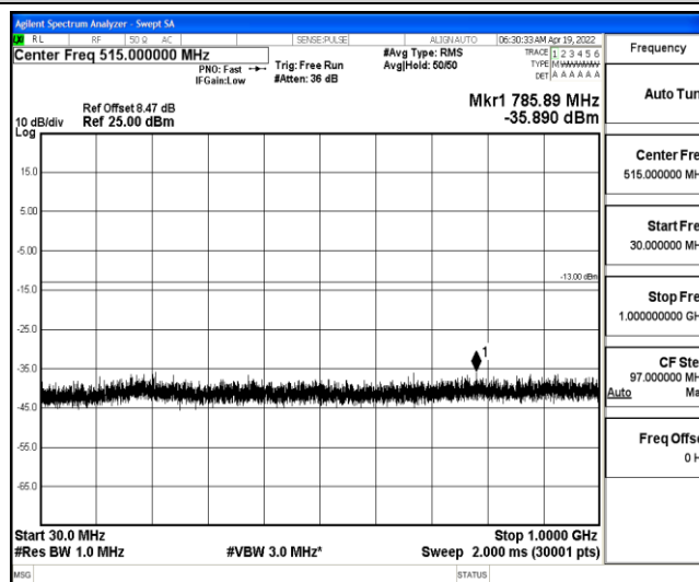
Band4-1.4MHz-QPSK-20393-1-0-High-30-1000--35.89-PASS
