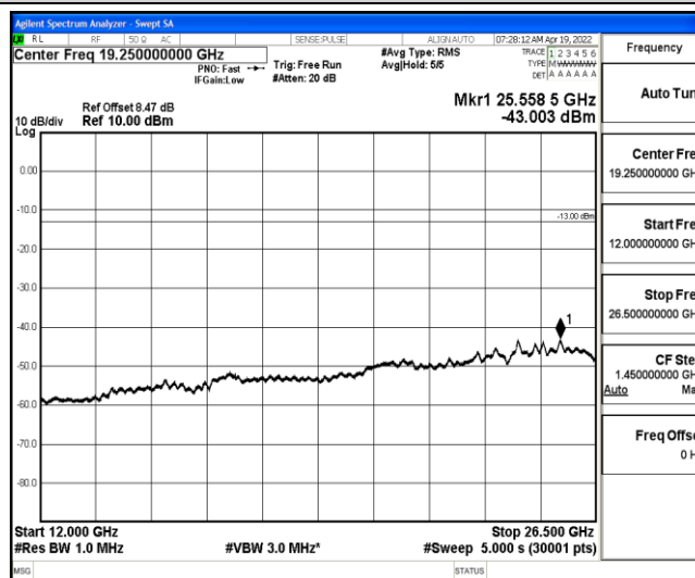
Band4-5MHz-QPSK-20375-1-0-High-12000-26500--43-PASS
