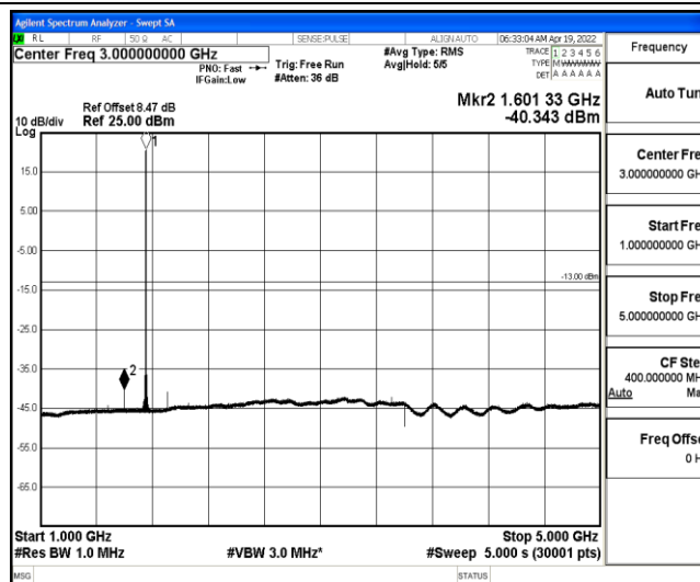
Band4-1.4MHz-16QAM-20393-1-0-High-1000-5000--40.34-PASS
