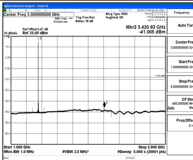
Band4-3MHz-QPSK-19965-1-0-Low-1000-5000--41.01-PASS
