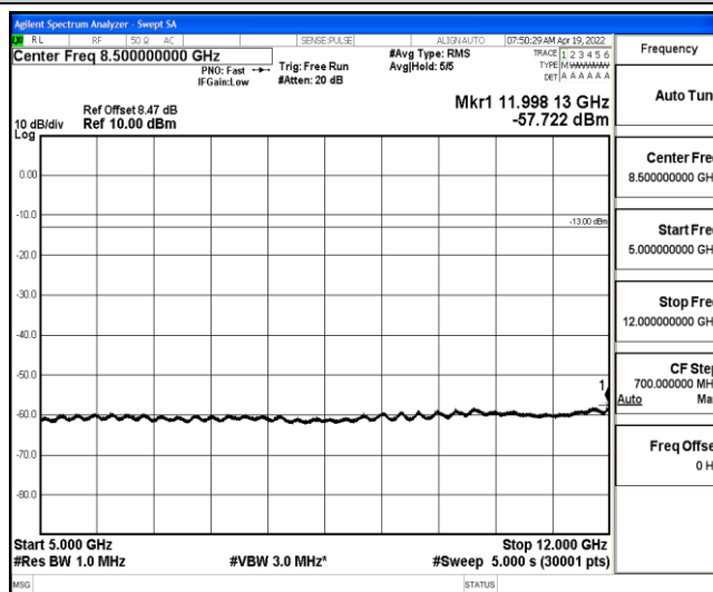
Band4-10MHz-QPSK-20000-1-0-Low-5000-12000--57.72-PASS
