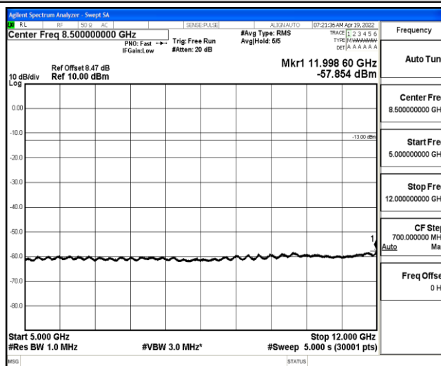
Band4-5MHz-16QAM-19975-1-0-Low-5000-12000--57.85-PASS
