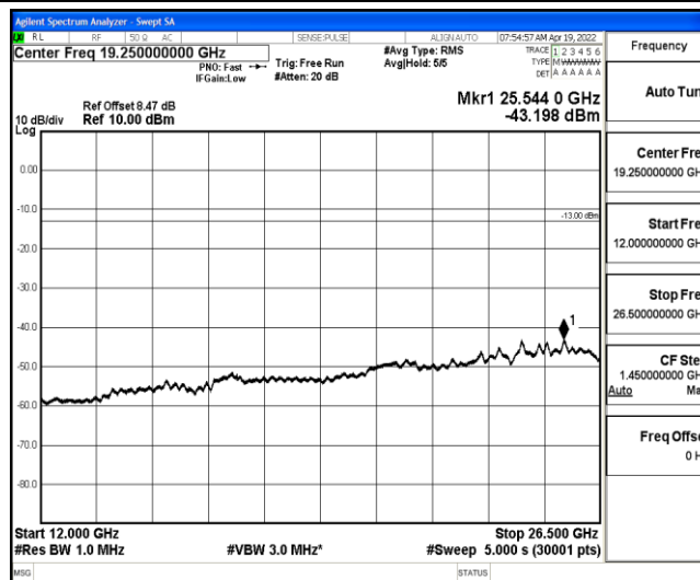
Band4-10MHz-QPSK-20175-1-0-Low-12000-26500--43.2-PASS
