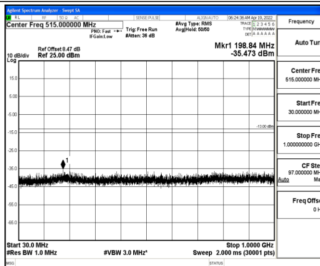
Band4-1.4MHz-16QAM-19957-1-0-Low-30-1000--35.47-PASS
