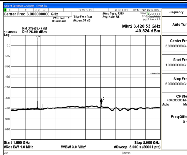
Band4-5MHz-QPSK-19975-1-0-Low-1000-5000--40.82-PASS
