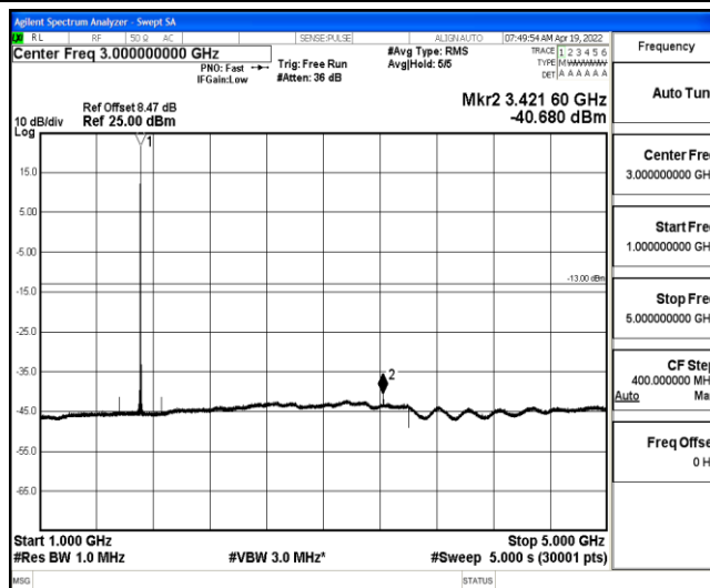
Band4-10MHz-QPSK-20000-1-0-Low-1000-5000--40.68-PASS
