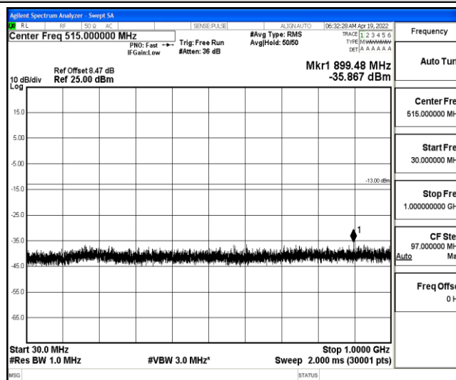
Band4-1.4MHz-16QAM-20393-1-0-High-30-1000--35.87-PASS
