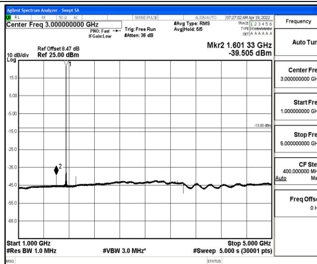
Band4-5MHz-QPSK-20375-1-0-High-1000-5000--39.51-PASS
