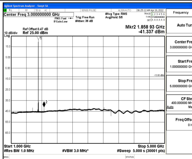
Band4-1.4MHz-16QAM-19957-1-0-Low-1000-5000--41.34-PASS
