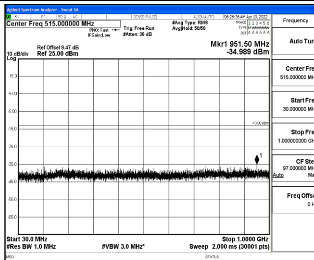
Band4-1.4MHz-QPSK-20175-1-0-Low-30-1000--34.99-PASS
