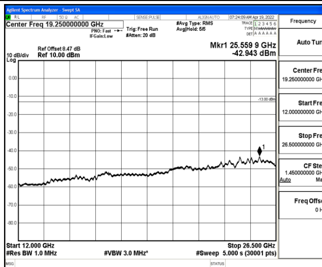
Band4-5MHz-QPSK-20175-1-0-Low-12000-26500--42.94-PASS
