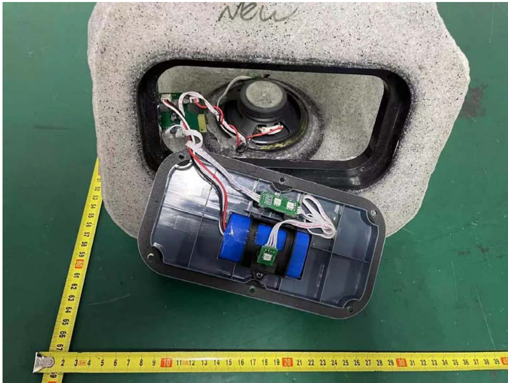
Internal photos M/N: ITSBO-L513
