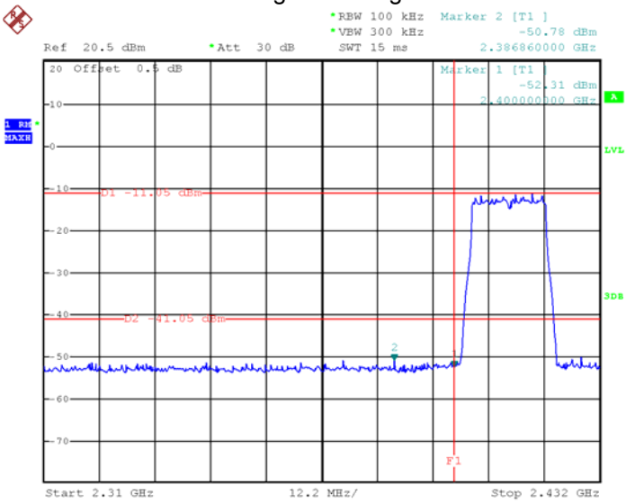
TX 11g: Band edge-left side
