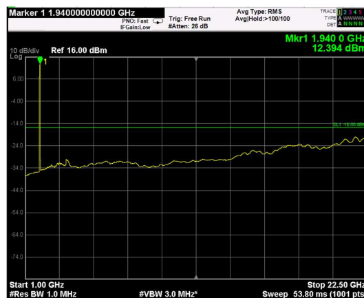
Channel: BOTTOM, Modulation: 64QAM, BW=20MHz, Range: Upper
