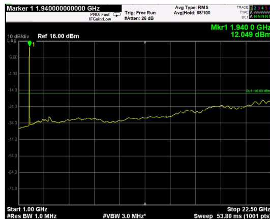
Channel: BOTTOM, Modulation: 16QAM, BW=20MHz, Range: Upper
