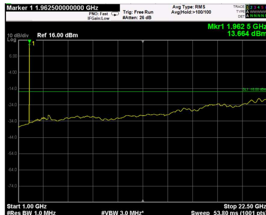
Channel: MIDDLE, Modulation: 16QAM, BW=20MHz, Range: Upper
