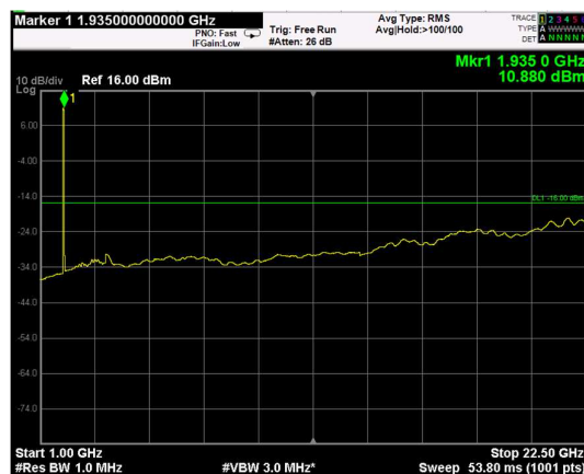
Channel: BOTTOM, Modulation: 16QAM, BW=10MHz, Range: Upper
