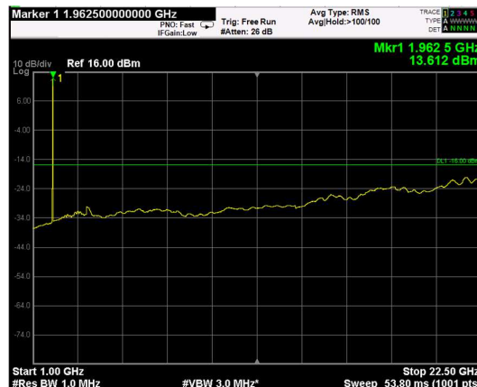
Channel: MIDDLE, Modulation: 16QAM, BW=15MHz, Range: Upper
