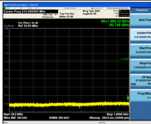
Band4-3MHz-QPSK-20175-1-0-Low-30-1000--60.75-PASS
