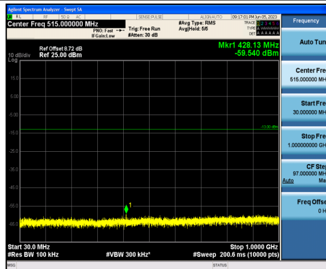
Band2-20MHz-16QAM-18700-1-0-Low-30-1000--59.54-PASS
