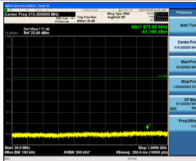
Band4-1.4MHz-16QAM-19957-1-0-Low-30-1000--61.17-PASS
