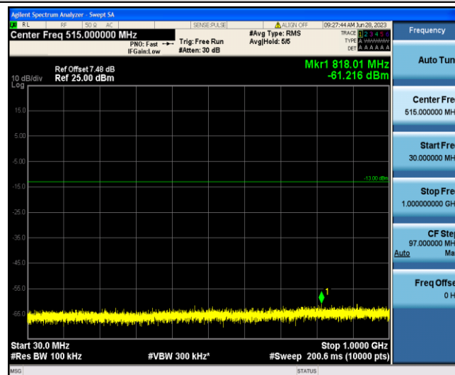
Band4-5MHz-QPSK-20175-1-0-Low-30-1000--61.22-PASS
