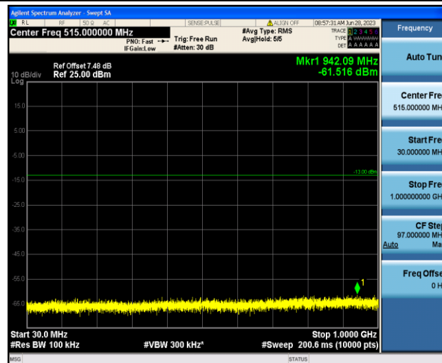
Band4-1.4MHz-QPSK-20175-1-0-Low-30-1000--61.52-PASS
