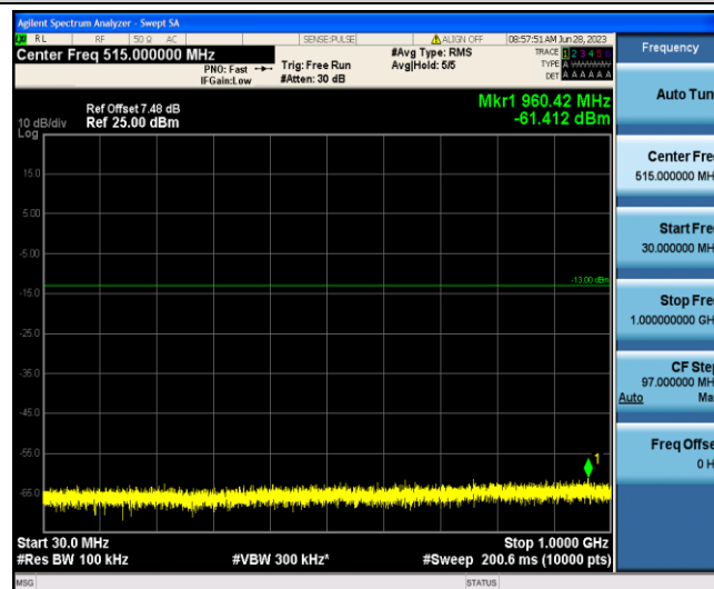
Band4-1.4MHz-16QAM-20175-1-0-Low-30-1000--61.41-PASS
