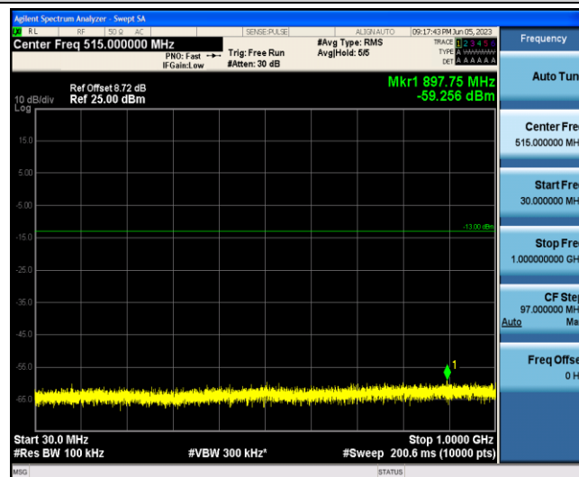
Band2-20MHz-16QAM-18900-1-0-Low-30-1000--59.26-PASS
