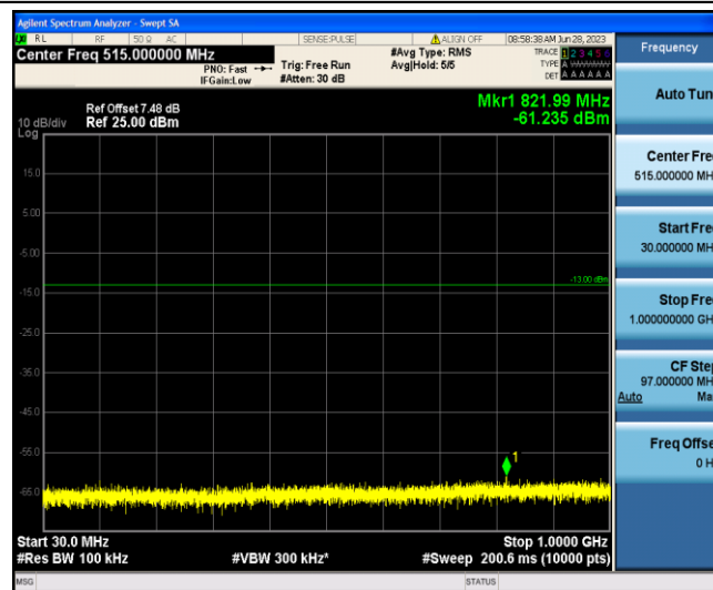
Band4-1.4MHz-16QAM-20393-1-0-Low-30-1000--61.24-PASS
