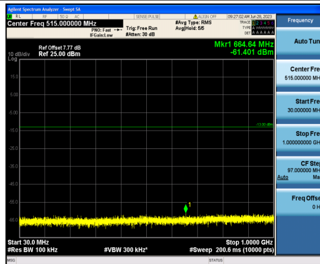
Band4-5MHz-QPSK-19975-1-0-Low-30-1000--61.4-PASS
