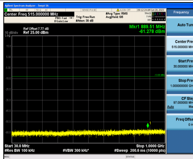
Band4-3MHz-16QAM-19965-1-0-Low-30-1000--61.28-PASS
