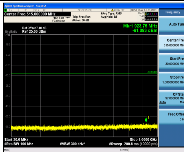
Band4-1.4MHz-QPSK-20393-1-0-Low-30-1000--61.08-PASS
