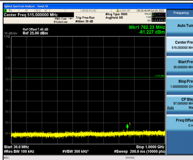
Band4-5MHz-16QAM-20375-1-0-Low-30-1000--61.23-PASS
