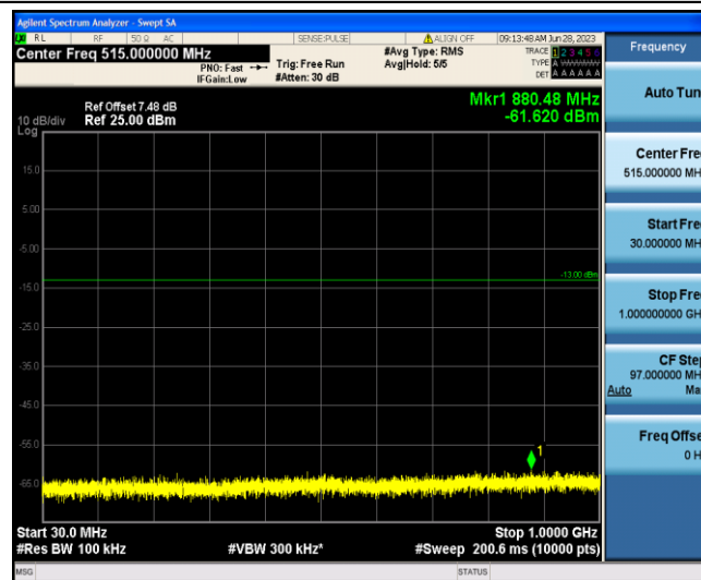
Band4-3MHz-16QAM-20385-1-0-Low-30-1000--61.62-PASS
