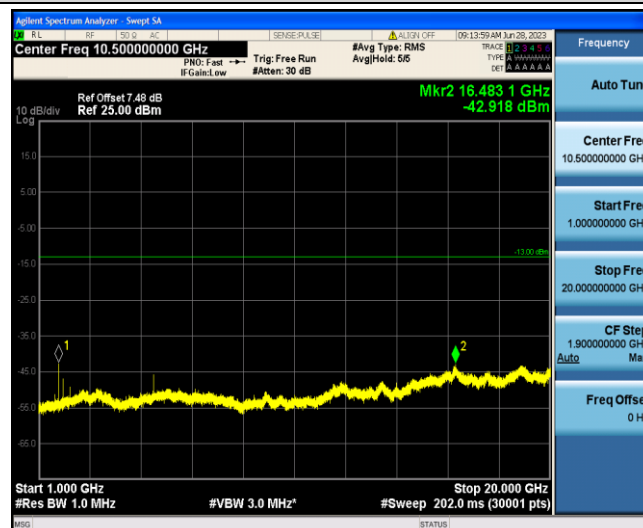
Band4-3MHz-16QAM-20385-1-0-Low-1000-20000--42.92-PASS
