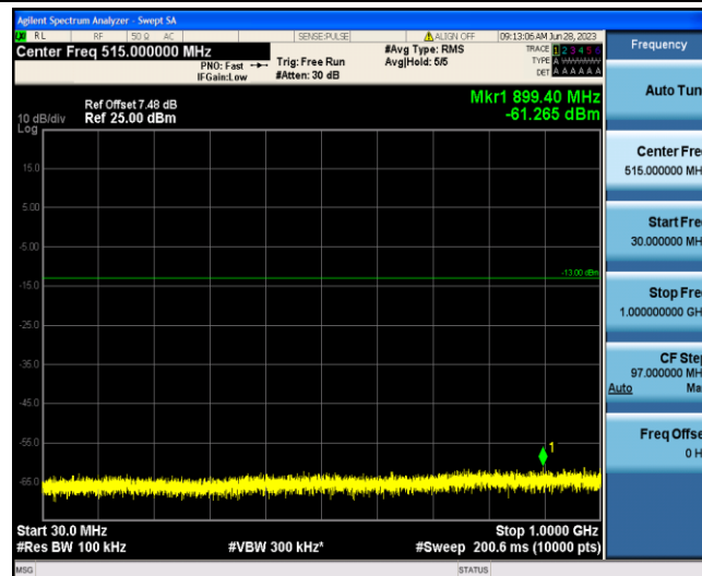
Band4-3MHz-16QAM-20175-1-0-Low-30-1000--61.27-PASS
