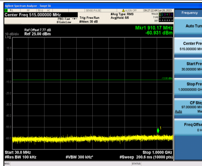
Band4-5MHz-16QAM-19975-1-0-Low-30-1000--60.93-PASS
