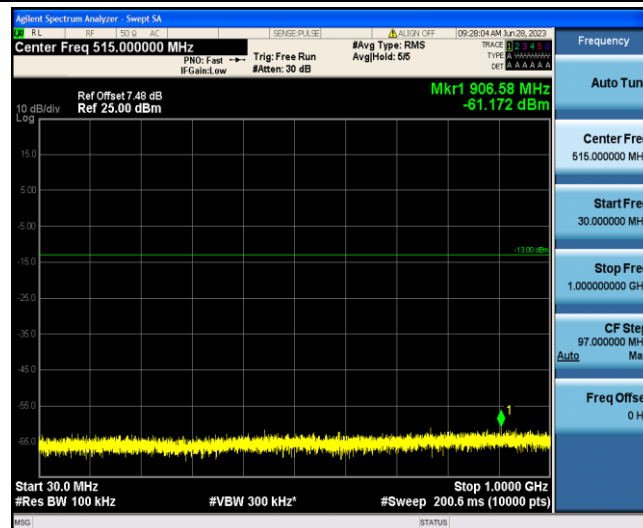
Band4-5MHz-16QAM-20175-1-0-Low-30-1000--61.17-PASS
