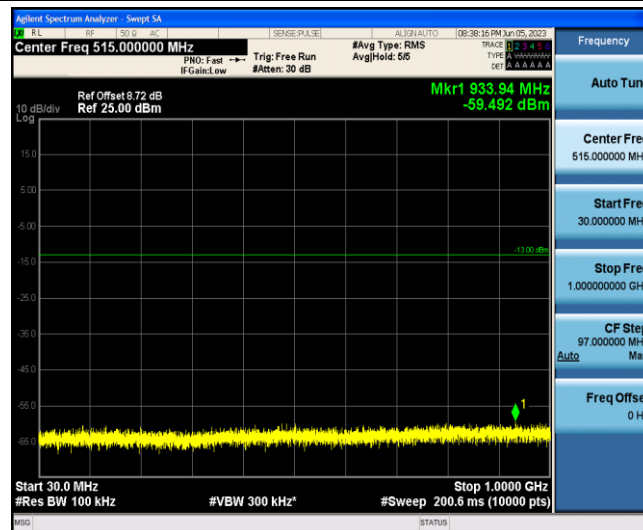
Band2-15MHz-16QAM-18675-1-0-Low-30-1000--59.49-PASS
