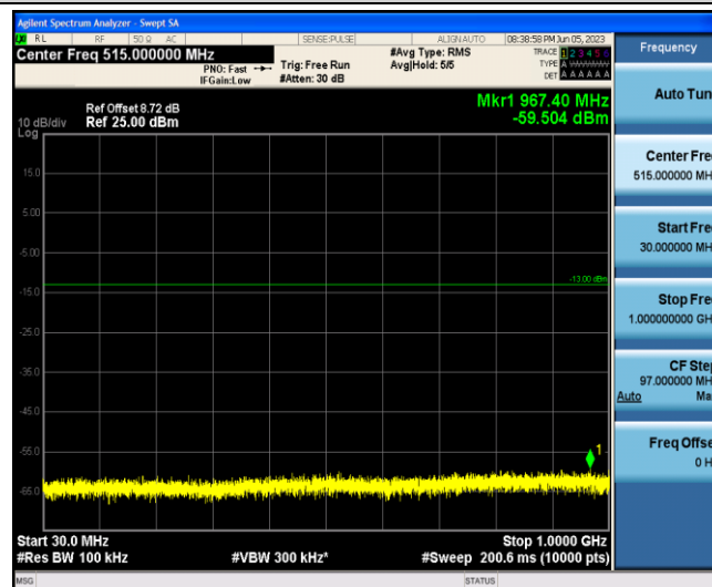
Band2-15MHz-16QAM-18900-1-0-Low-30-1000--59.5-PASS
