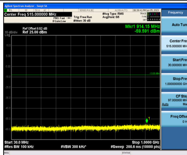
Band2-15MHz-16QAM-19125-1-0-Low-30-1000--59.59-PASS
