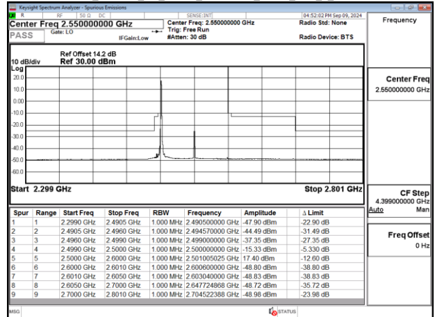
Band41_100MHz_CP_OFDM_SCS30kHz_QPSK_RB1_0_CH510000
