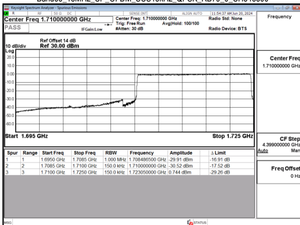
Band66_15MHz_CP_OFDM_SCS15kHz_QPSK_RB79_0_CH343500
