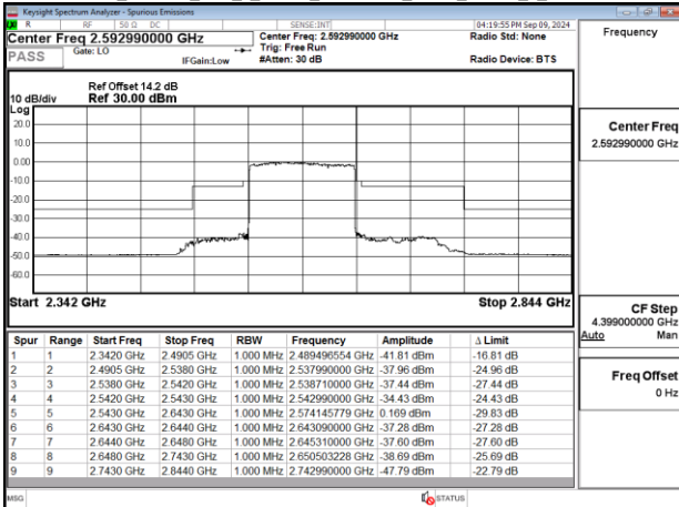
Band41_100MHz_DFT_s_OFDM_SCS30kHz_BPSK_RB270_0_CH518598
