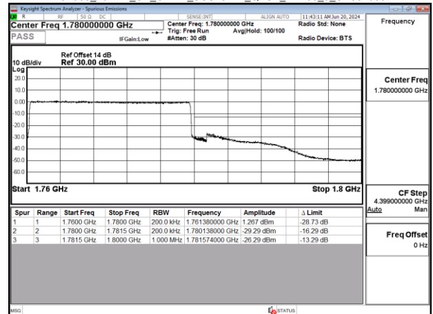
Band66_20MHz_CP_OFDM_SCS15kHz_QPSK_RB106_0_CH354000
