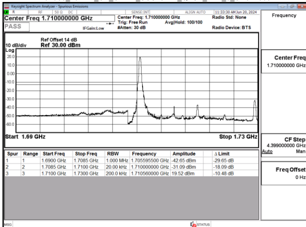
Band66_20MHz_CP_OFDM_SCS15kHz_QPSK_RB1_0_CH344000
