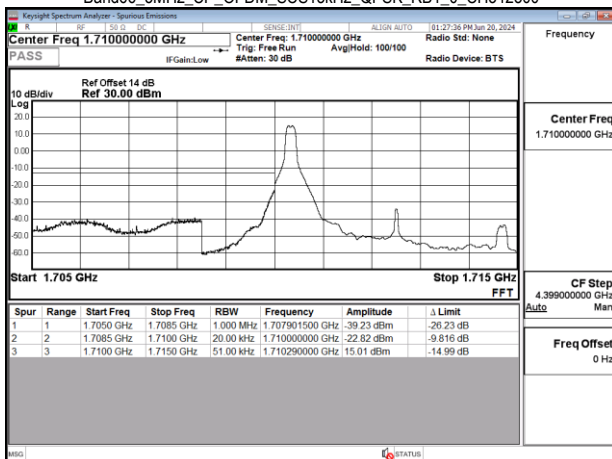
Band66_5MHz_CP_OFDM_SCS15kHz_QPSK_RB1_0_CH342500
