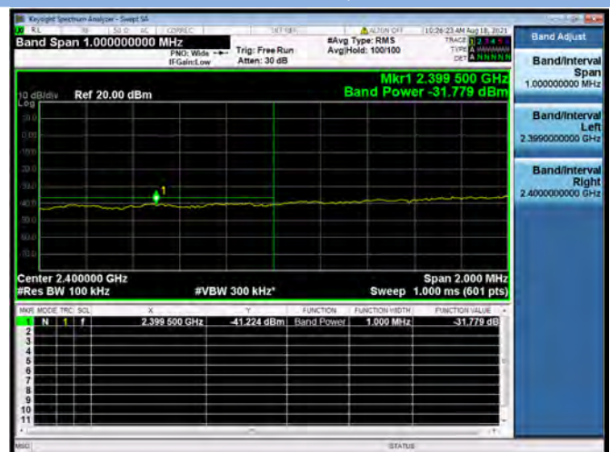
802.11n-20 MHz CHANNEL 1, Reference level
