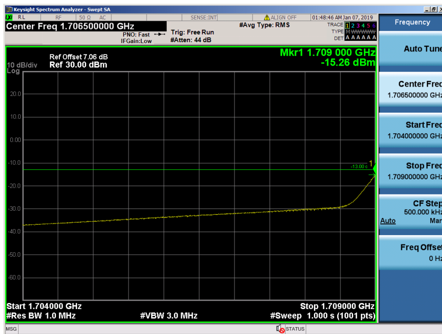
LTE Band 66, 4 / 5MHz / 64QAM Offset/Size (25/0)
