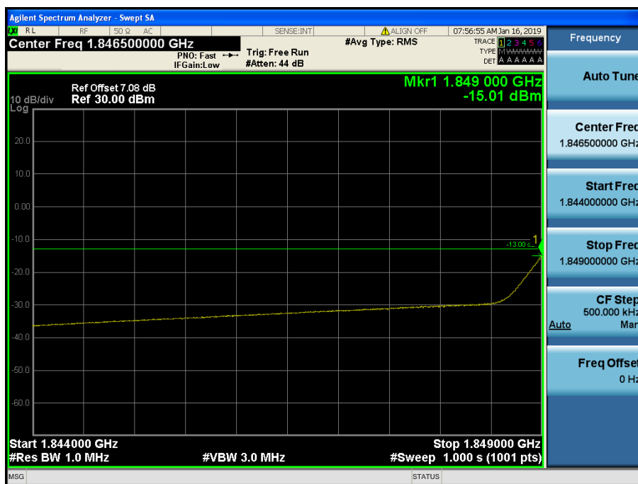
LTE Band 2 / 5MHz / 64QAM Size/Offset (25/0)
