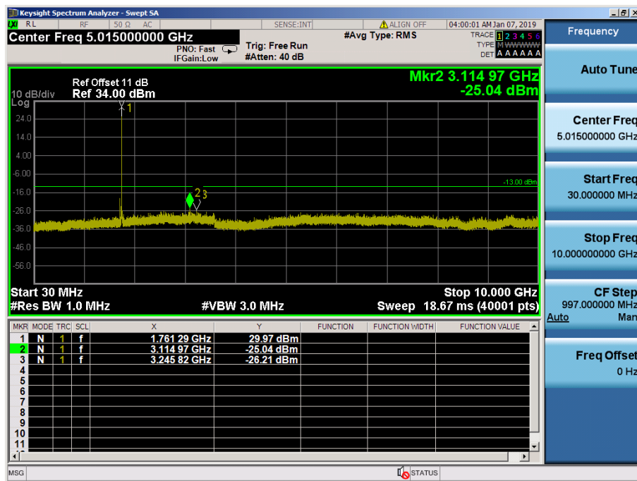
LTE Band 66, 4 / 20MHz / 64QAM - RB Size/Offset (1/0) – High Channel
