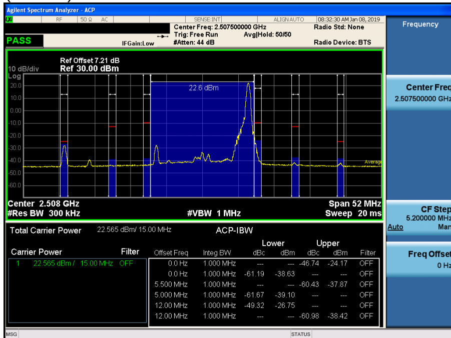
LTE Band 7 / 15MHz / QPSK - RB Size/Offset (1/75)
