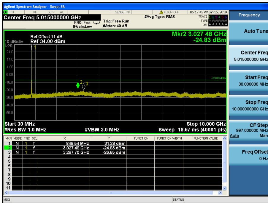
LTE Band 5 / 10MHz / 64QAM - RB Size/Offset (1/49) – High Channel
