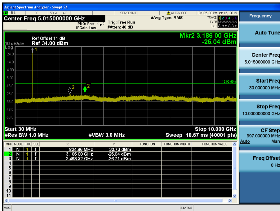
LTE Band 5 / 1.4MHz / 64QAM - RB Size/Offset (1/0) – Low Channel
