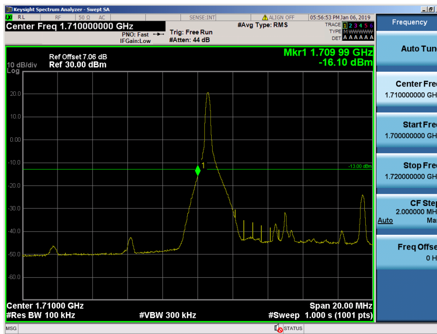
LTE Band 66, 4 / 10MHz / QPSK - RB Size/Offset (1/0)
