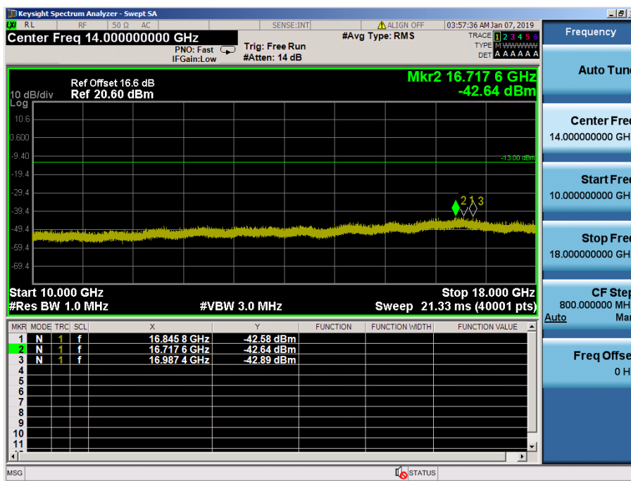
LTE Band 66, 4 / 20MHz / 64QAM - RB Size/Offset (100/0)–Mid Channel
