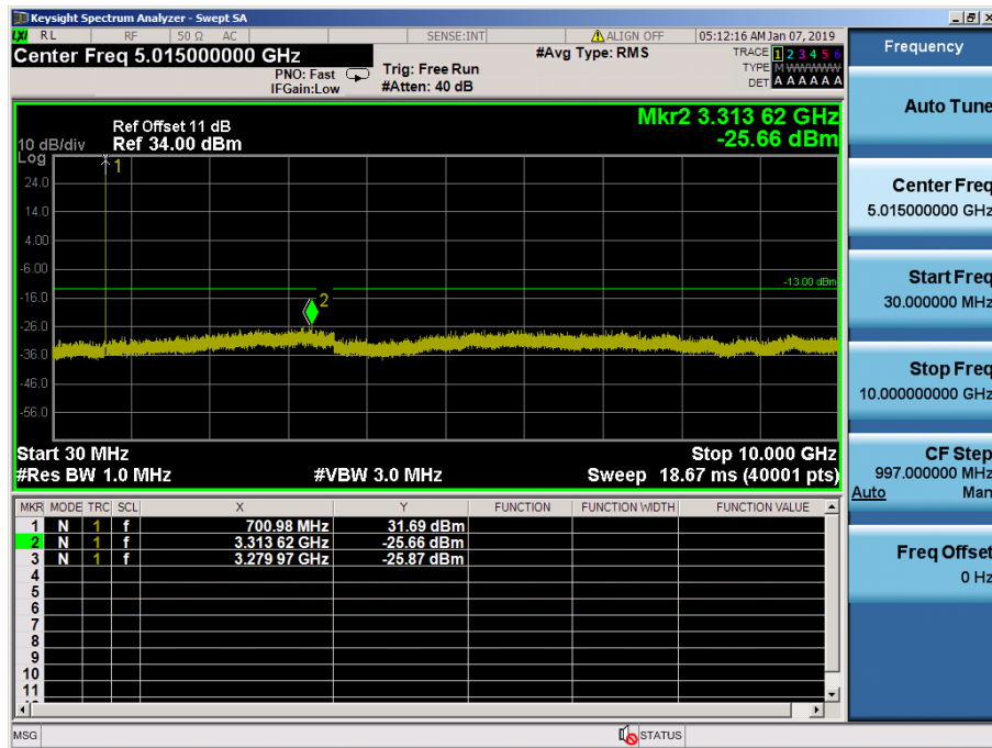
LTE Band 12 / 3MHz / QPSK - RB Size/Offset (1/7) – Low Channel
