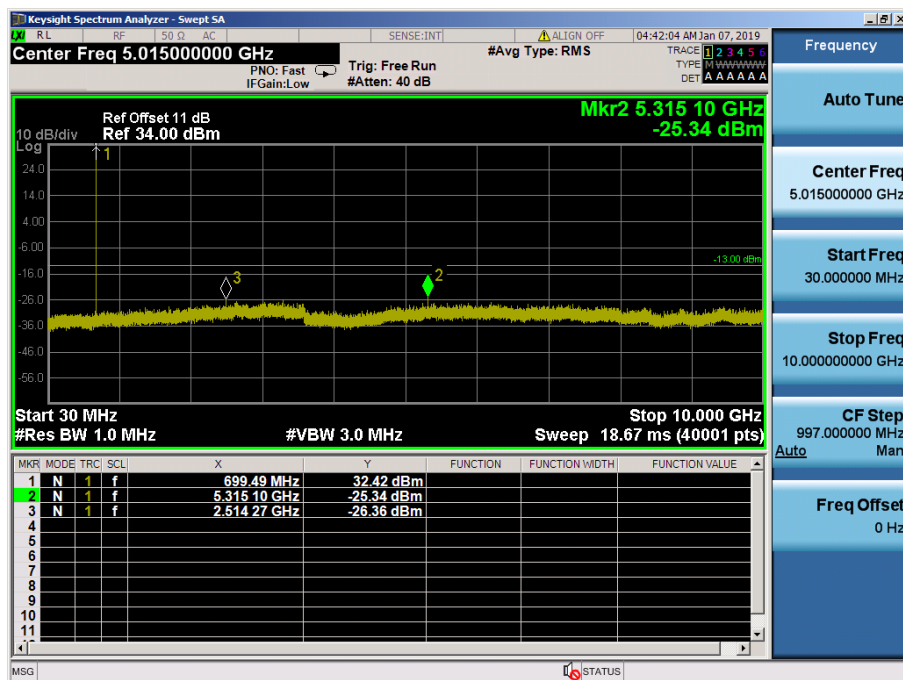
LTE Band 12 / 1.4MHz / QPSK - RB Size/Offset (3/0) – Low Channel
