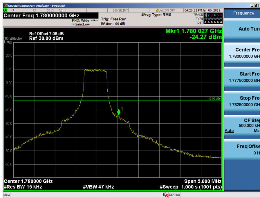
LTE Band 66, 4 / 1.4MHz / QPSK - RB Size/Offset (3/3)
