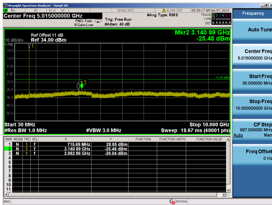
LTE Band 12 / 3MHz / QPSK - RB Size/Offset (8/7) – High Channel
