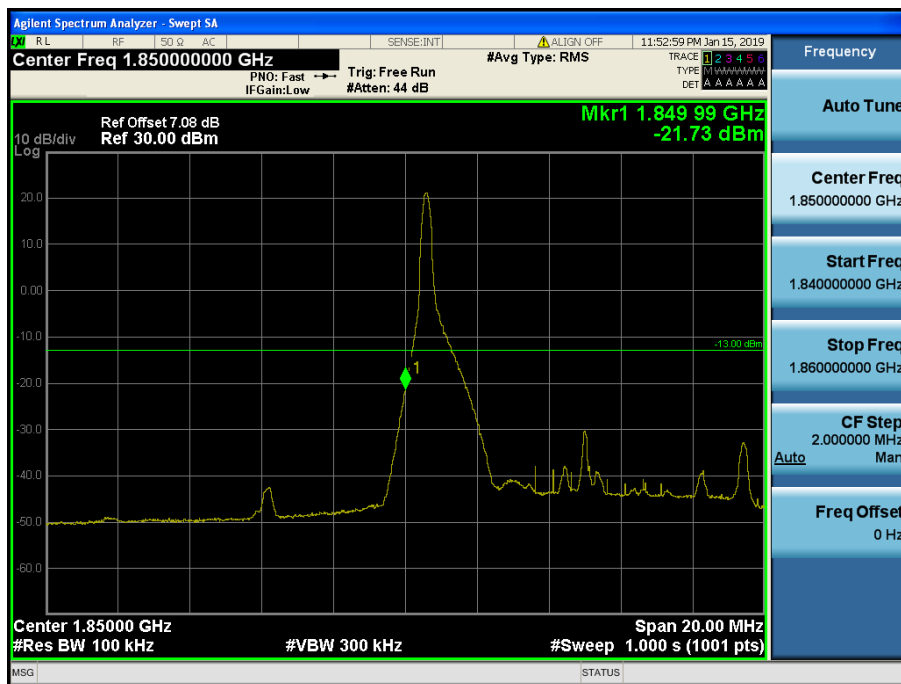
LTE Band 2 / 10MHz / QPSK - RB Size/Offset (1/0)
