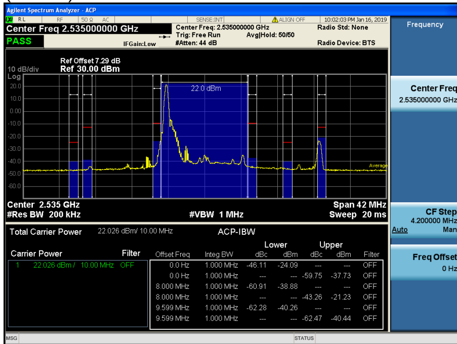
LTE Band 7 / 10MHz / 16QAM - RB Size/Offset (1/0)
