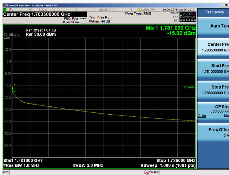
LTE Band 66, 4 / 5MHz / 16QAM - RB Size/Offset (12/13)
