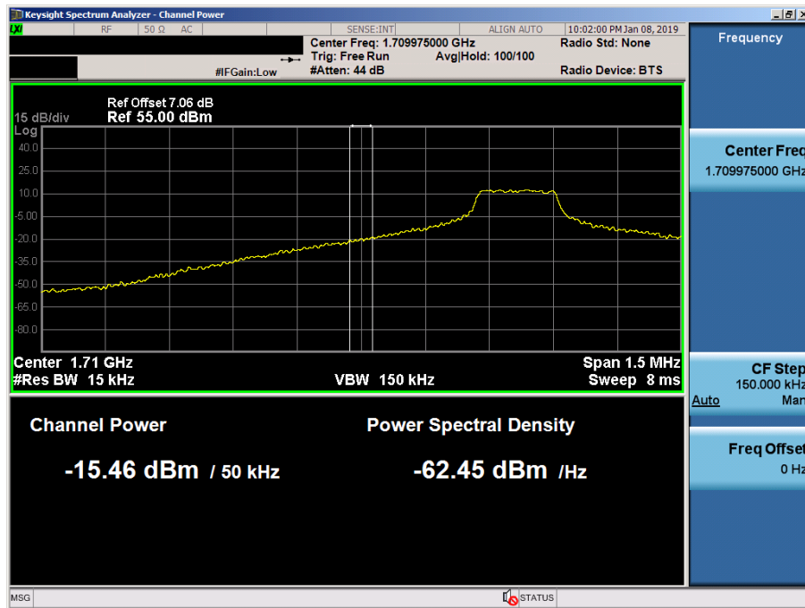
LTE Band 66, 4 / 5MHz / 16QAM Offset/Size (1/0)
