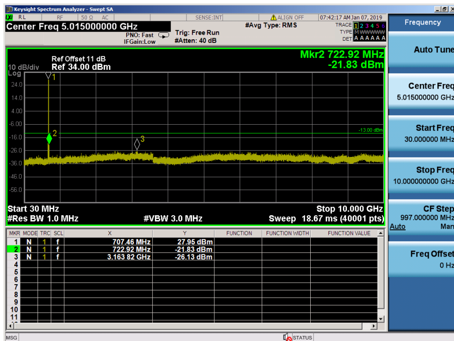
LTE Band 12 / 3MHz / 16QAM - RB Size/Offset (15/0) – Mid Channel
