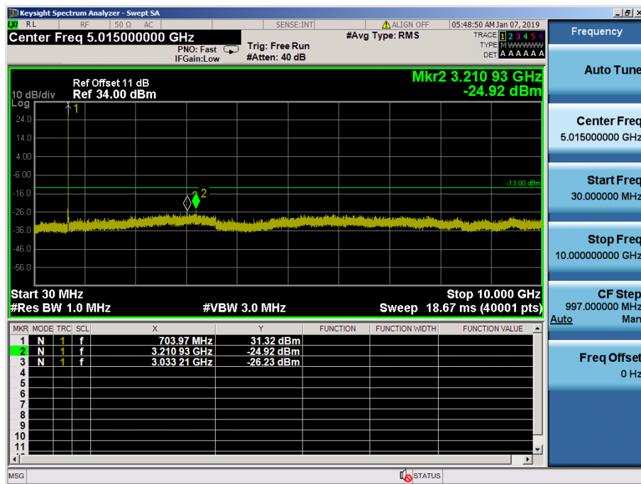
LTE Band 12, 17 / 5MHz / QPSK - RB Size/Offset (1/24) – Low Channel
