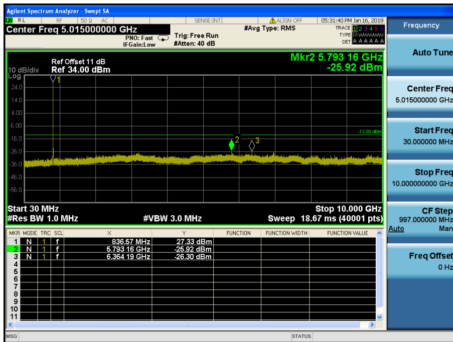
LTE Band 5 / 5MHz / 64QAM - RB Size/Offset (12/13) – Mid Channel
