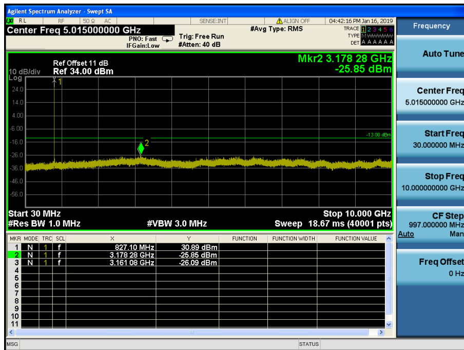
LTE Band 5 / 3MHz / 64QAM - RB Size/Offset (1/14) – Low Channel
