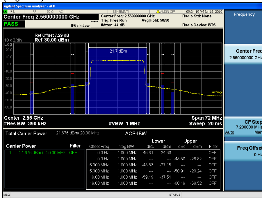
LTE Band 7 / 20MHz / QPSK - RB Size/Offset (50/0)
