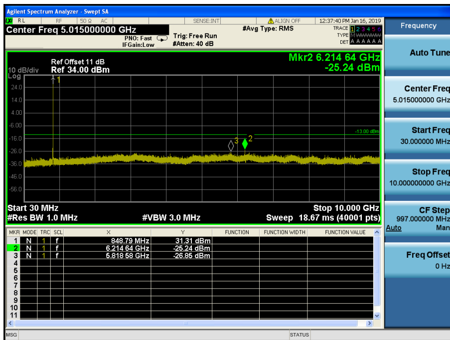
LTE Band 5 / 5MHz / QPSK - RB Size/Offset (1/24) – High Channel
