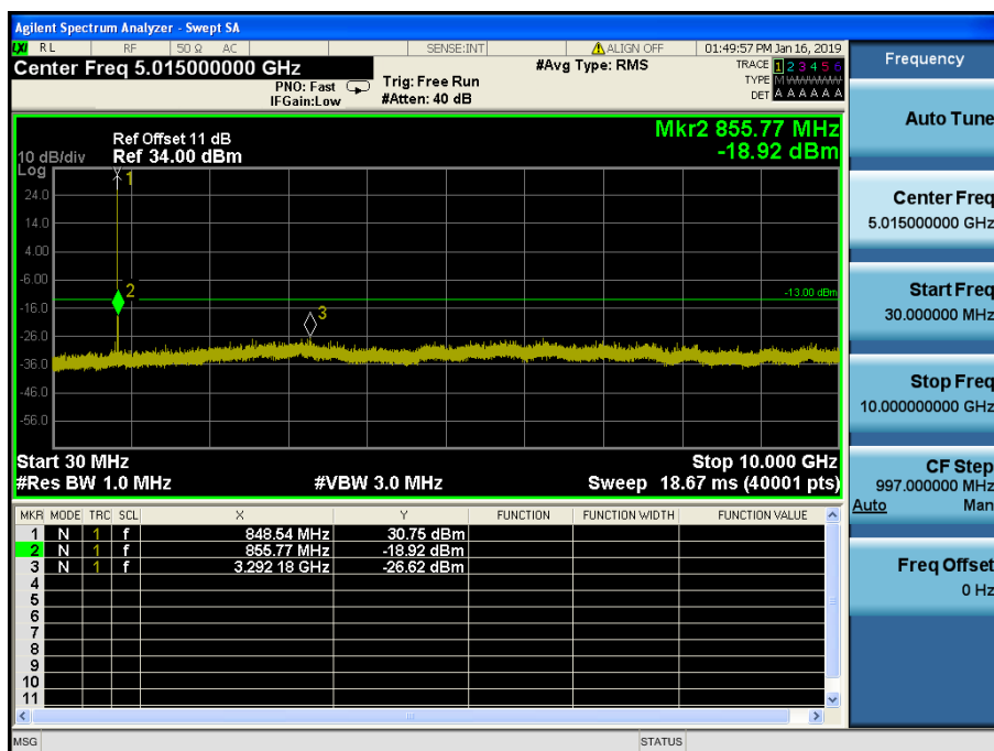
LTE Band 5 / 1.4MHz / 16QAM - RB Size/Offset (1/2) – High Channel
