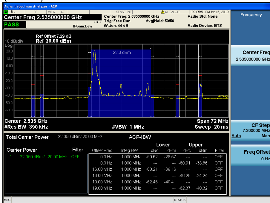
LTE Band 7 / 20MHz / QPSK - RB Size/Offset (1/0)
