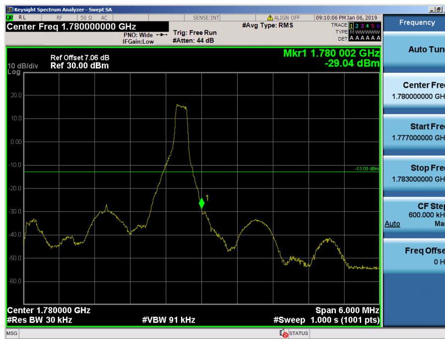
LTE Band 66, 4 / 3MHz / 16QAM - RB Size/Offset (1/14)
