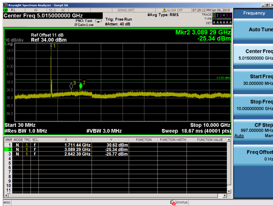
LTE Band 66, 4 / 20MHz / QPSK - RB Size/Offset (1/0) –Low Channel
