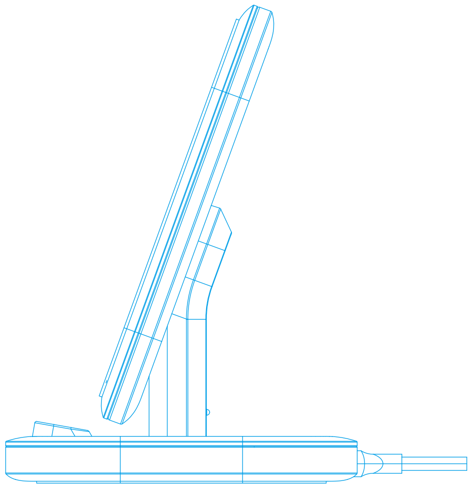
right view
