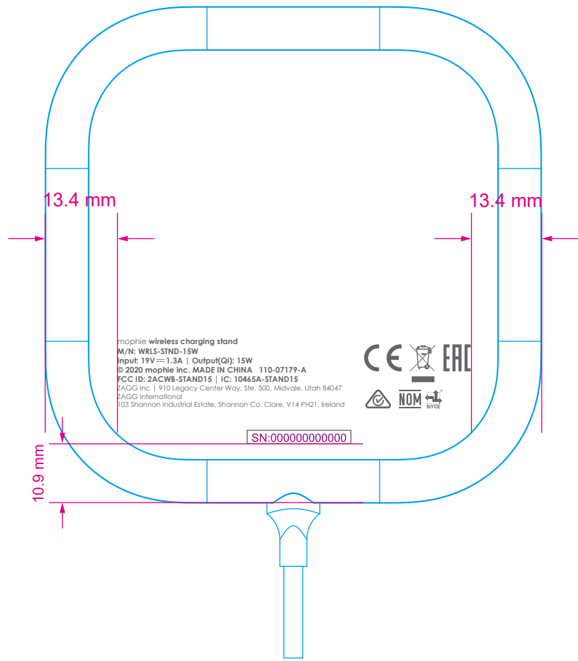
bottom view
