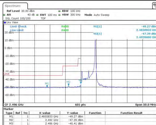
Band41-5MHz-QPSK-39675-25RB#0
