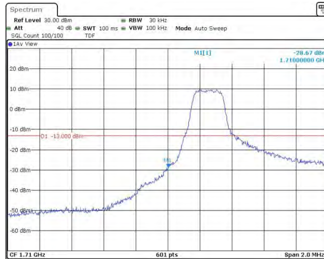
Band66-1.4MHz-QPSK-131979-1RB#5
