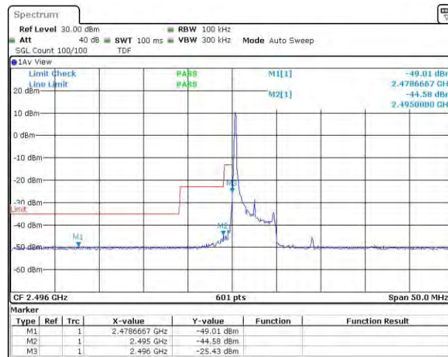
Band41-5MHz-QPSK-39675-1RB#24
