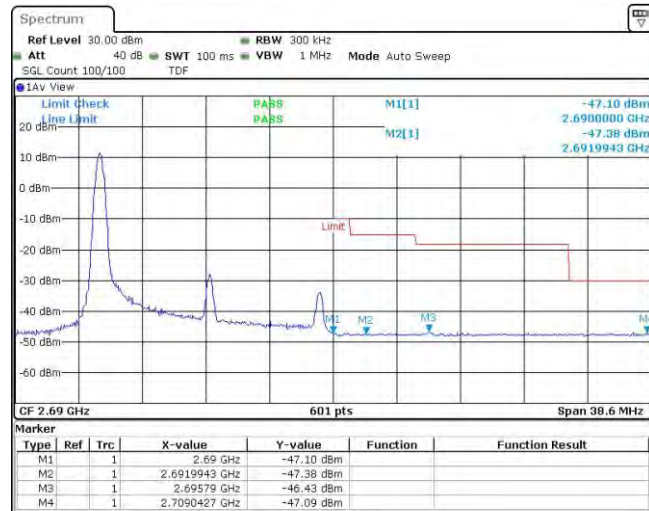
Band41-15MHz-16QAM-41515-1RB#74
