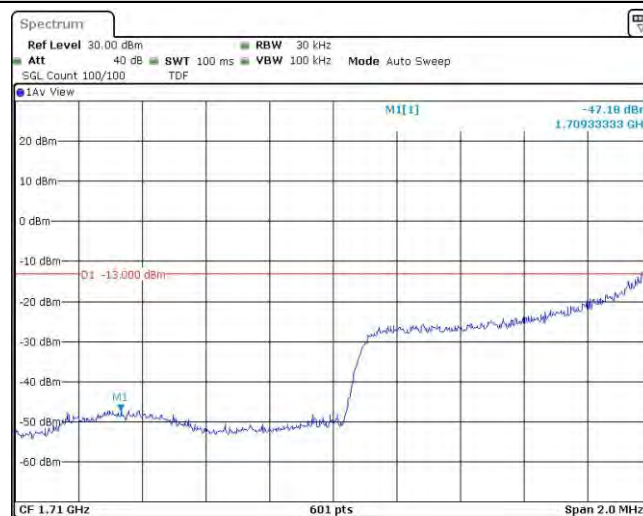
Band66-1.4MHz-QPSK-131979-6RB#0
