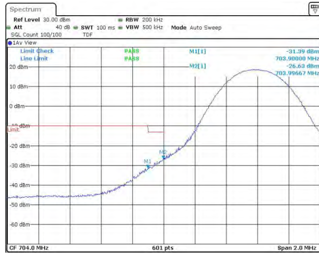
Band17-10MHz-QPSK-23780-1RB#49
