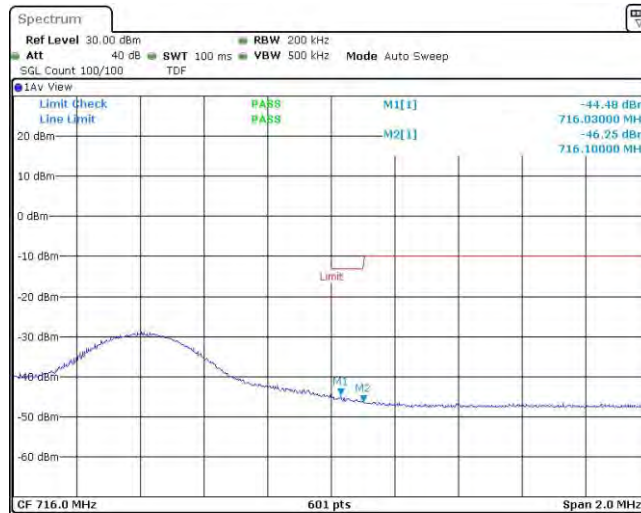
Band17-10MHz-16QAM-23800-1RB#49
