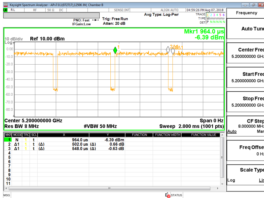
DUTY CYCLE 802.11n HT20 2TX MODE
