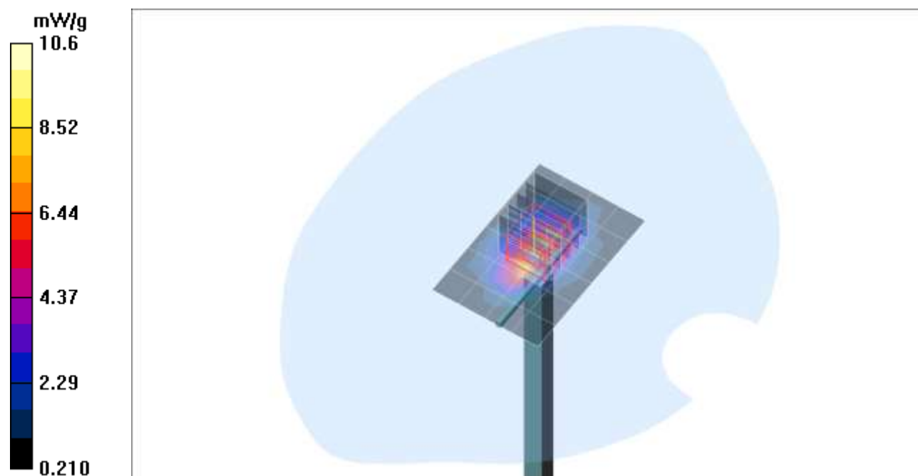
Plot. 2: System Verification Measurement 1900 MHz, body (April 01, 2019).
