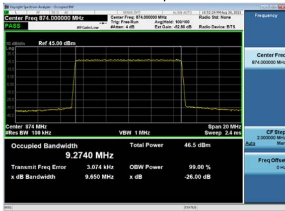
Channel Frequency 874MHz, 1C, 64QAM 10MHz BW, TX3
