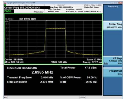
Channel Frequency 885MHz, 1C, 64QAM 3MHz BW, TX1
