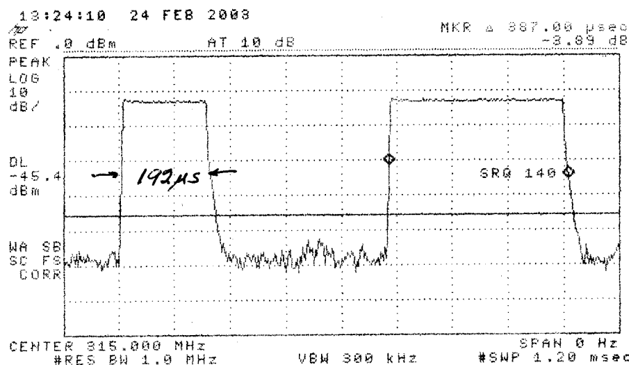
Figure 6.1(cont.). Transmissions modulation characteristics: (top) superhete pre-amble, (center) regen pre-amble, (bottom) expanded bits.
