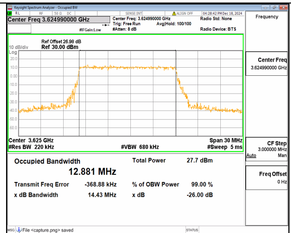
n48 15M DFT-s-OFDM 64QAM Outer_Full Mid
