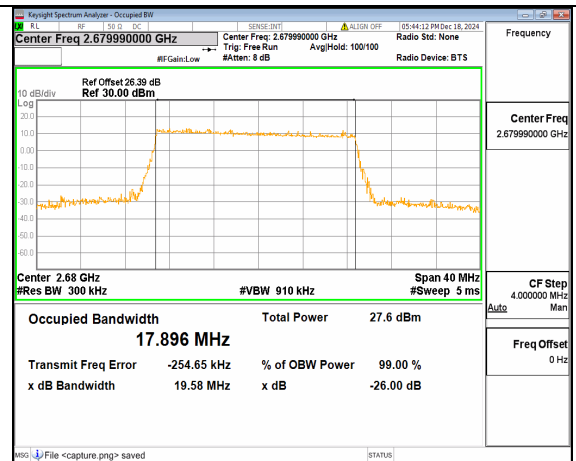
n41 20M DFT-s-OFDM 64QAM Outer_Full High
