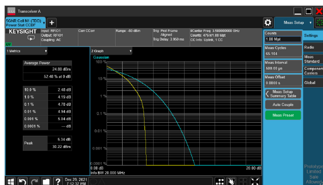
5G NR n77 CH633334 20M 1RB 16-QAM Ratio
