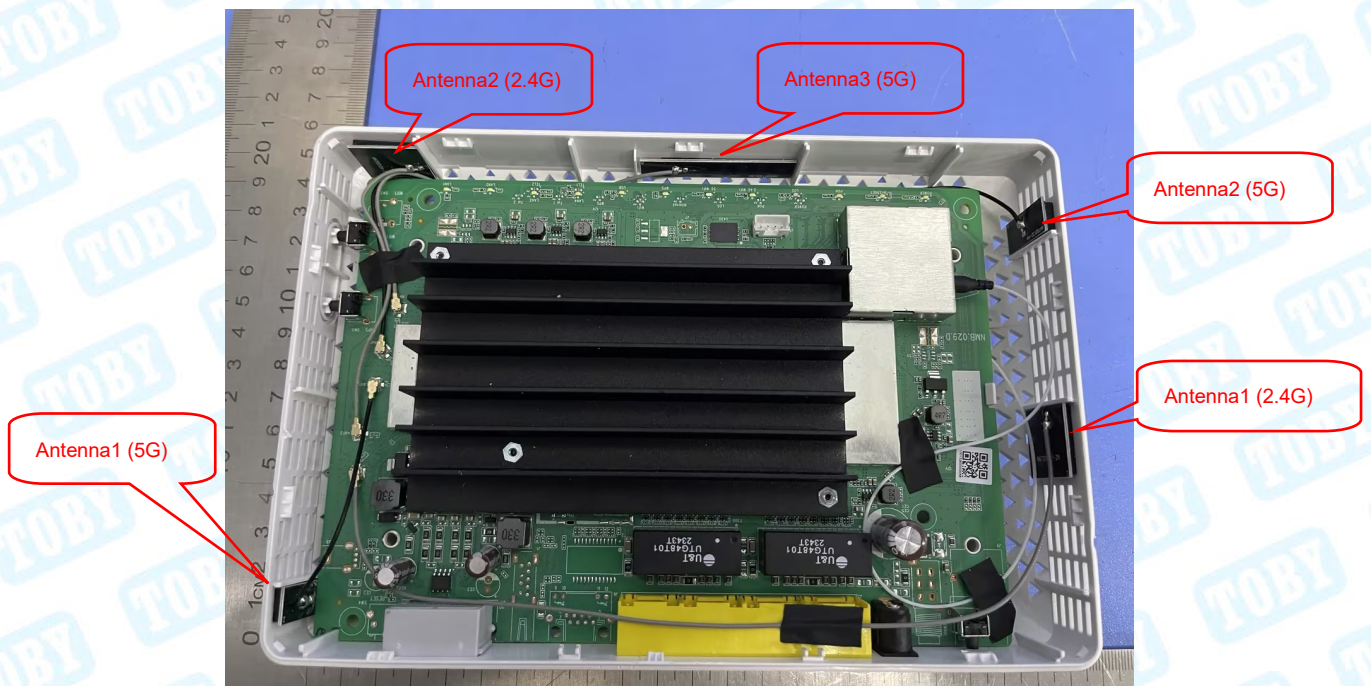
Photo 9 Internal of EUT
