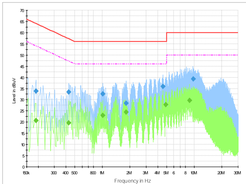
Fig.B.8.1 AC Powerline Conducted Emission- BLE
