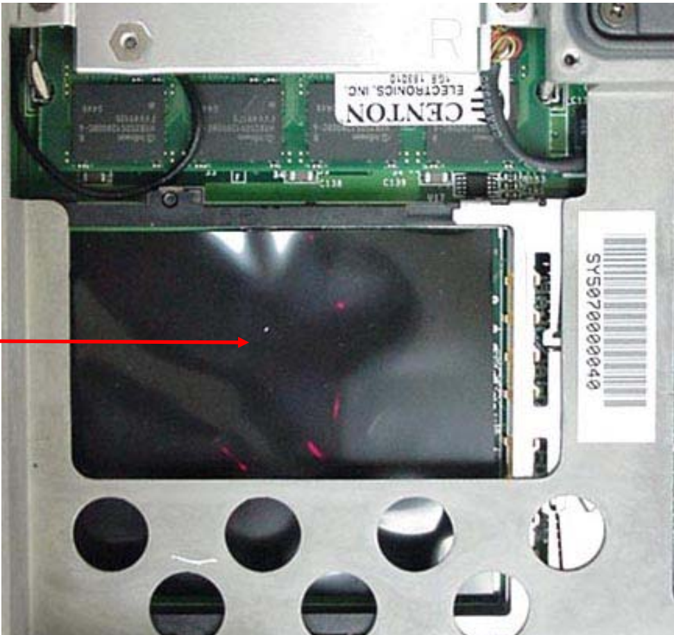
AirCard 580 Removed
