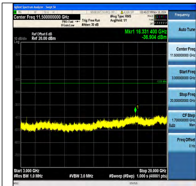
Band2_10MHz_QPSK_18650_1RB#0_3000~20000_3000~20000
