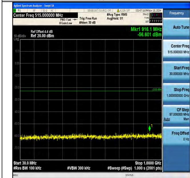
Band2_10MHz_16QAM_18900_1RB#0_30~1000_30~1000
