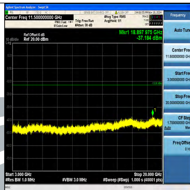
Band2_20MHz_16QAM_18700_1RB#0_3000~20000_3000~20000
