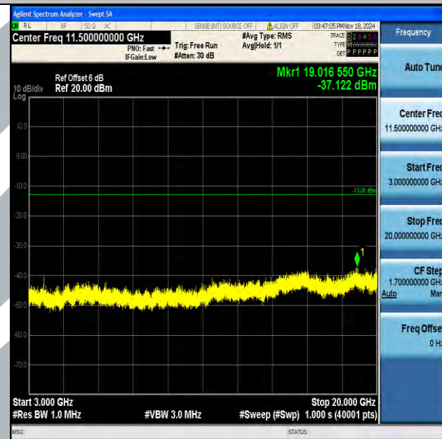
Band2_10MHz_QPSK_18900_1RB#0_3000~20000_3000~20000
