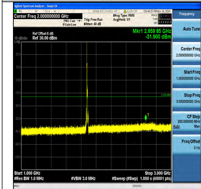
Band2_10MHz_QPSK_18900_1RB#0_1000~3000_1000~3000
