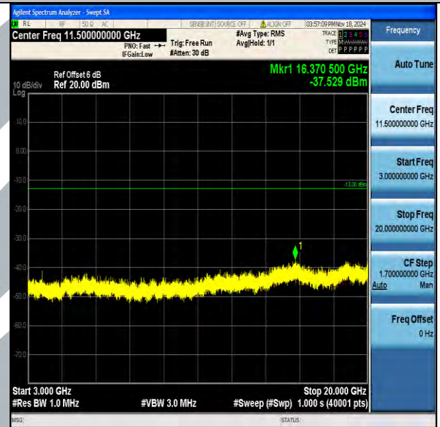
Band2_15MHz_16QAM_18675_1RB#0_3000~20000_3000~20000
