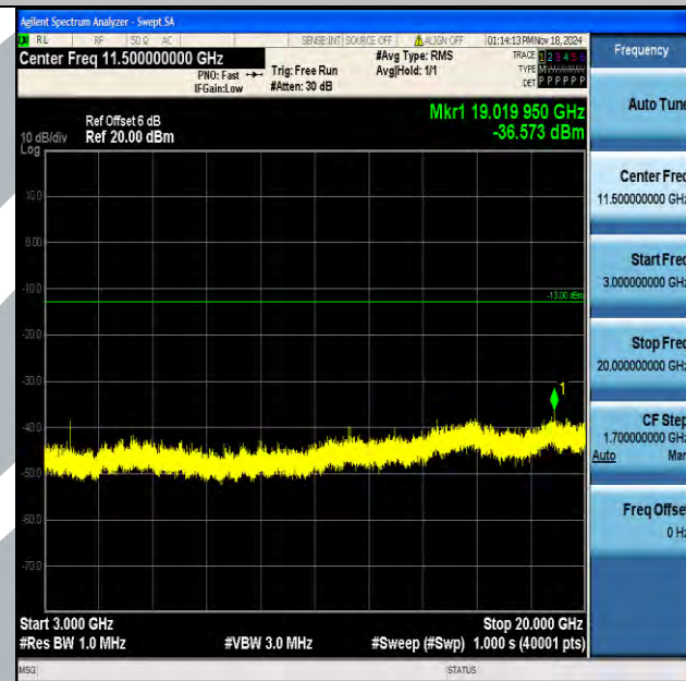
Band2_3MHz_16QAM_19185_1RB#0_3000~20000_3000~20000
