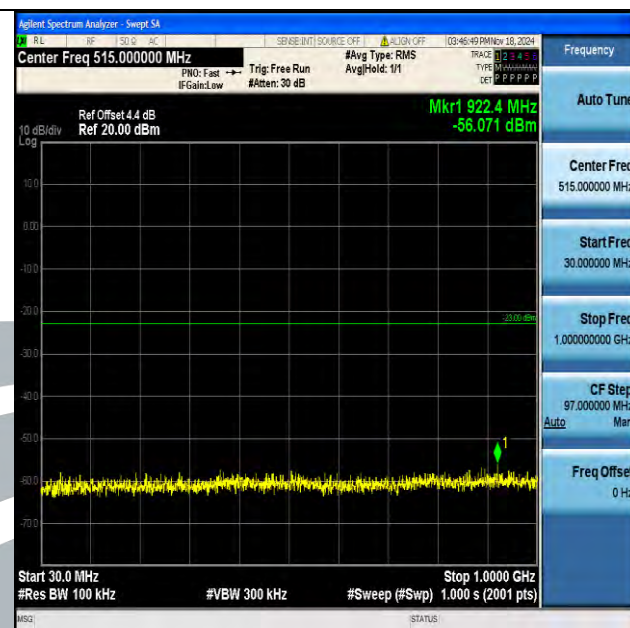
Band2_10MHz_QPSK_18900_1RB#0_30~1000_30~1000
