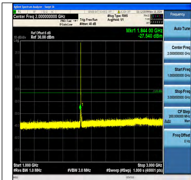
Band2_3MHz_16QAM_18615_1RB#0_1000~3000_1000~3000
