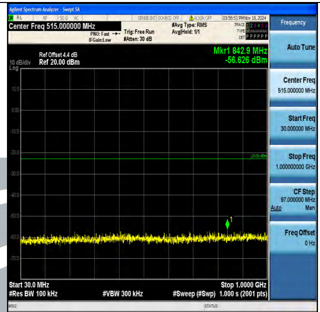
Band2_15MHz_16QAM_18675_1RB#0_30~1000_30~1000
