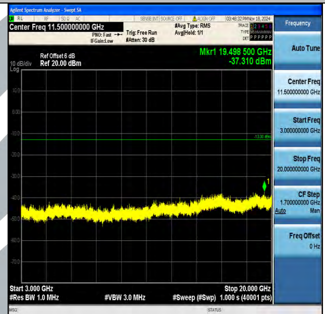
Band2_10MHz_16QAM_19150_1RB#0_3000~20000_3000~20000
