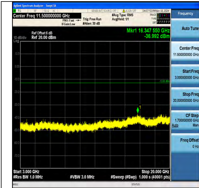
Band2_20MHz_16QAM_18900_1RB#0_3000~20000_3000~20000
