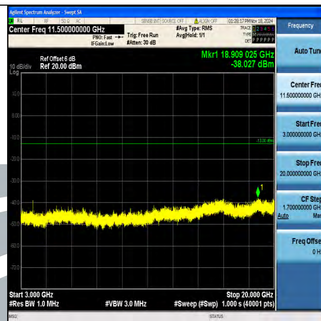
Band2_5MHz_16QAM_19175_1RB#0_3000~20000_3000~20000
