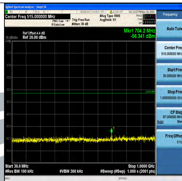
Band2_3MHz_16QAM_19185_1RB#0_30~1000_30~1000
