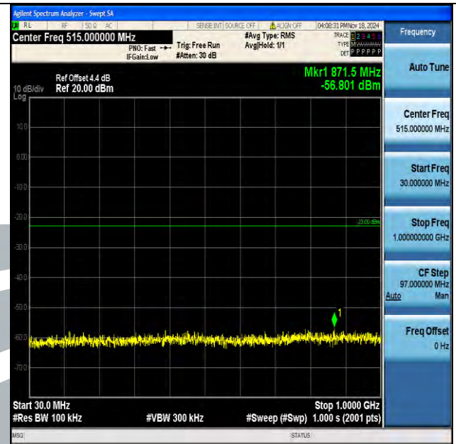
Band2_20MHz_16QAM_19100_1RB#0_30~1000_30~1000
