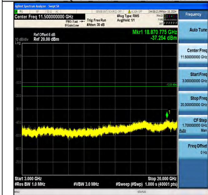
Band2_20MHz_QPSK_19100_1RB#0_3000~20000_3000~20000
