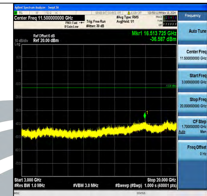
Band2_15MHz_16QAM_19125_1RB#0_3000~20000_3000~20000
