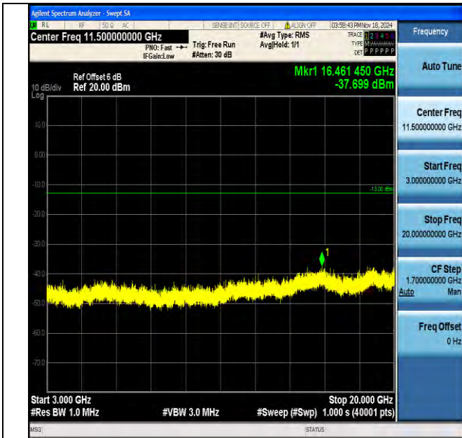
Band2_15MHz_QPSK_19125_1RB#0_3000~20000_3000~20000
