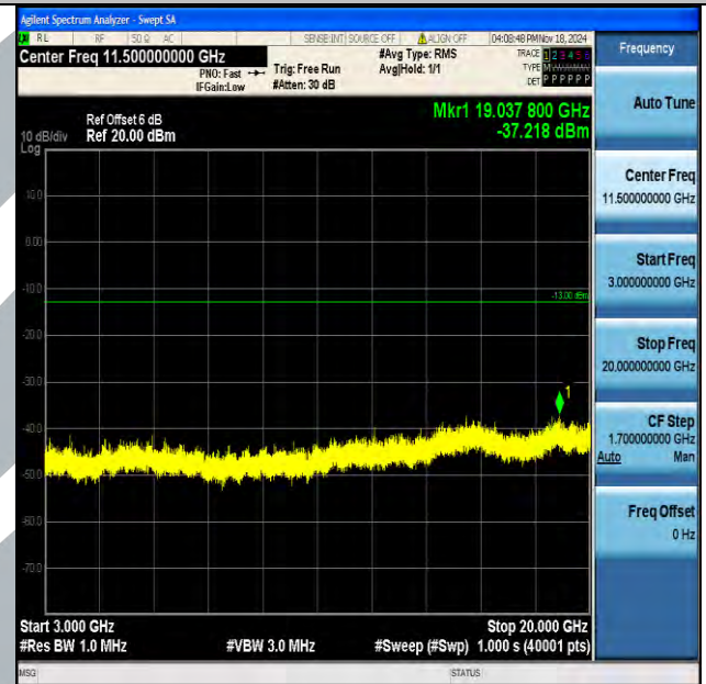
Band2_20MHz_16QAM_19100_1RB#0_3000~20000_3000~20000
