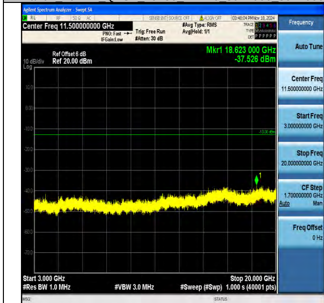
Band2_10MHz_QPSK_19150_1RB#0_3000~20000_3000~20000
