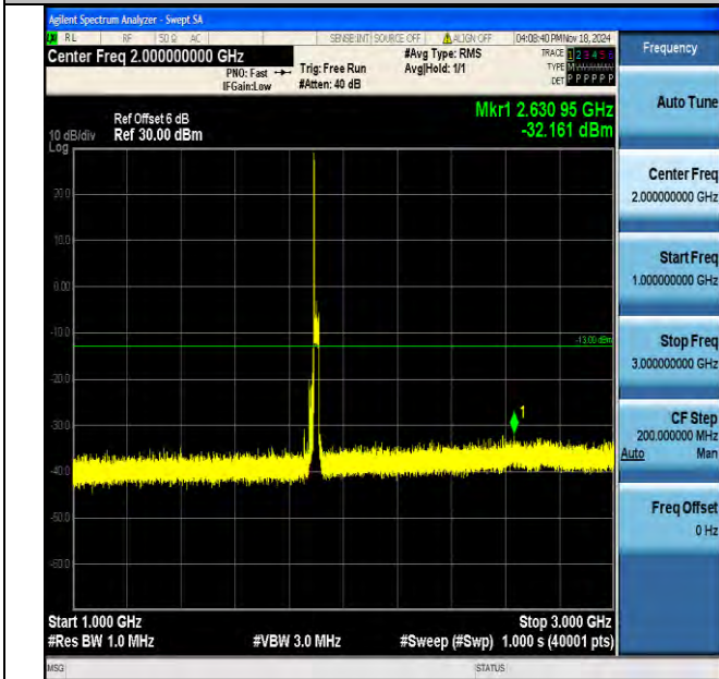
Band2_20MHz_16QAM_19100_1RB#0_1000~3000_1000~3000
