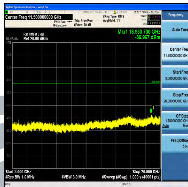
Band2_3MHz_16QAM_18615_1RB#0_3000~20000_3000~20000
