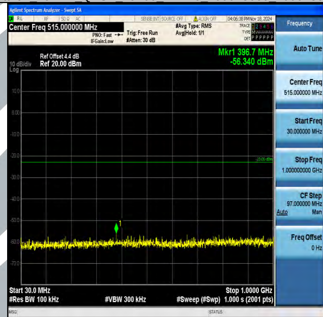
Band2_20MHz_16QAM_18700_1RB#0_30~1000_30~1000
