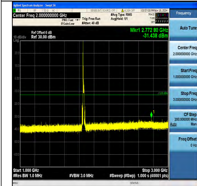
Band2_15MHz_16QAM_18675_1RB#0_1000~3000_1000~3000
