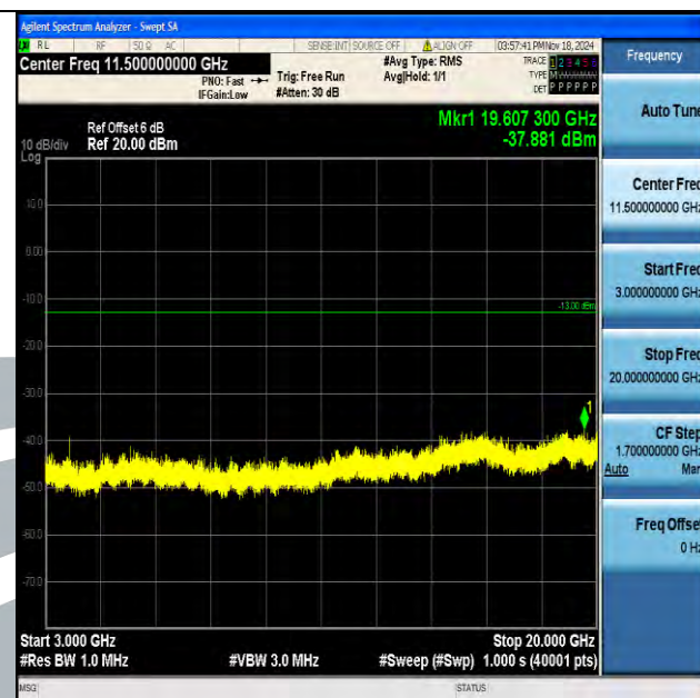
Band2_15MHz_QPSK_18900_1RB#0_3000~20000_3000~20000
