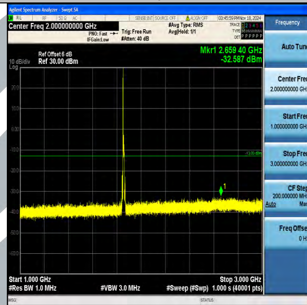
Band2_10MHz_QPSK_18650_1RB#0_1000~3000_1000~3000
