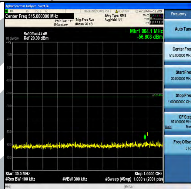
Band2_10MHz_16QAM_18650_1RB#0_30~1000_30~1000
