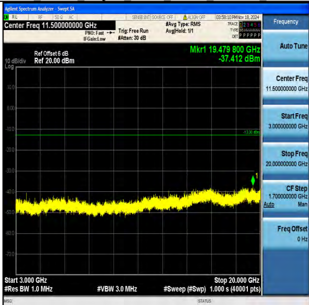
Band2_15MHz_16QAM_18900_1RB#0_3000~20000_3000~20000
