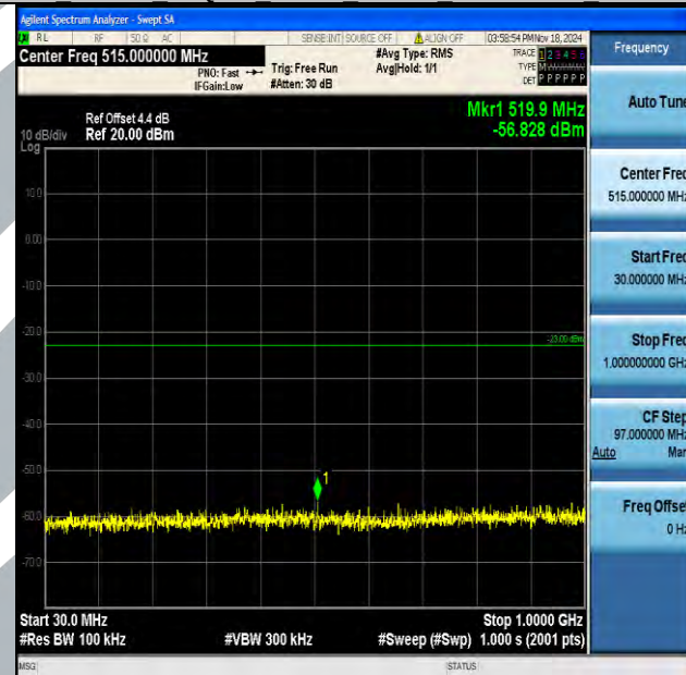
Band2_15MHz_16QAM_19125_1RB#0_30~1000_30~1000
