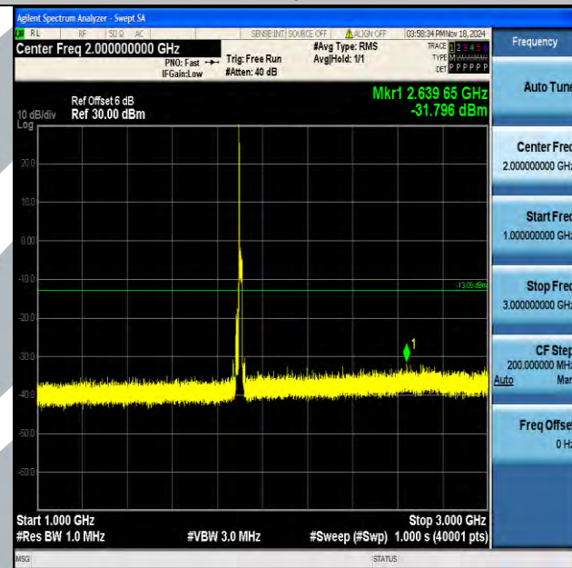
Band2_15MHz_QPSK_19125_1RB#0_1000~3000_1000~3000
