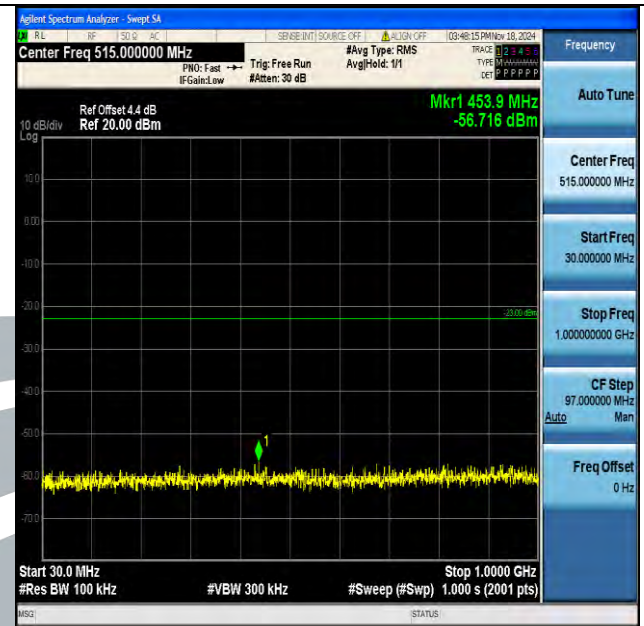
Band2_10MHz_16QAM_19150_1RB#0_30~1000_30~1000
