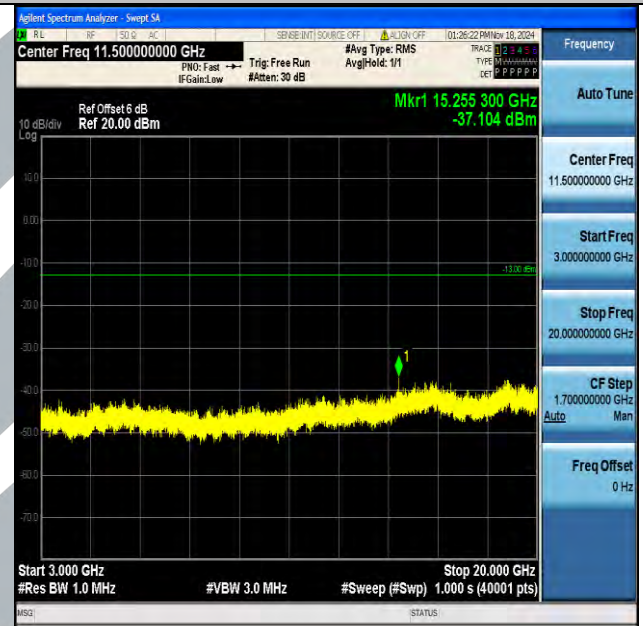
Band2_5MHz_16QAM_18625_1RB#0_3000~20000_3000~20000
