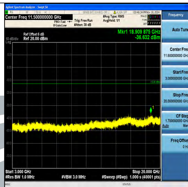
Band2_10MHz_16QAM_18650_1RB#0_3000~20000_3000~20000
