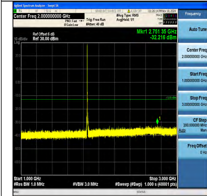
Band2_5MHz_16QAM_18625_1RB#0_1000~3000_1000~3000
