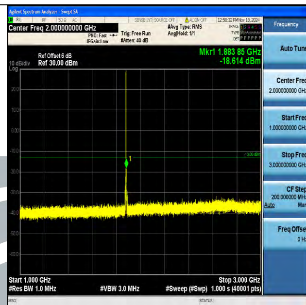
Band2_1.4MHz_16QAM_18900_1RB#0_1000~3000_1000~3000
