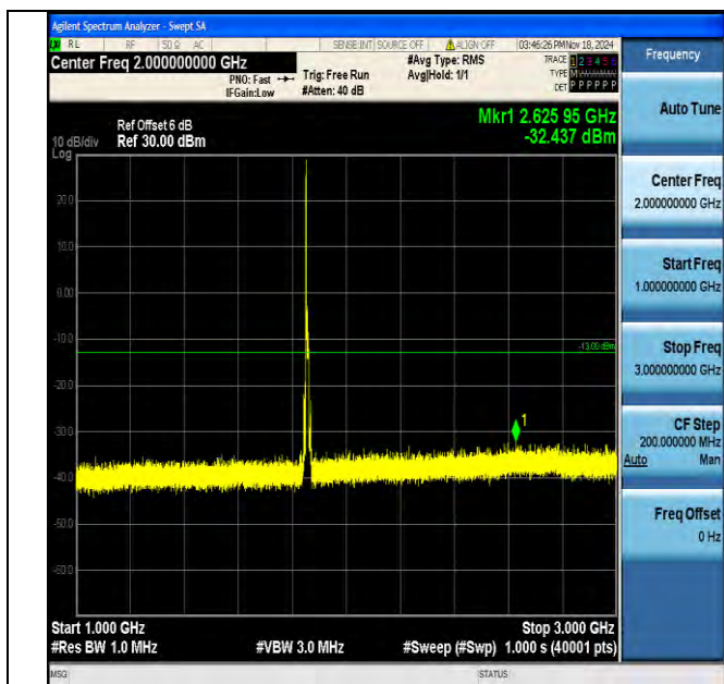
Band2_10MHz_16QAM_18650_1RB#0_1000~3000_1000~3000
