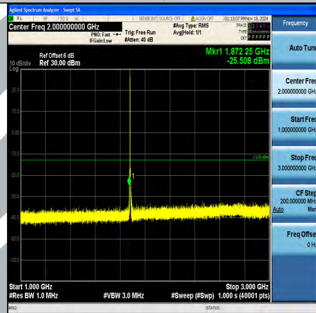
Band2_3MHz_16QAM_18900_1RB#0_1000~3000_1000~3000
