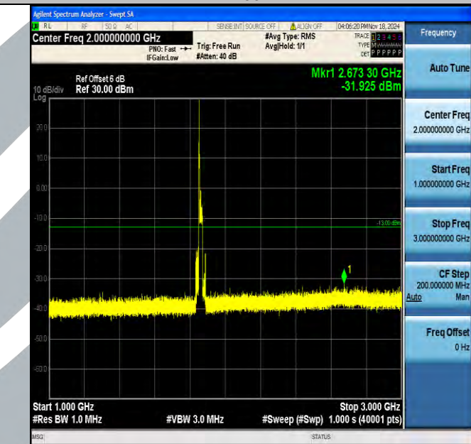
Band2_20MHz_QPSK_18700_1RB#0_1000~3000_1000~3000
