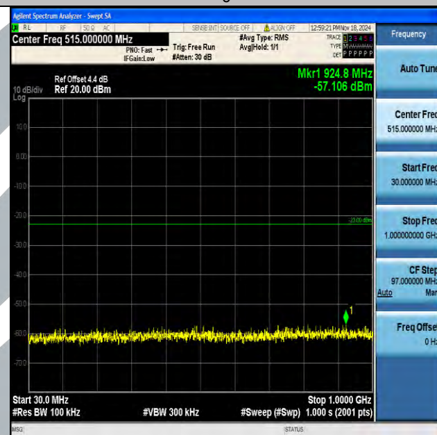
Band2_1.4MHz_16QAM_19193_1RB#0_30~1000_30~1000
