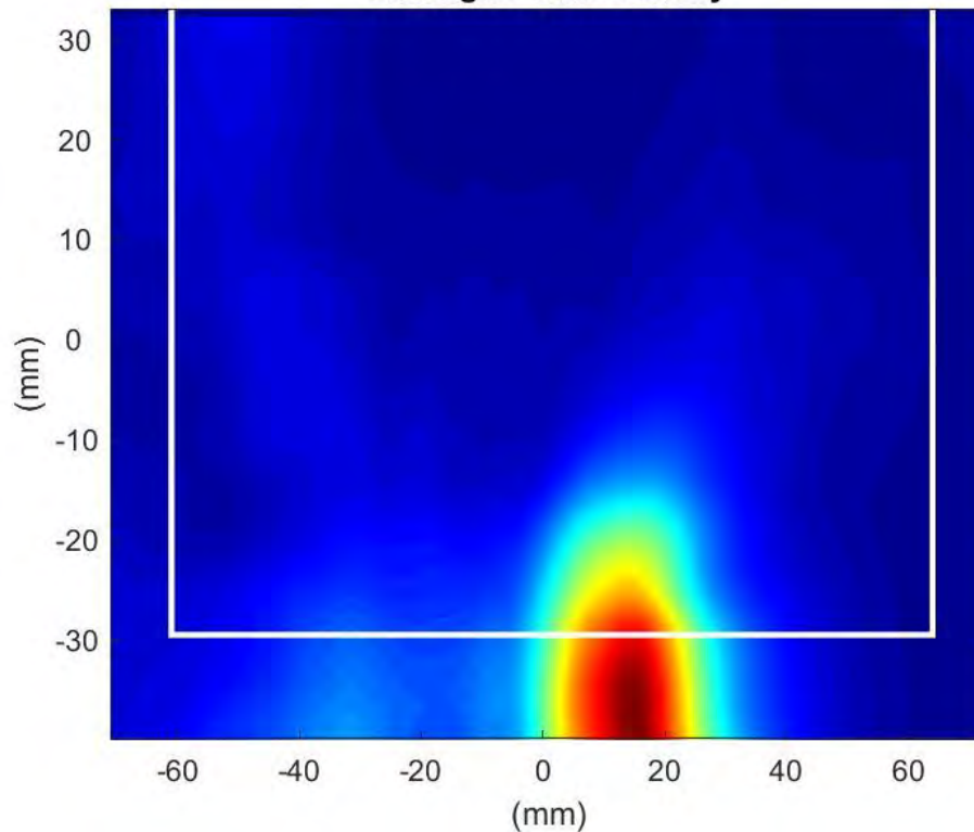
Phaser2 Beam:177 Surface:S1 Average Power Density
