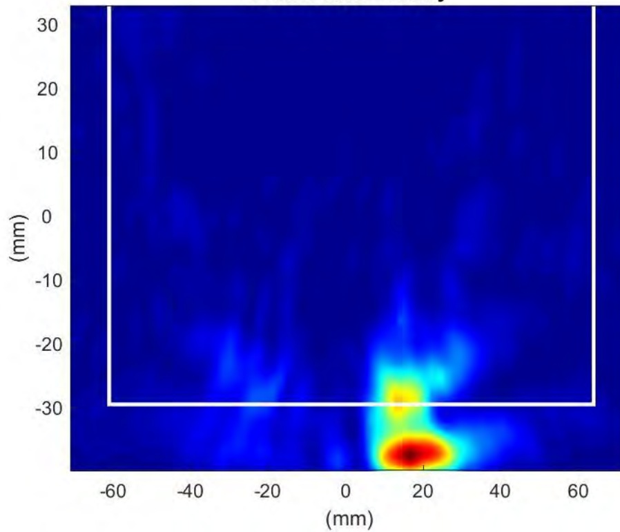
Phaser2 Beam Pair:46-177 Surface:S1 Average Power Density
