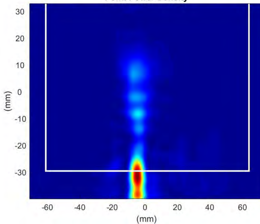
Phaser2 Beam Pair:22-149 Surface:S1 Average Power Density
