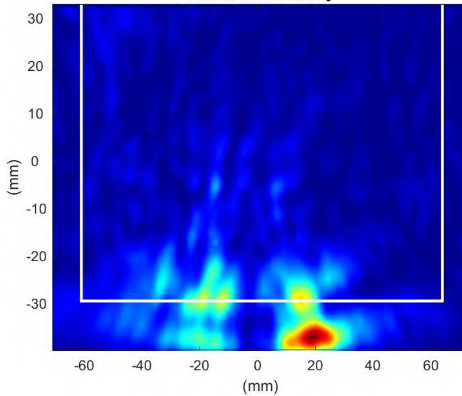
Phaser2 Beam Pair:20-148 Surface:S1 Average Power Density
