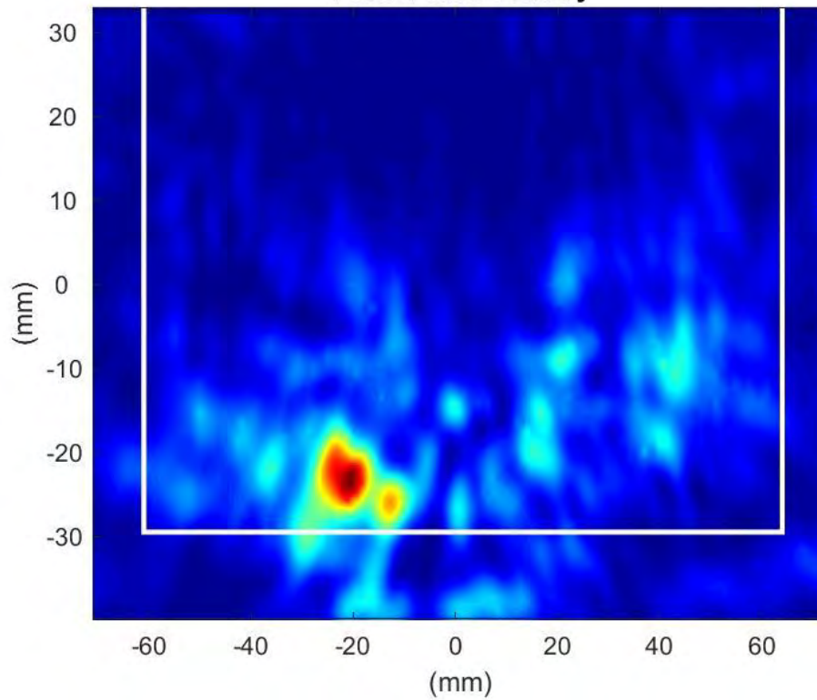
Phaser2 Beam Pair:22-149 Surface:S2 Average Power Density
