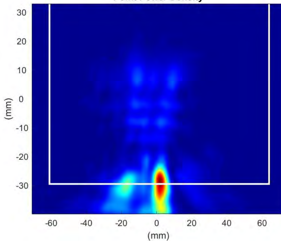
Phaser2 Beam Pair:21-150 Surface:S1 Average Power Density
