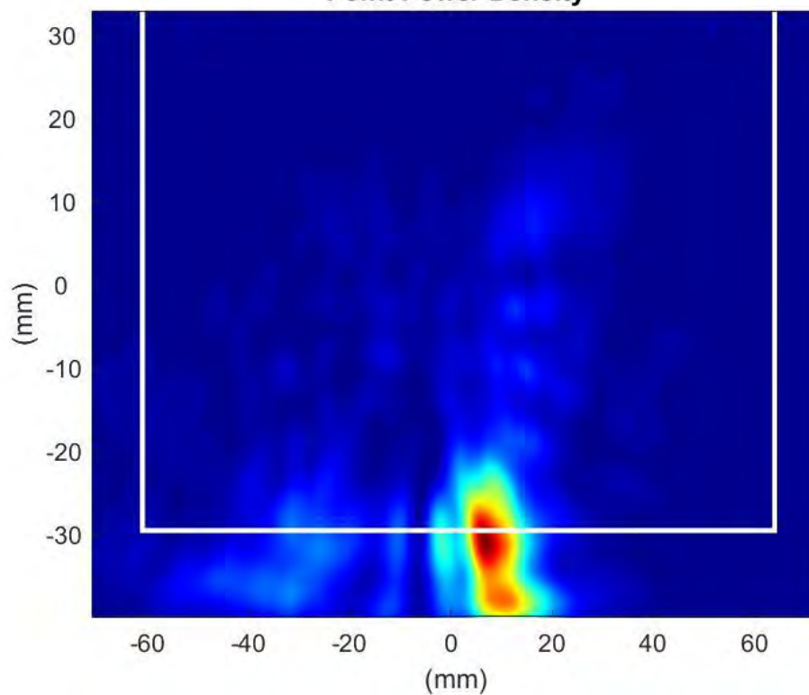
Phaser2 Beam Pair:23-151 Surface:S1 Average Power Density
