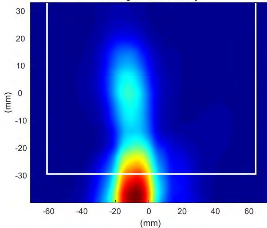
Phaser2 Beam Pair:34-162 Surface:S1 Average Power Density
