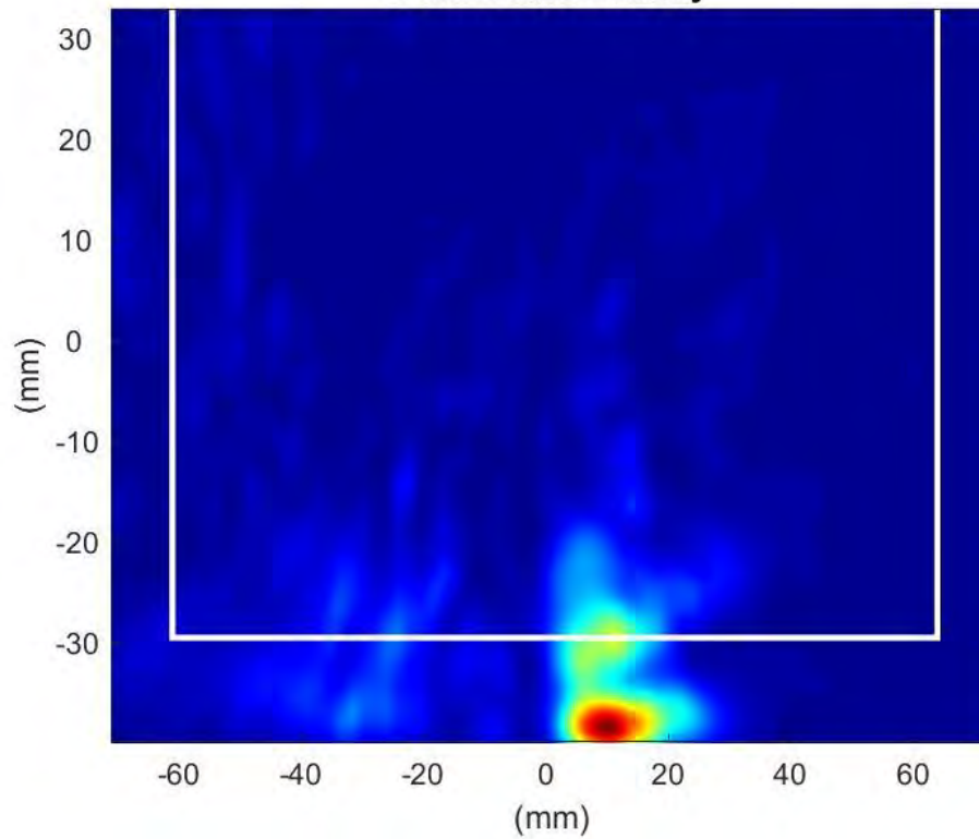
Phaser2 Beam Pair:59-189 Surface:S1 Average Power Density
