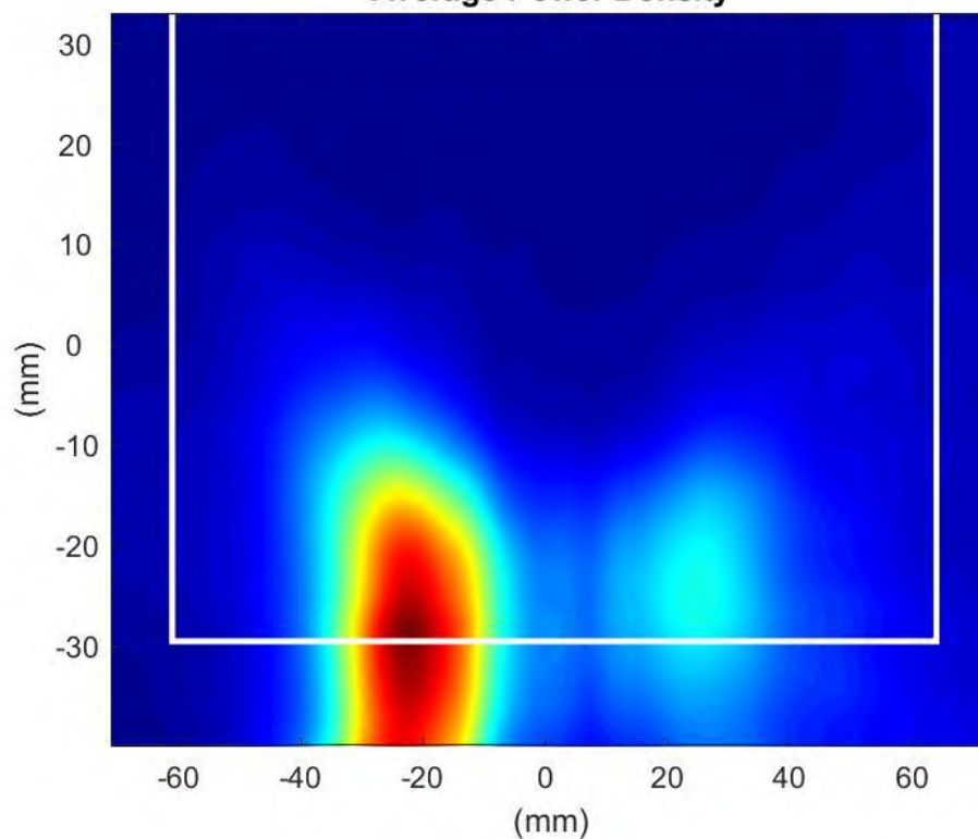
Phaser2 Beam:178 Surface:S2 Average Power Density
