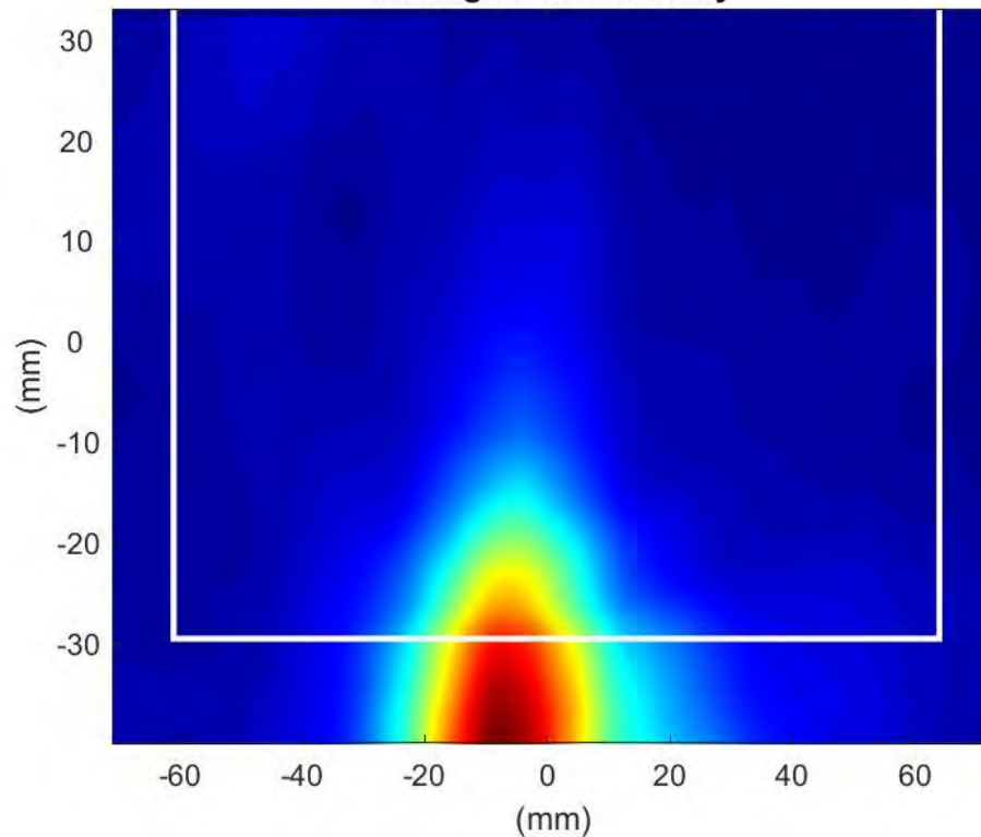
Phaser2 Beam Pair:4-132 Surface:S1 Average Power Density
