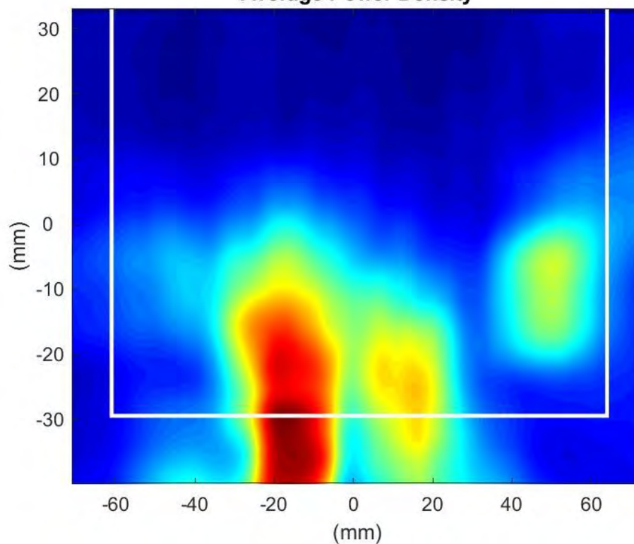
Phaser2 Beam Pair:21-150 Surface:S2 Average Power Density
