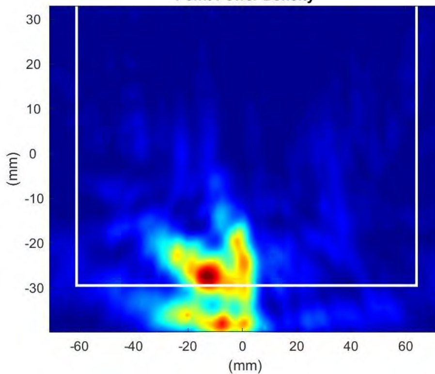
Phaser2 Beam Pair:33-160 Surface:S2 Average Power Density
