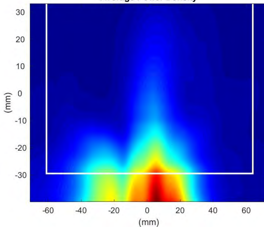
Phaser2 Beam Pair:62-188 Surface:S1 Average Power Density
