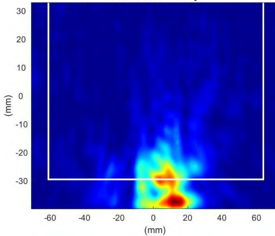
Phaser2 Beam Pair:32-161 Surface:S1 Average Power Density
