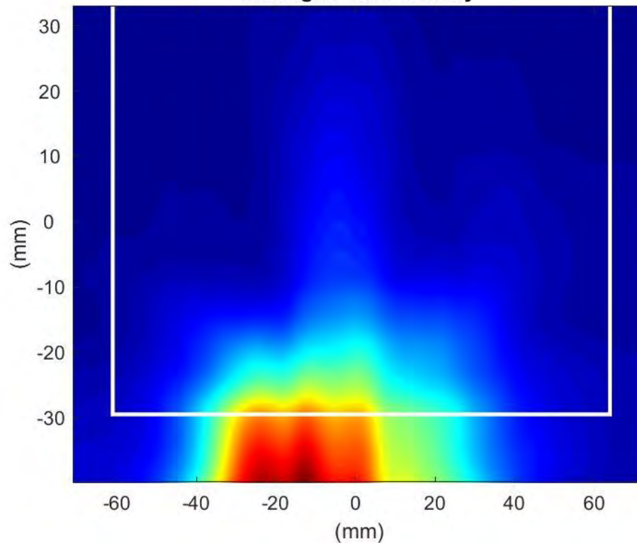
Phaser2 Beam Pair:49-175 Surface:S1 Average Power Density
