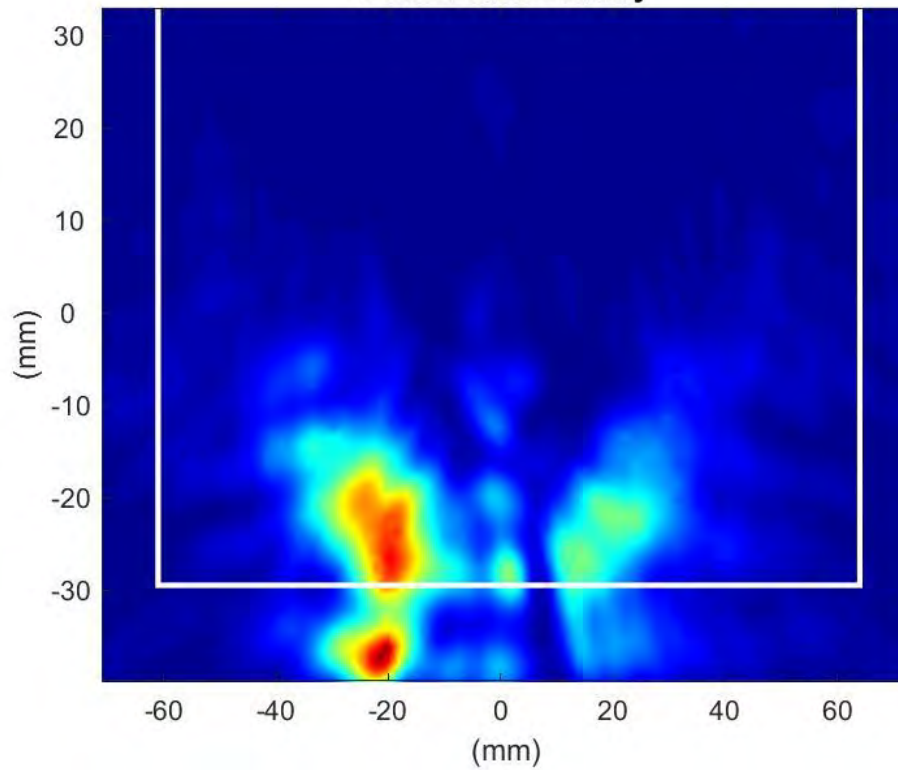
Phaser2 Beam Pair:60-190 Surface:S2 Average Power Density
