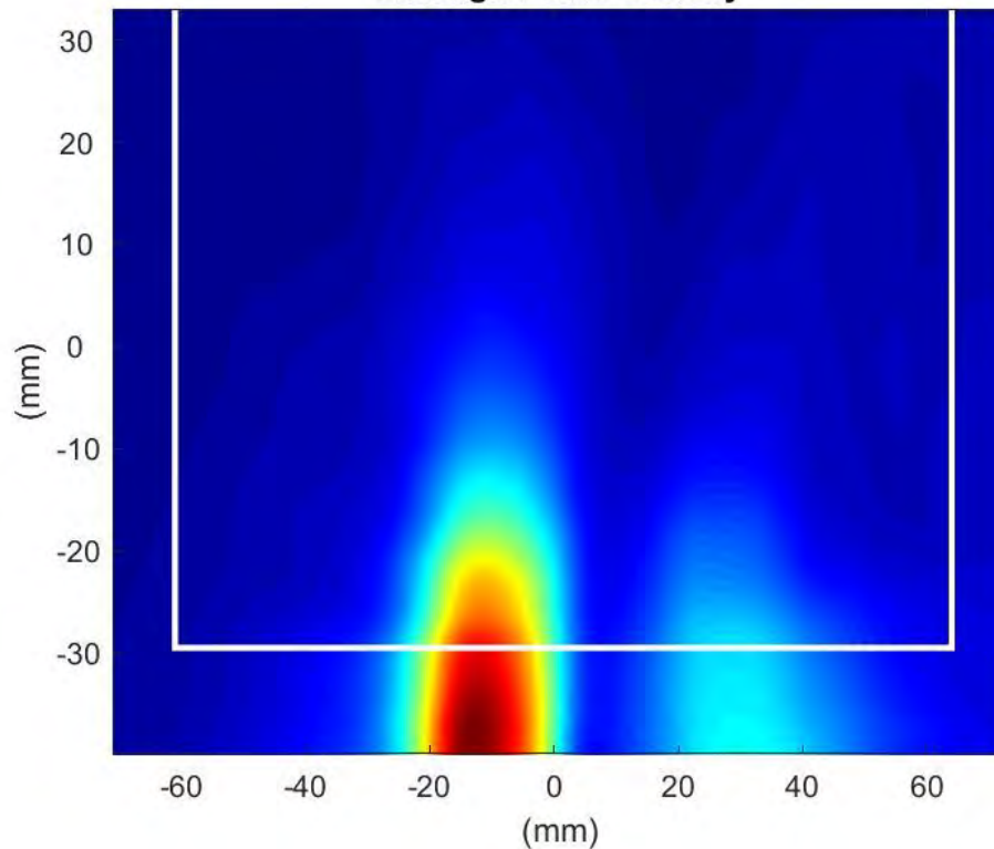
Phaser2 Beam Pair:61-187 Surface:S1 Average Power Density
