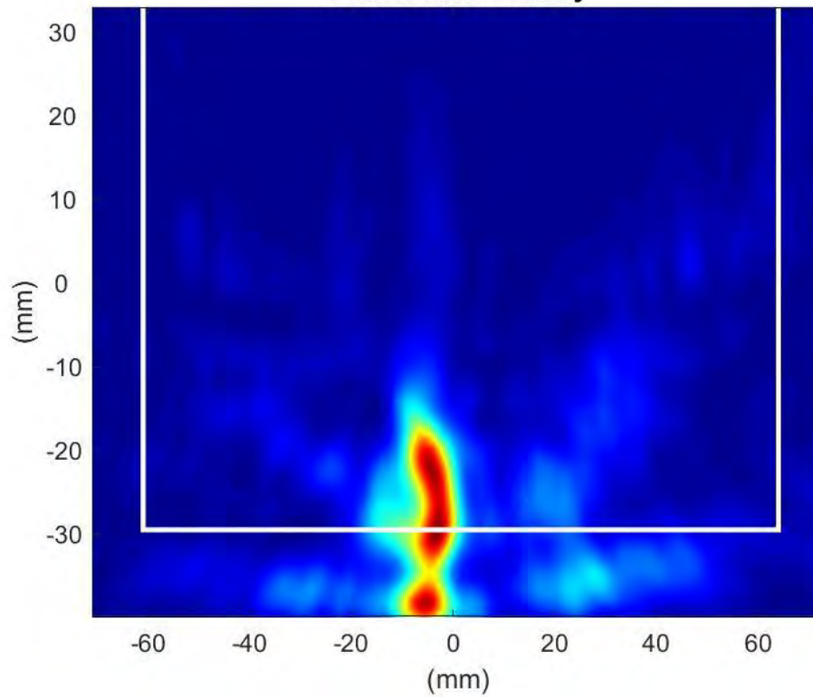
Phaser2 Beam Pair:49-175 Surface:S2 Average Power Density
