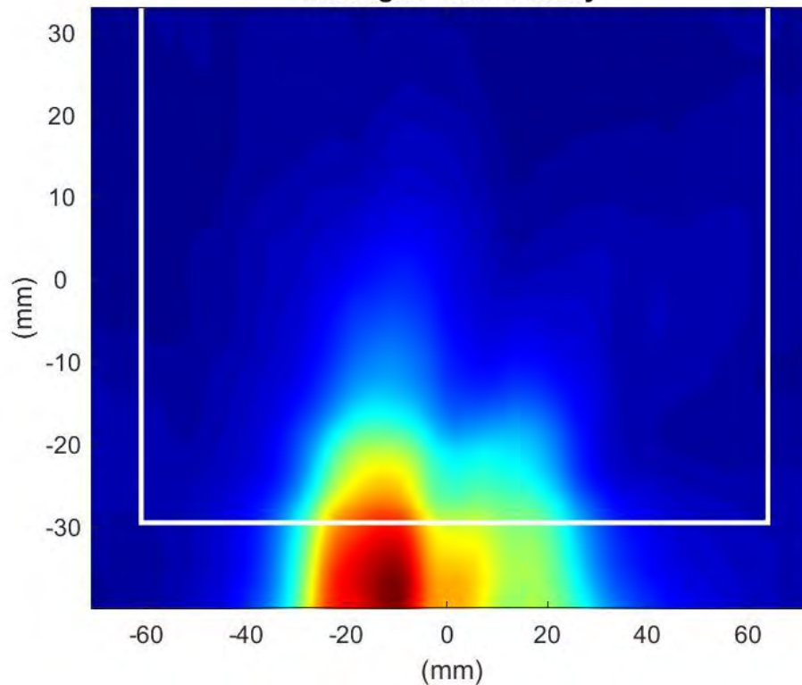
Phaser2 Beam Pair:60-190 Surface:S1 Average Power Density
