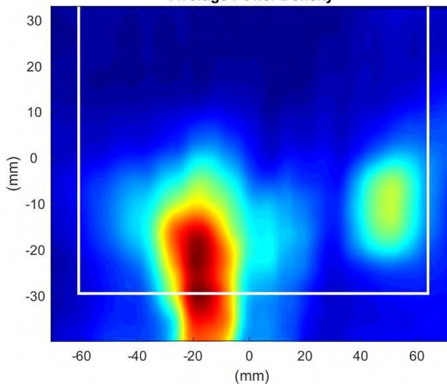
Phaser2 Beam Pair:34-162 Surface:S2 Average Power Density
