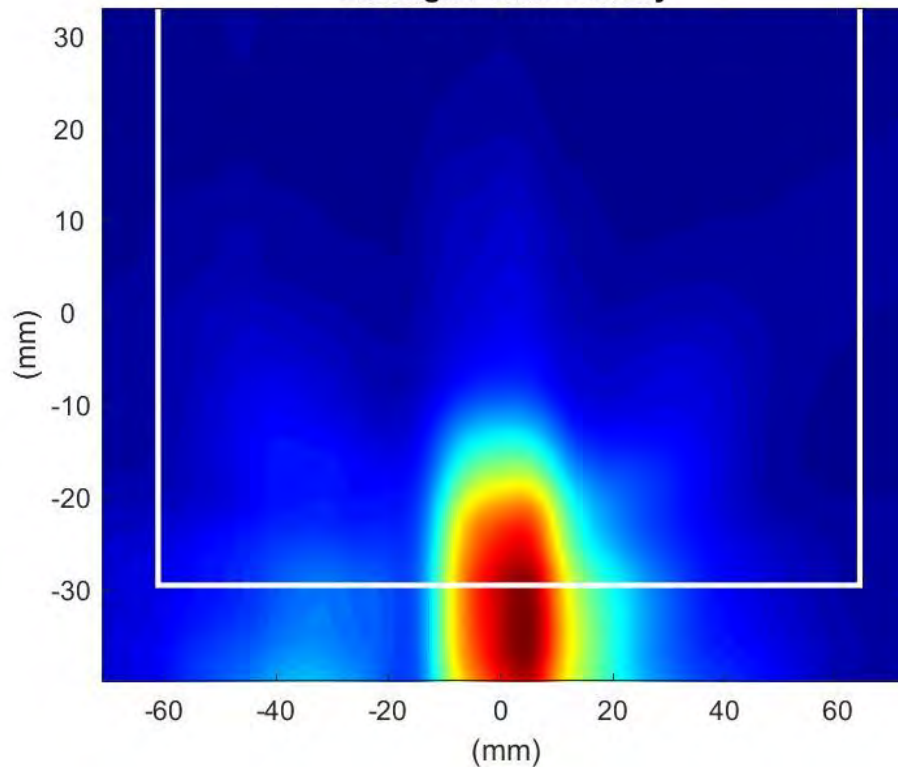
Phaser2 Beam Pair:62-188 Surface:S2 Average Power Density
