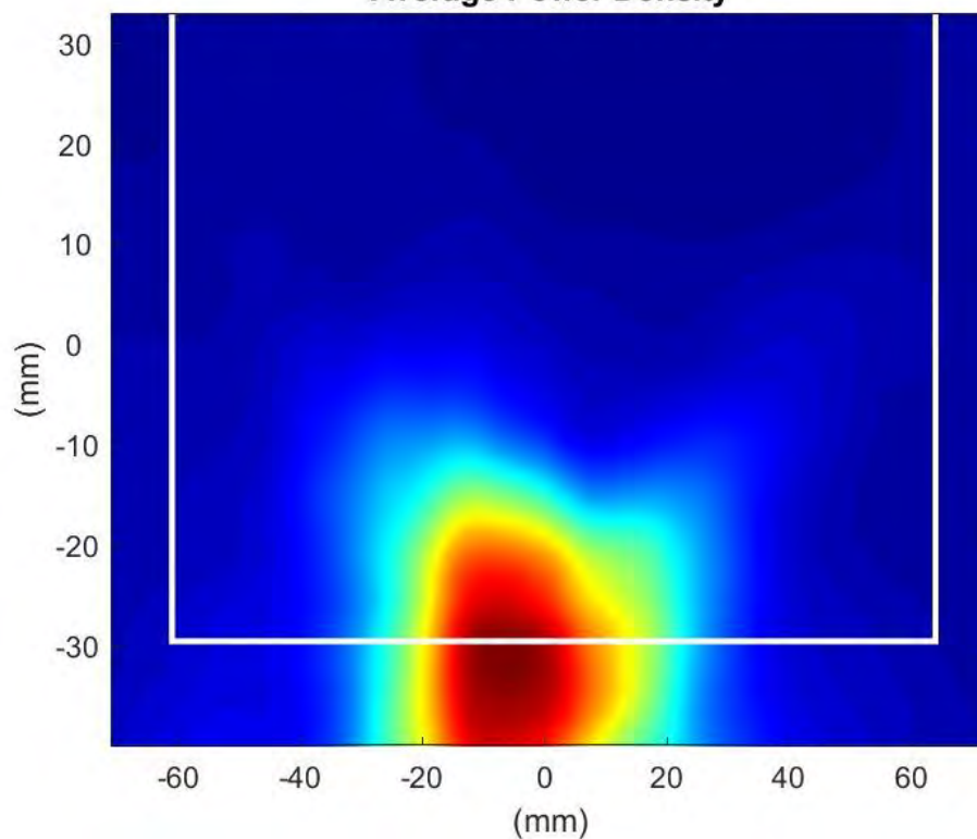
Phaser2 Beam Pair:4-132 Surface:S2 Average Power Density
