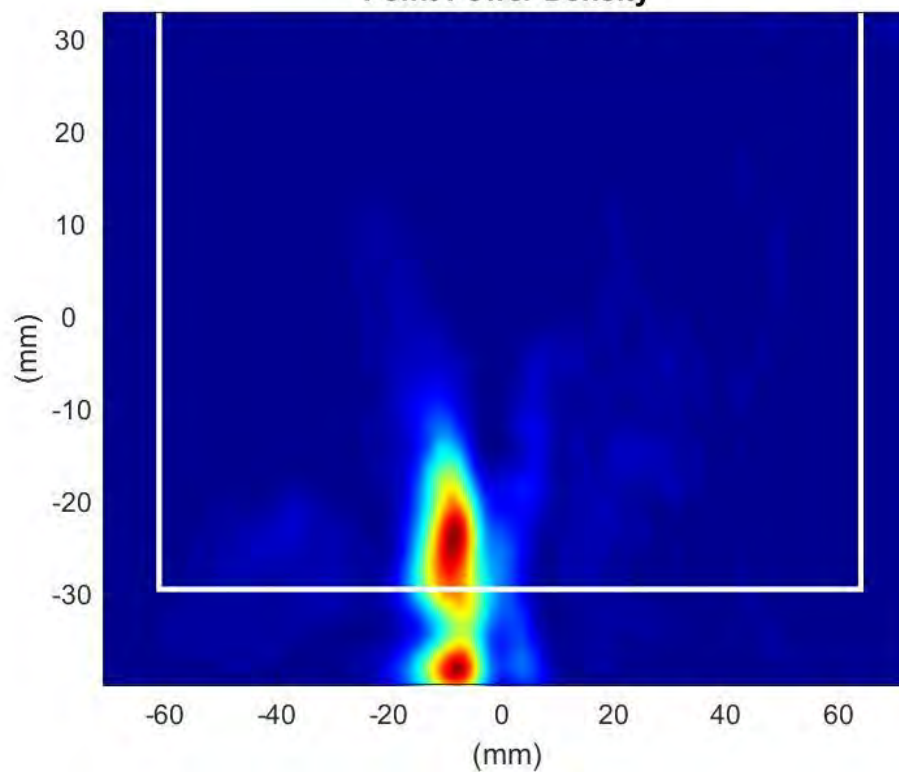
Phaser2 Beam:187 Surface:S2 Average Power Density
