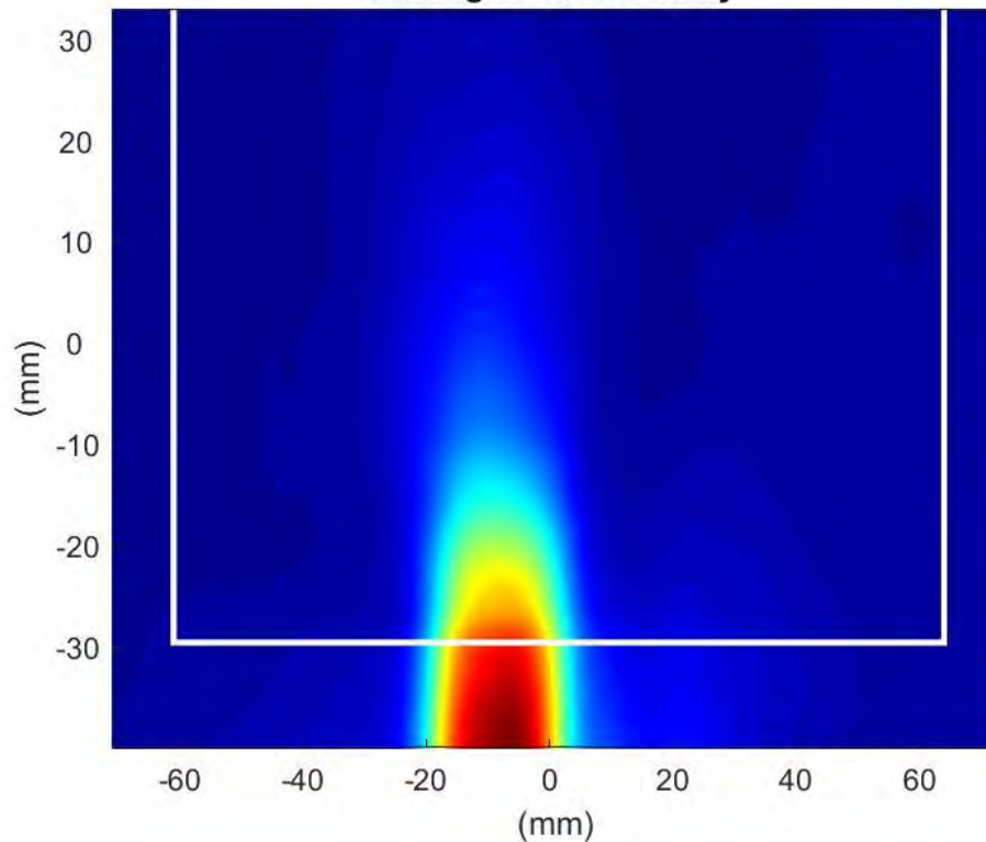
Phaser2 Beam:187 Surface:S1 Average Power Density
