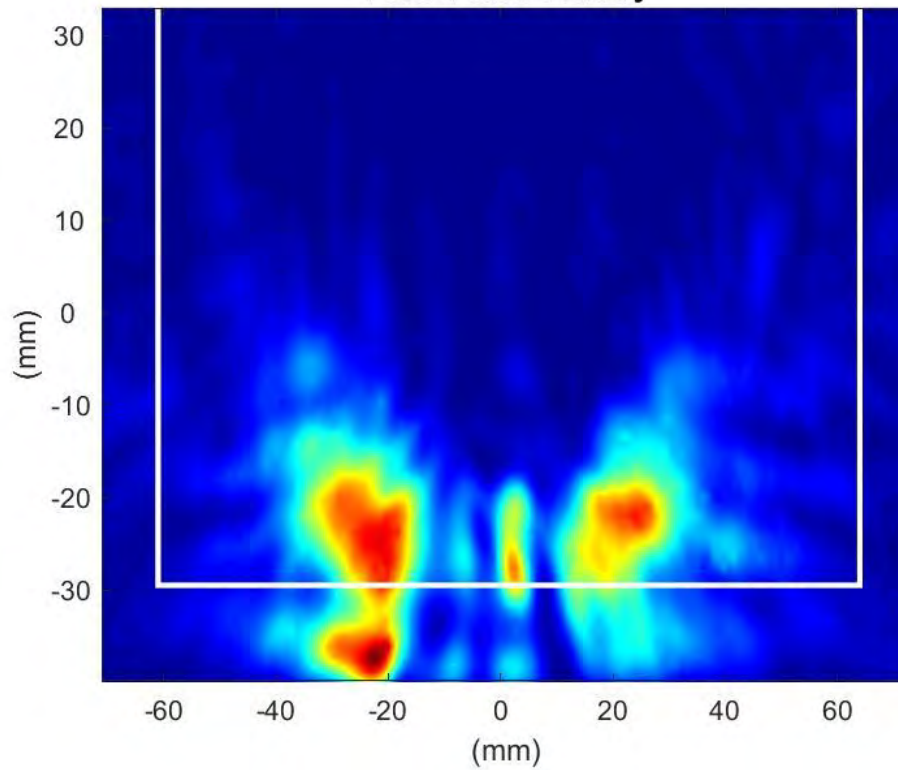
Phaser2 Beam:190 Surface:S2 Average Power Density
