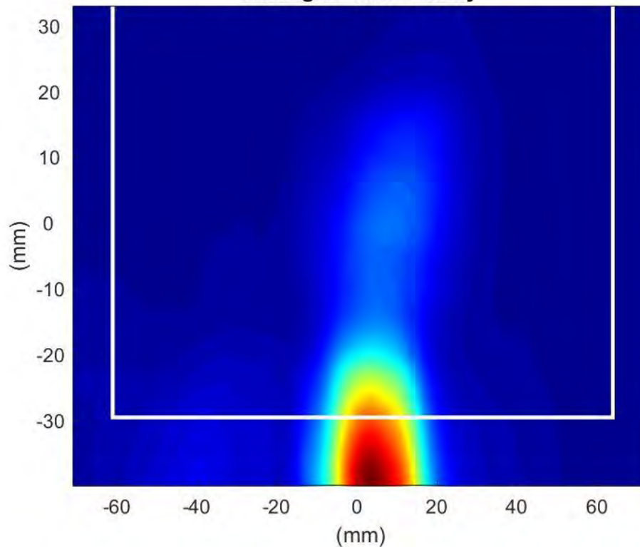
Phaser2 Beam Pair:35-163 Surface:S1 Average Power Density
