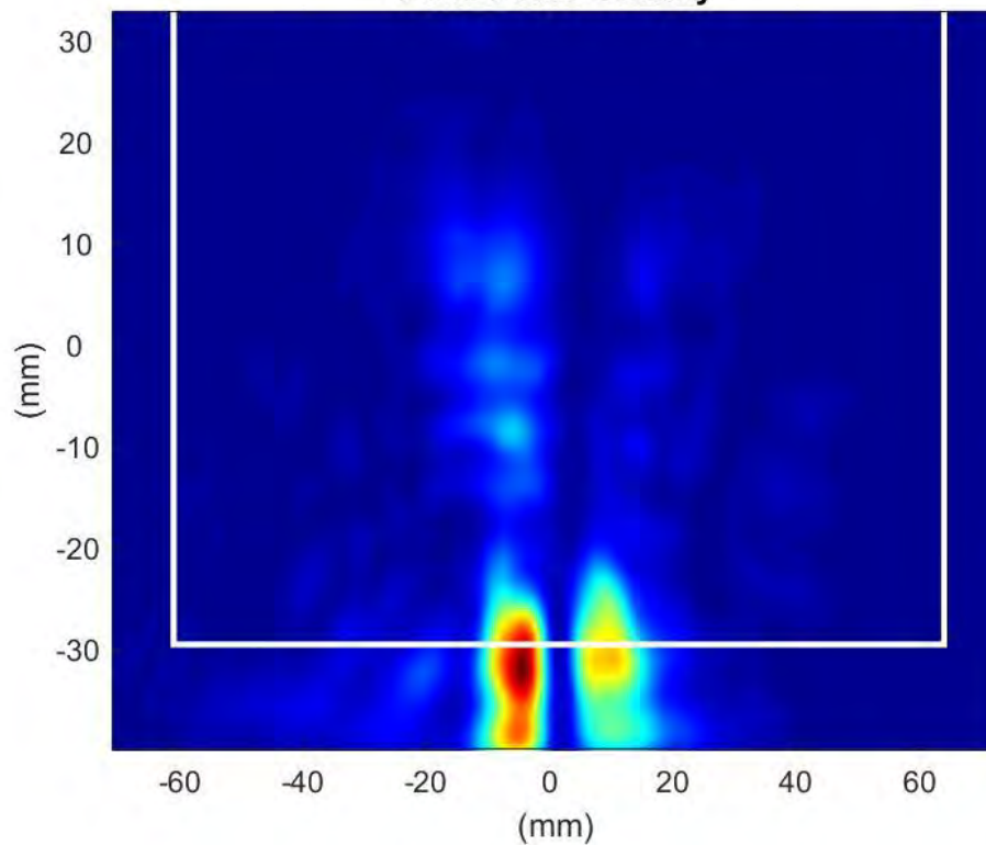
Phaser2 Beam Pair:5-133 Surface:S1 Average Power Density
