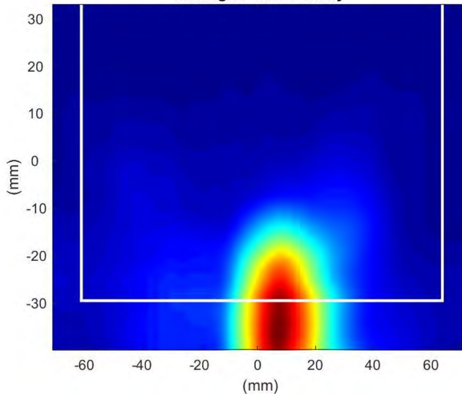
Phaser2 Beam Pair:18-147 Surface:S2 Average Power Density
