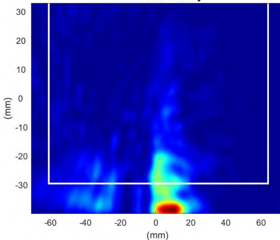
Phaser2 Beam Pair:50-176 Surface:S1 Average Power Density
