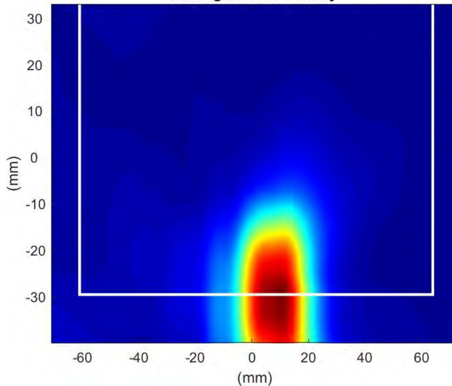
Phaser2 Beam:189 Surface:S2 Average Power Density
