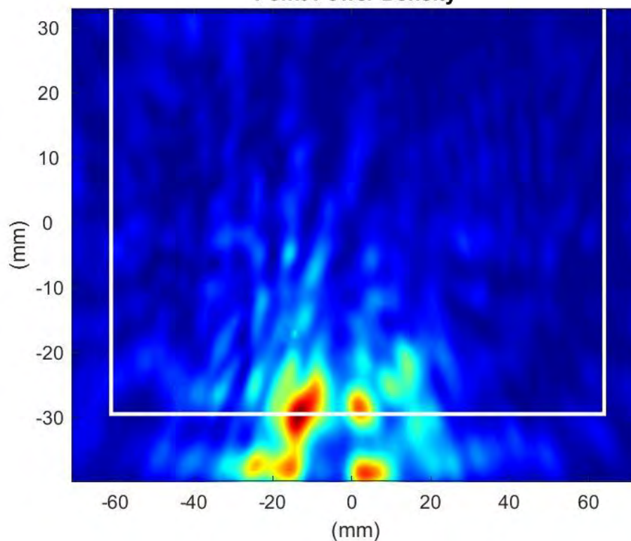
Phaser2 Beam Pair:47-178 Surface:S1 Average Power Density
