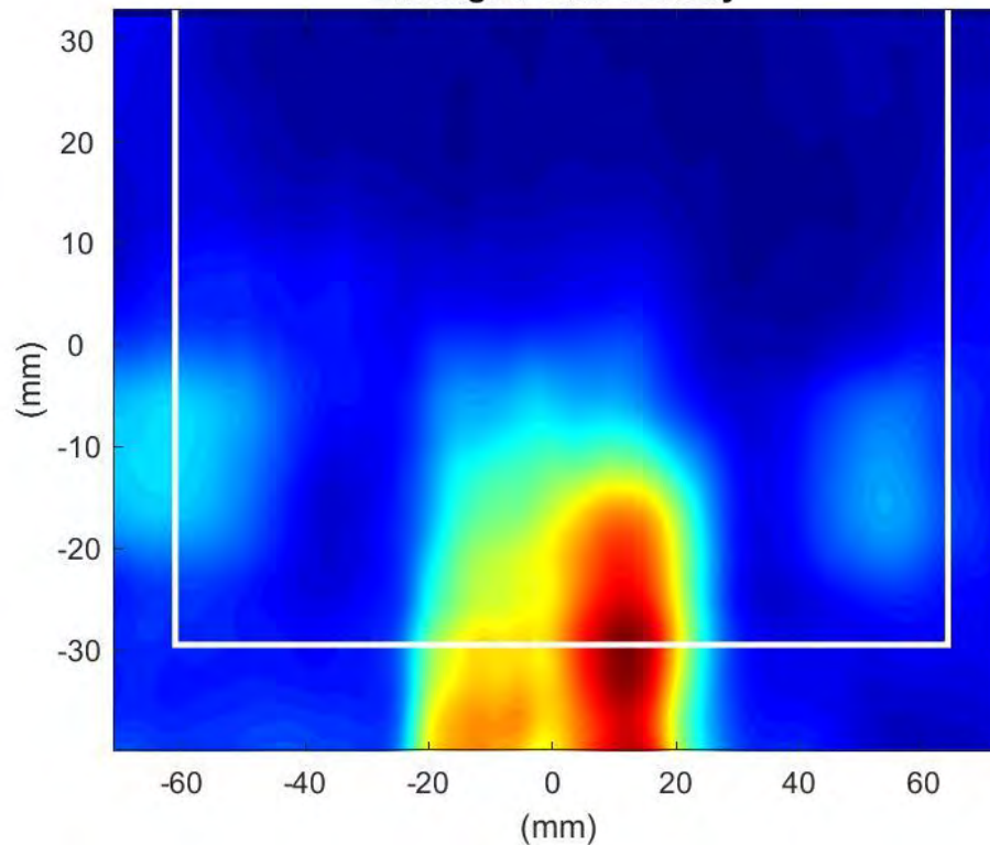
Phaser2 Beam Pair:5-133 Surface:S2 Average Power Density
