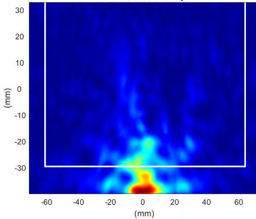
Phaser2 Beam Pair:33-160 Surface:S1 Average Power Density
