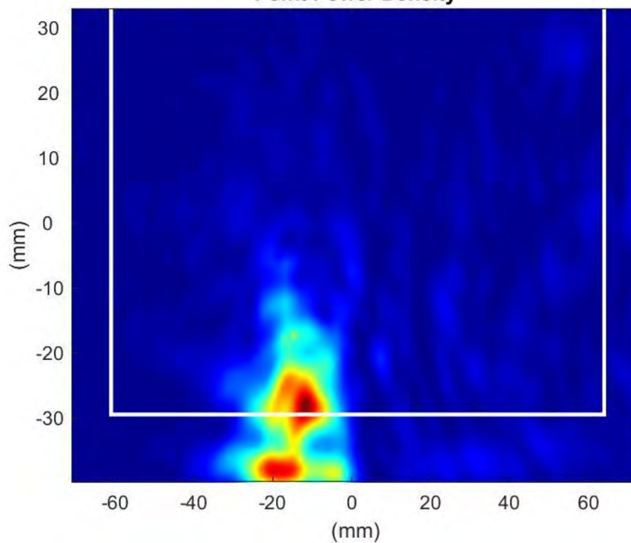
Phaser2 Beam Pair:48-174 Surface:S1 Average Power Density
