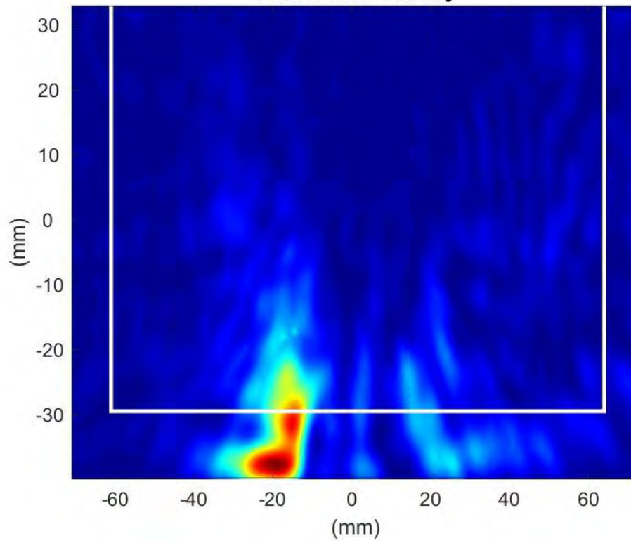
Phaser2 Beam:178 Surface:S1 Average Power Density
