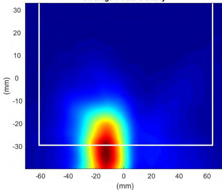
Phaser2 Beam Pair:19-146 Surface:S2 Average Power Density
