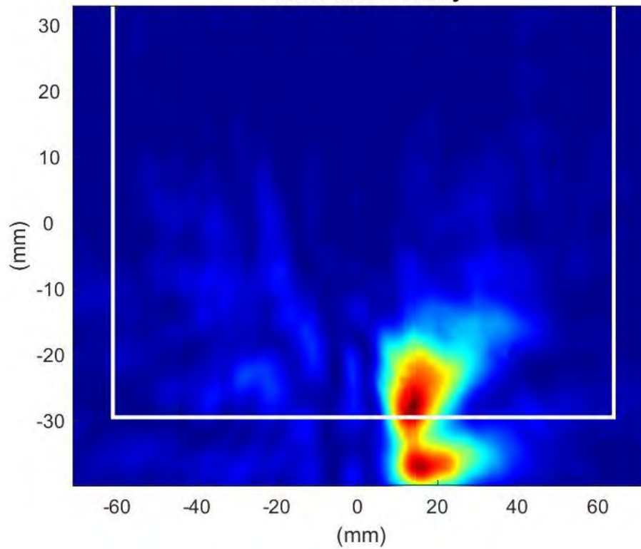
Phaser2 Beam Pair:46-177 Surface:S2 Average Power Density
