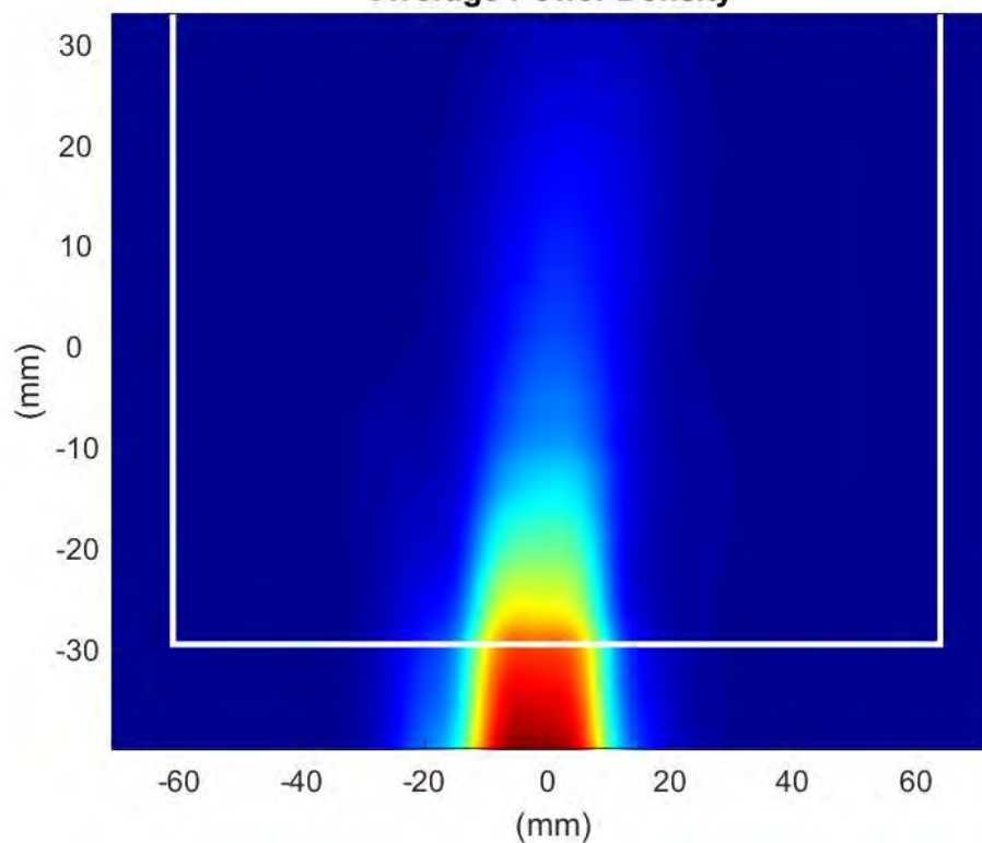
Phaser2 Beam:188 Surface:S1 Average Power Density
