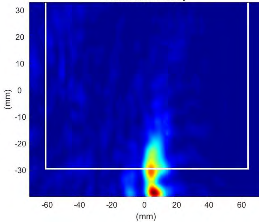
Phaser2 Beam:189 Surface:S1 Average Power Density
