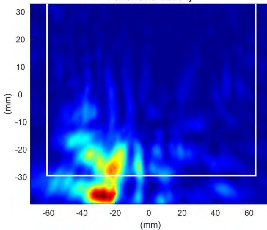
Phaser2 Beam Pair:20-148 Surface:S2 Average Power Density
