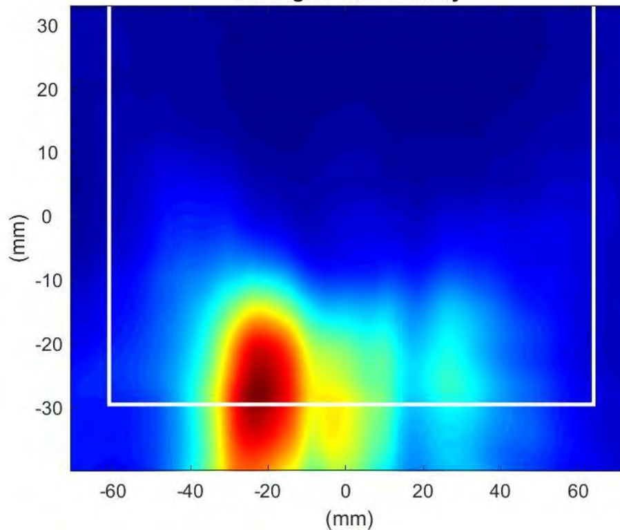
Phaser2 Beam Pair:47-178 Surface:S2 Average Power Density
