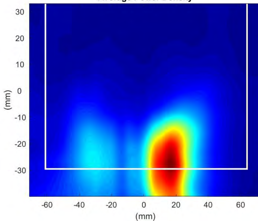
Phaser2 Beam:177 Surface:S2 Average Power Density
