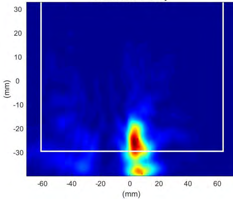
Phaser2 Beam Pair:50-176 Surface:S2 Average Power Density
