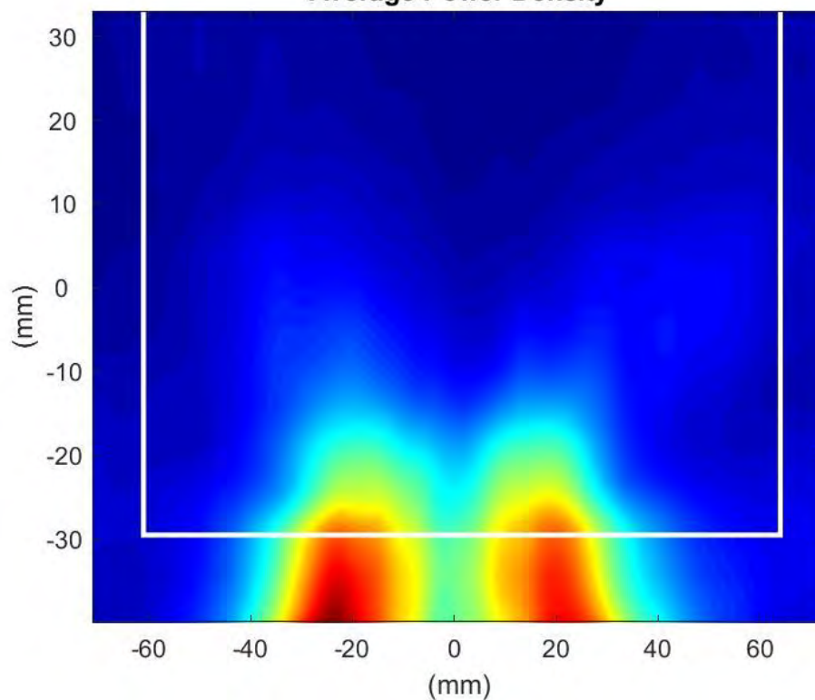
Phaser2 Beam:190 Surface:S1 Average Power Density
