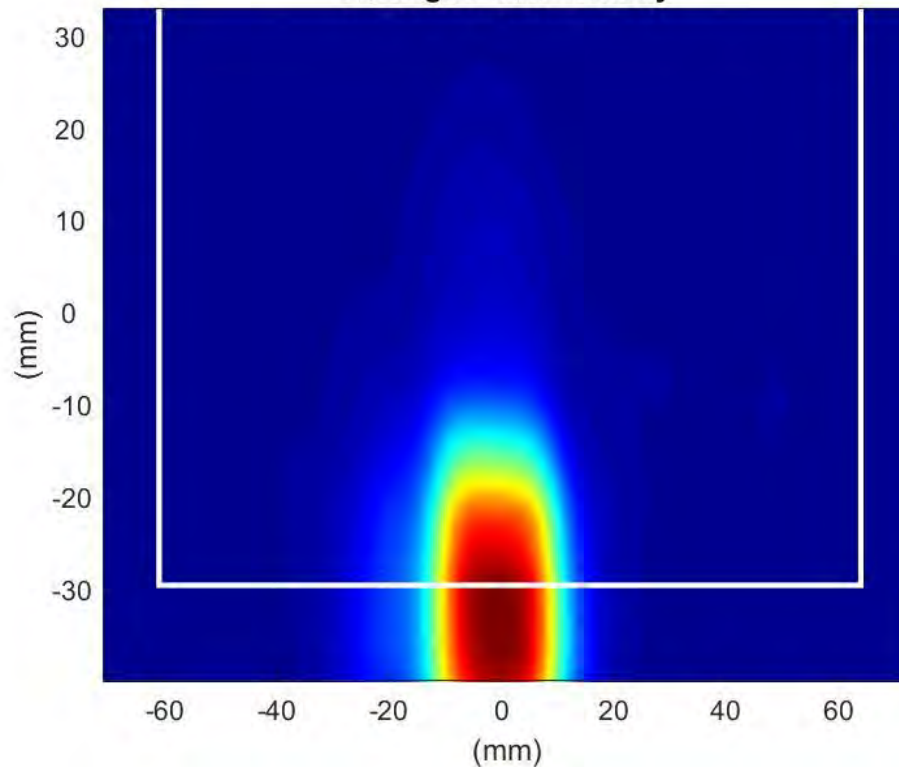
Phaser2 Beam:188 Surface:S2 Average Power Density
