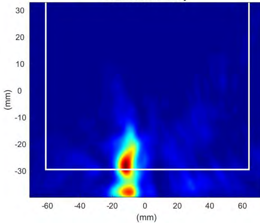
Phaser2 Beam Pair:61-187 Surface:S2 Average Power Density
