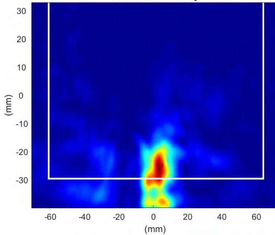
Phaser2 Beam Pair:32-161 Surface:S2 Average Power Density
