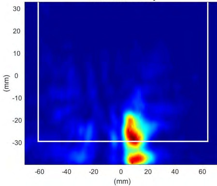
Phaser2 Beam Pair:59-189 Surface:S2 Average Power Density
