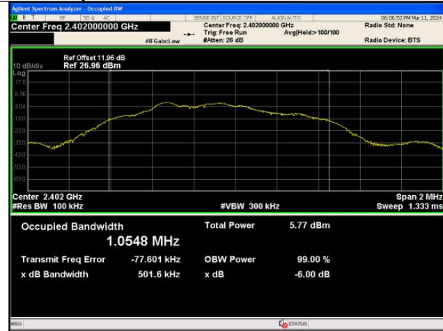
LE_Channel 0
