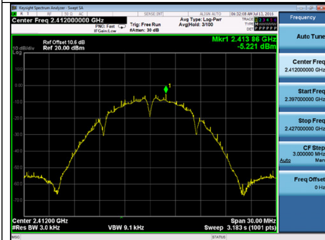
PSD-2.4G-802.11b Low-chain3
