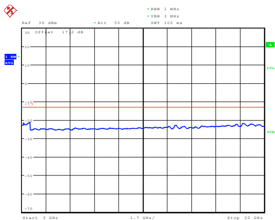
LTE Band 25 3MHz CH-Middle 3GHz~20GHz
