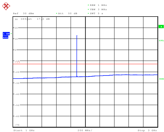
LTE Band 25 3MHz CH-Middle 1GHz~3GHz
