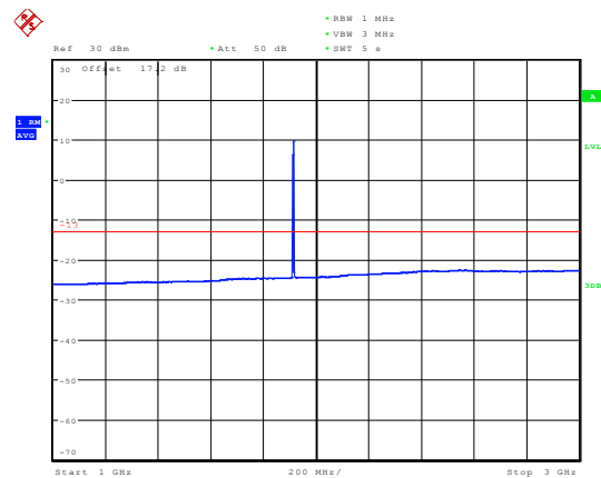
LTE Band 25 3MHz CH-High 1GHz~3GHz
