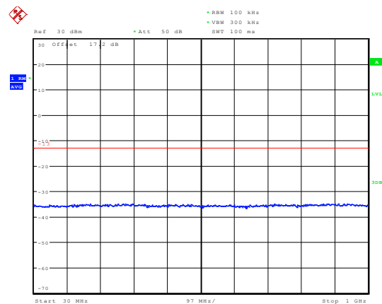
LTE Band 25 3MHz CH-High 30MHz~1GHz
