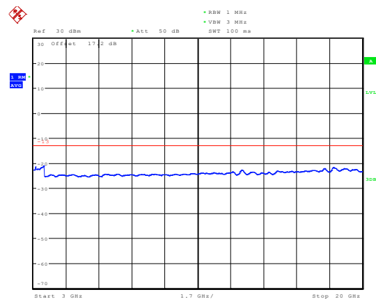
LTE Band 25 3MHz CH-High 3GHz~20GHz
