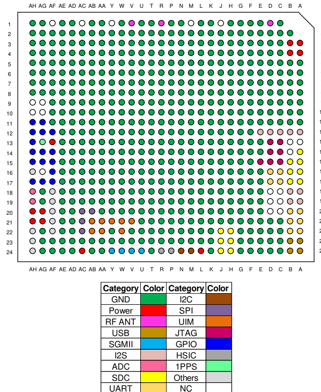
Figure 1: VMC-9628NV1 Pin-out (Top View)
