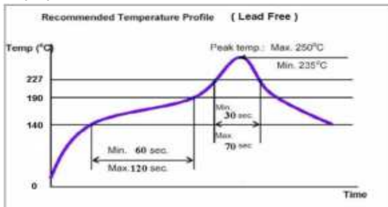
Figure 5: Reflow Profile
