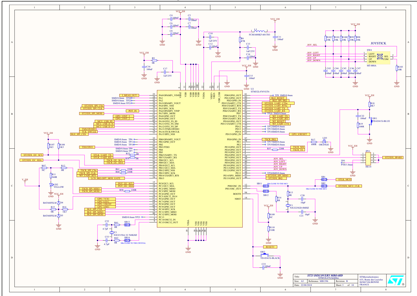
Figure 11. MB1396 - MCU
