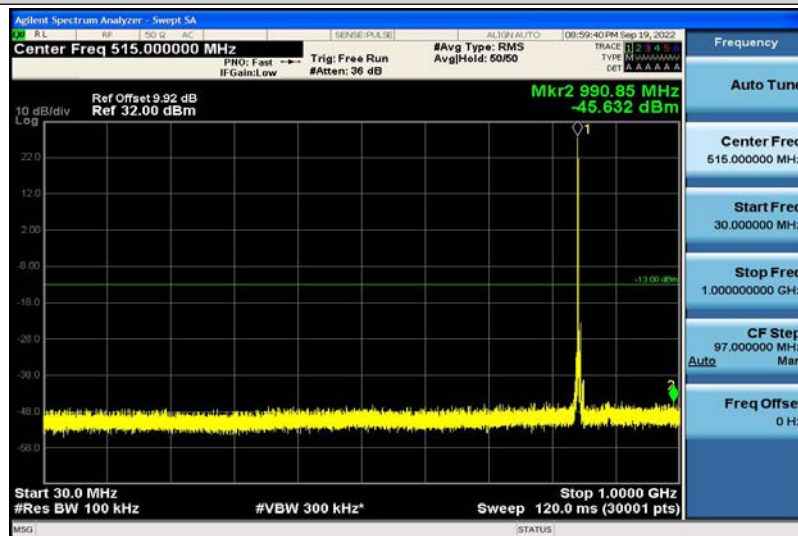
Band5-5MHz-16QAM-20625-1RB#0-30~1000MHz
