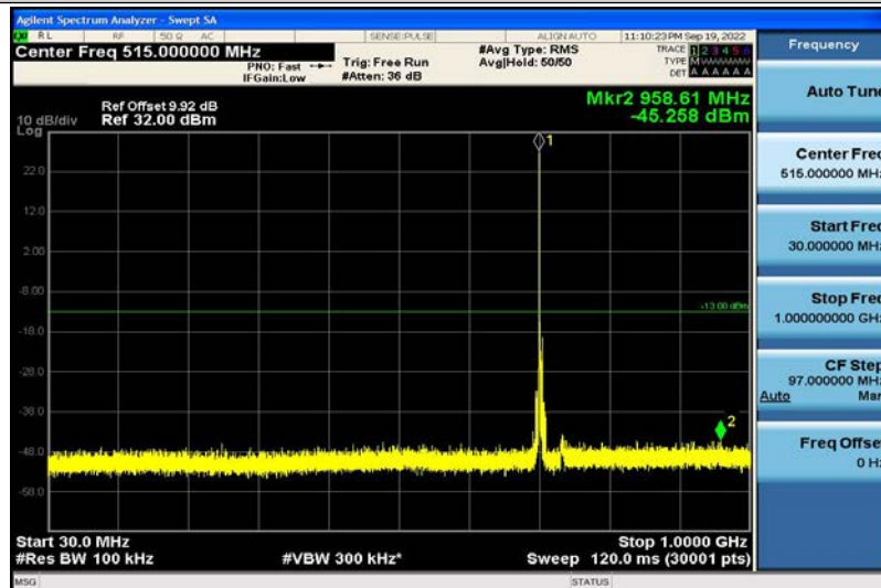
Band17-5MHz-16QAM-23790-1RB#0-30~1000MHz
