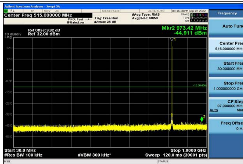
Band5-1.4MHz-16QAM-20407-1RB#0-30~1000MHz
