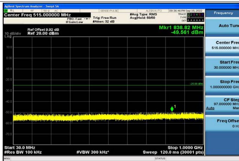
Band7-5MHz-QPSK-20775-1RB#0-30~1000MHz
