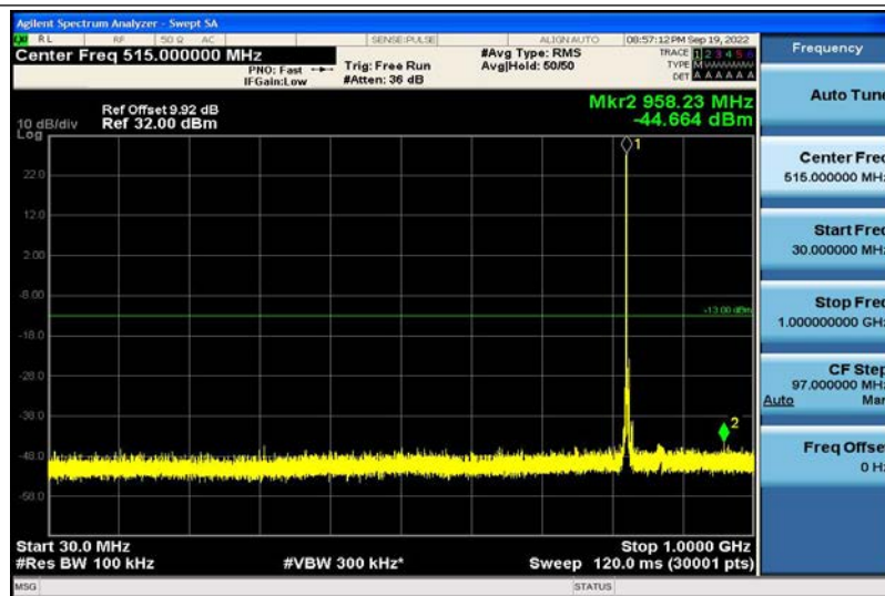
Band5-5MHz-16QAM-20425-1RB#0-30~1000MHz
