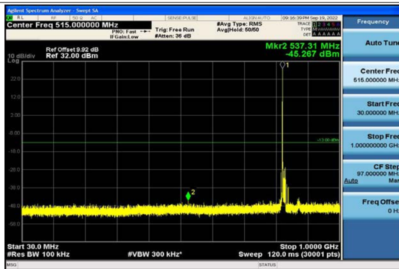
Band5-10MHz-16QAM-20450-1RB#0-30~1000MHz
