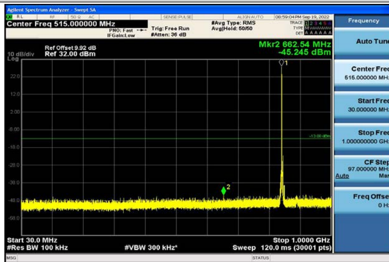
Band5-5MHz-QPSK-20625-1RB#0-30~1000MHz
