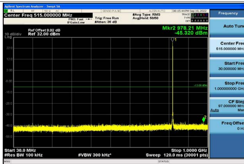
Band5-1.4MHz-QPSK-20407-1RB#0-30~1000MHz
