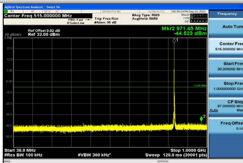
Band5-3MHz-16QAM-20525-1RB#0-30~1000MHz
