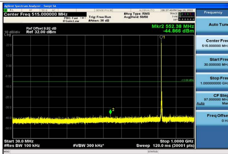
Band5-3MHz-16QAM-20415-1RB#0-30~1000MHz
