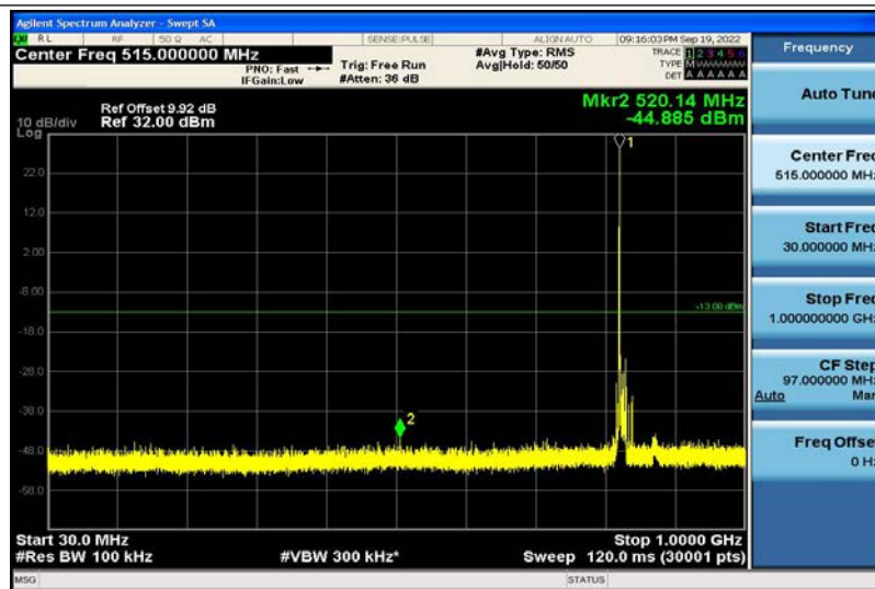
Band5-10MHz-QPSK-20450-1RB#0-30~1000MHz
