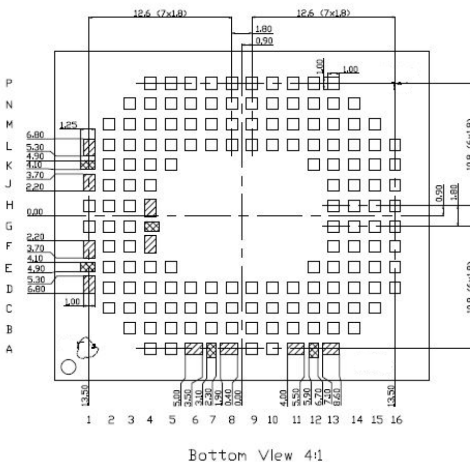
Figure 24: Dimensions of PLS63-X (all dimensions in mm)
