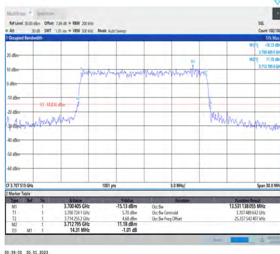
1-N78-3700-3800-30-15-L-9-CP-256QAM-Outer_Full-38@0-Ant1-13.531-14.310-≤15-PASS
