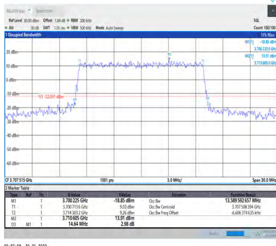
1-N78-3700-3800-30-15-L-6-CP-QPSK-Outer_Full-38@0-Ant1-13.59-14.640-≤15-PASS
