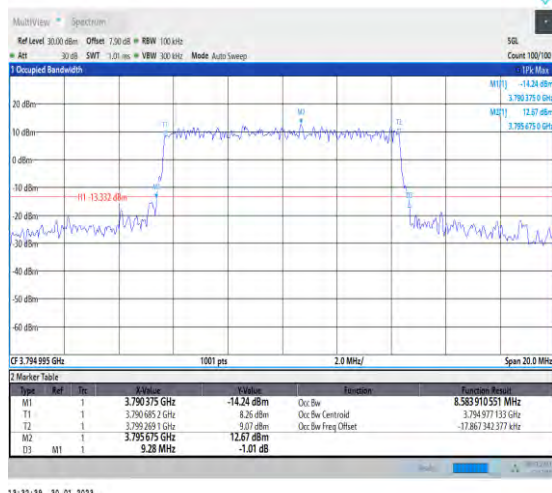
1-N78-3700-3800-30-10-H-7-CP-16QAM-Outer_Full-24@0-Ant1-8.584-9.280-≤10-PASS
