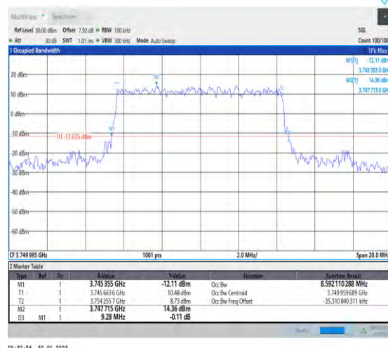
1-N78-3700-3800-30-10-M-1-DFT-QPSK-Outer_Full- 24@0-Ant1-8.592-9.280-≤10-PASS
