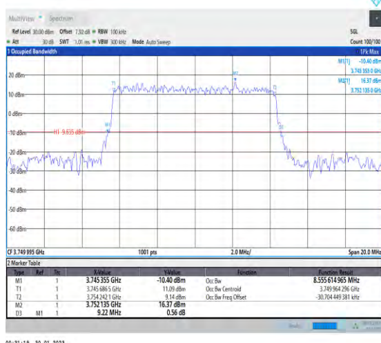
1-N78-3700-3800-30-10-M-2-DFT-PI2BPSK-Outer_ Full-24@0-Ant1-8.556-9.220-≤10-PASS
