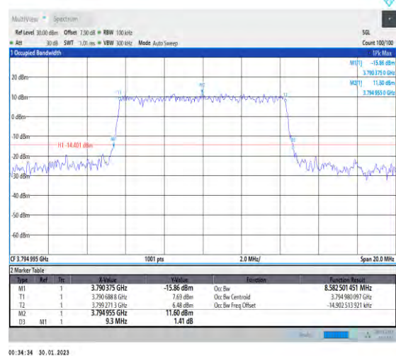
1-N78-3700-3800-30-10-H-6-CP-QPSK-Outer_Full-2 4@0-Ant1-8.583-9.300-≤10-PASS
