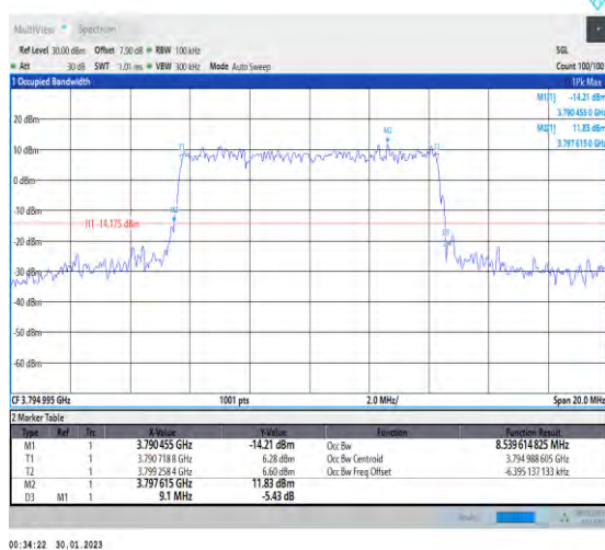
1-N78-3700-3800-30-10-H-5-DFT-256QAM-Outer_F ull-24@0-Ant1-8.54-9.100-≤10-PASS
