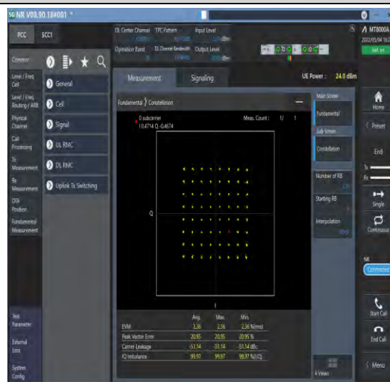
1-N78-3700-3800--30-100-M-4-DFT-64QAM-Outter_Full-270@0-Ant1-see graph-PASS
