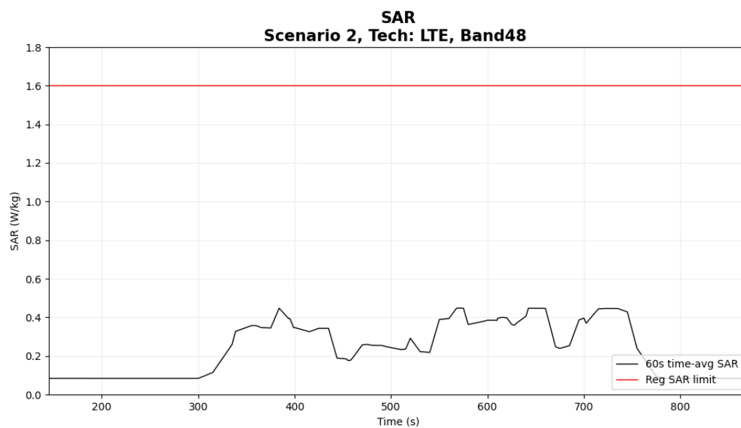
Figure 5- 28 Time-averaged SAR
