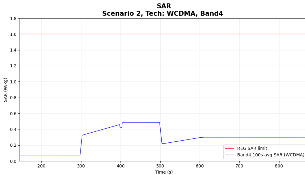
Figure 6-13 Time-averaged SAR
