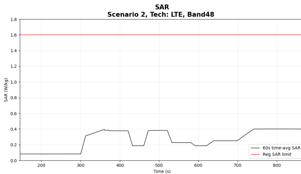
Figure 5- 26 Time-averaged SAR
