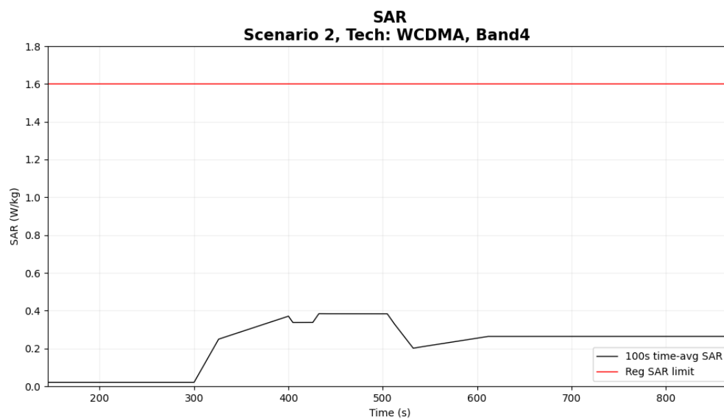
Figure 5- 19 Time-averaged SAR
