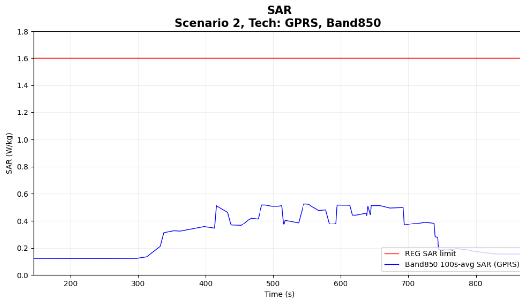
Figure 6-18 Time-averaged SAR
