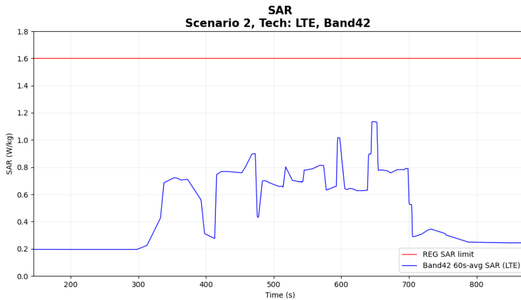
Figure 6-8 Time-averaged SAR
