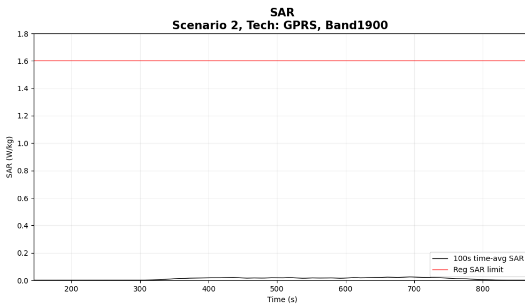
Figure 5- 10 Time-averaged SAR
