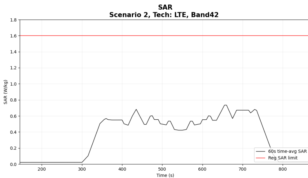
Figure 5- 24 Time-averaged SAR
