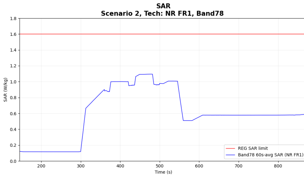
Figure 6-5 Time-averaged SAR
