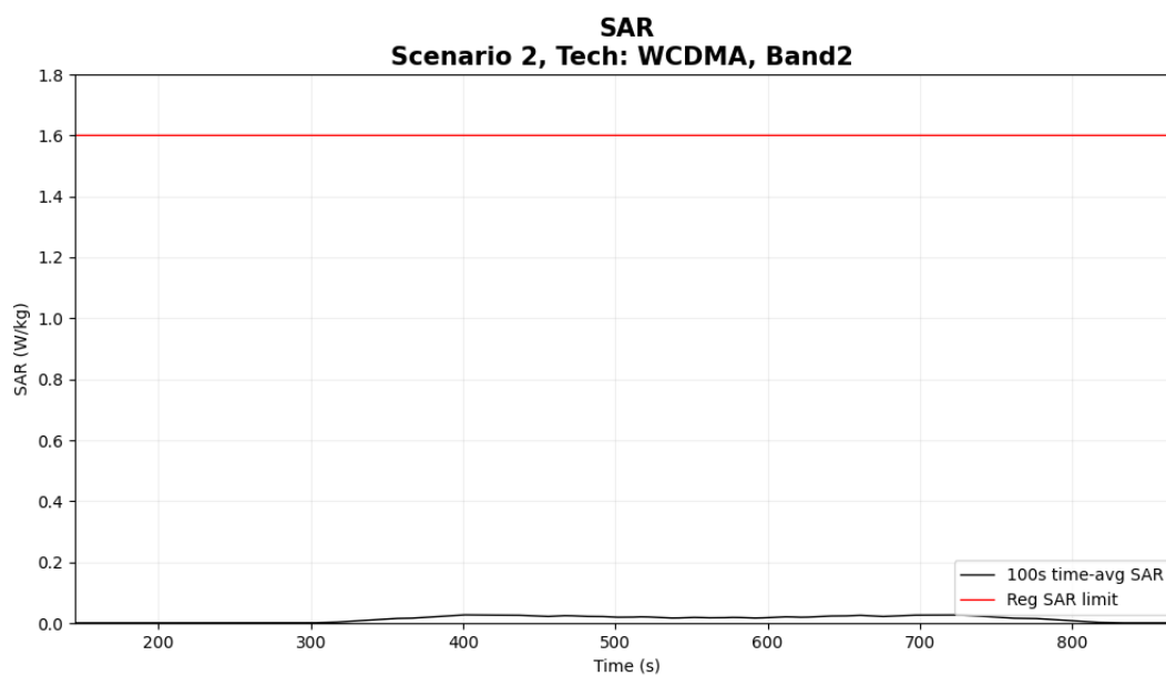
Figure 5- 17 Time-averaged SAR
