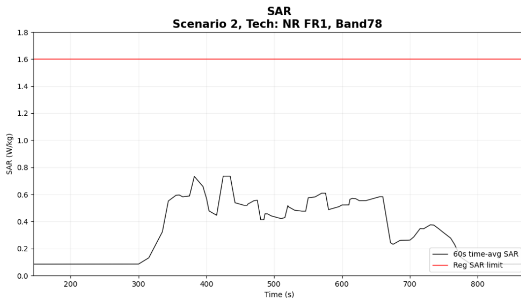
Figure 5- 36 Time-averaged SAR
