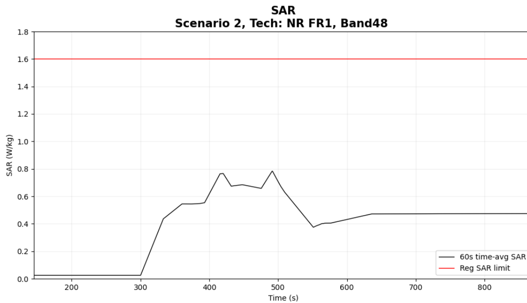
Figure 5- 30 Time-averaged SAR
