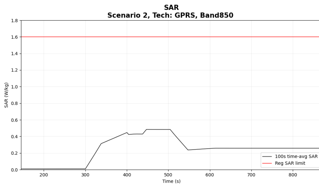
Figure 5- 12 Time-averaged SAR
