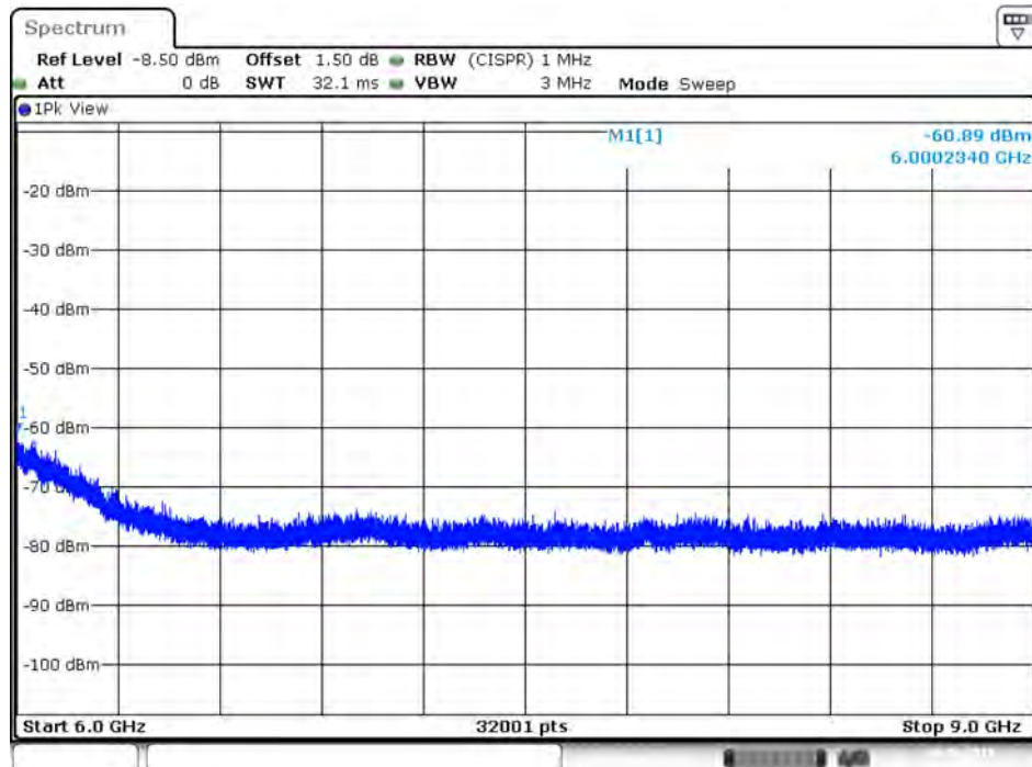
Plot on IEEE 802.11ac Nss1 MCS0 VHT80 / 5530 MHz / Peak / Port 1 / 6GHz~9GHz
