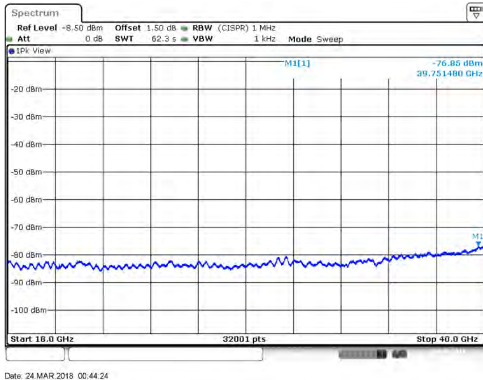
Plot on IEEE 802.11ac Nss1 MCS0 VHT80 / 5530 MHz / Peak / Port 1 / 18GHz~40GHz
