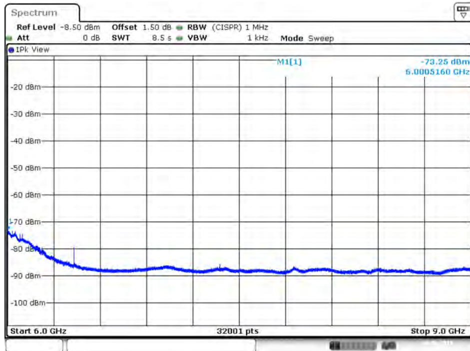
Plot on IEEE 802.11ac Nss1 MCS0 VHT80 / 5530 MHz / Average / Port 1 / 6GHz~9GHz
