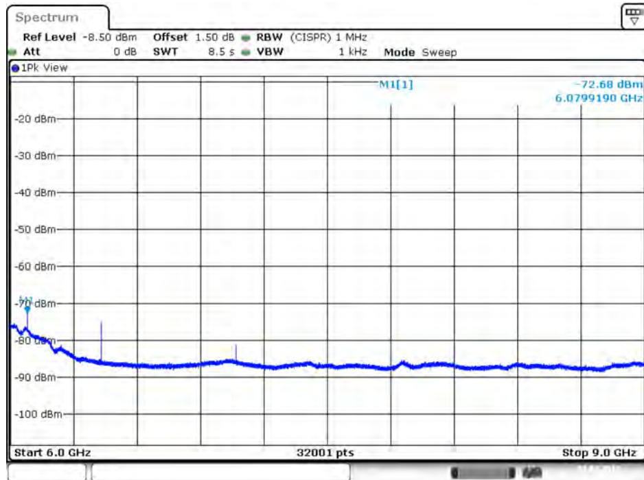
Plot on IEEE 802.11ac Nss1 MCS0 VHT20 / 5300 MHz / Average / Port 2 / 6GHz~9GHz
