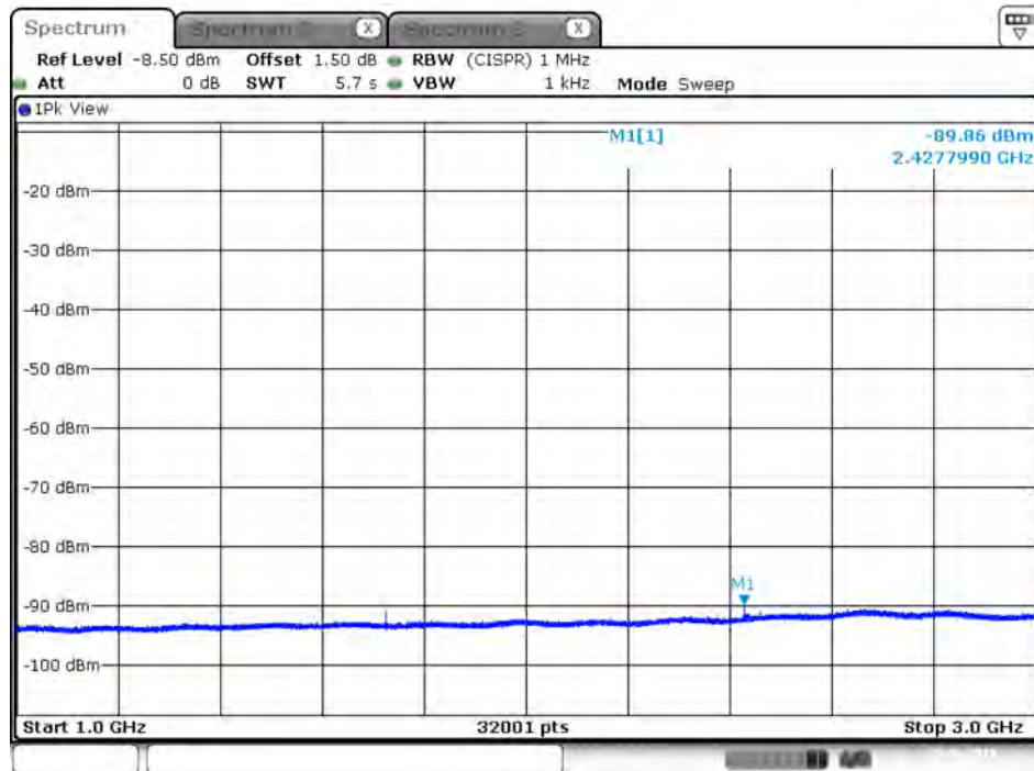
Plot on IEEE 802.11ac Nss1 MCS0 VHT20 / 5500 MHz / Average / Port 2 / 1GHz~3GHz
