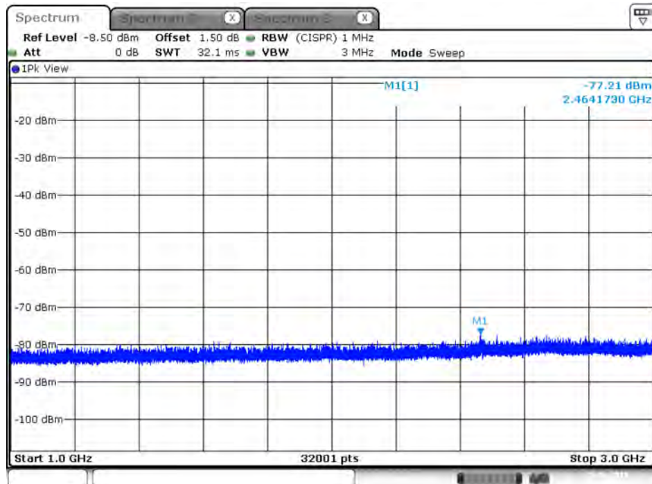
Plot on IEEE 802.11ac Nss1 MCS0 VHT20 / 5500 MHz / Peak / Port 2 / 1GHz~3GHz
