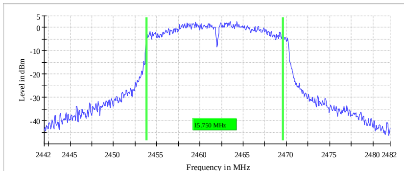
6 dB Bandwidth
