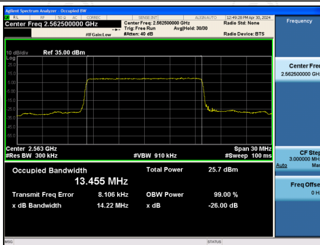
Band41-15MHz-16QAM-40315-75RB#0
