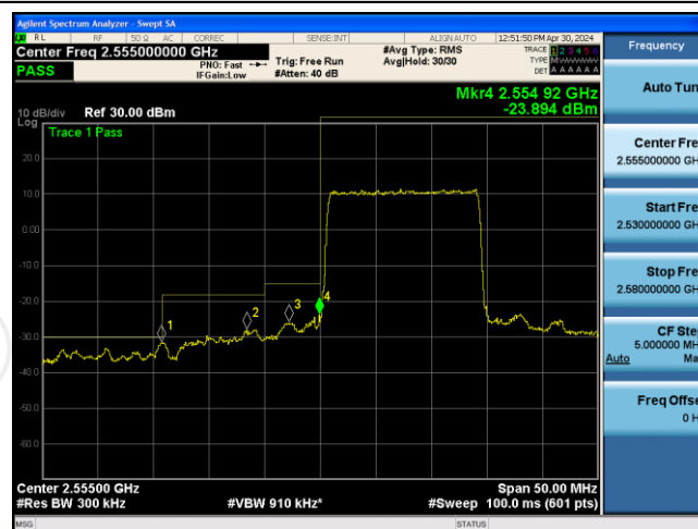
Band41-15MHz-QPSK-40315-75RB#0
