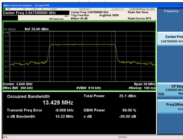
Band41-15MHz-QPSK-41165-75RB#0
