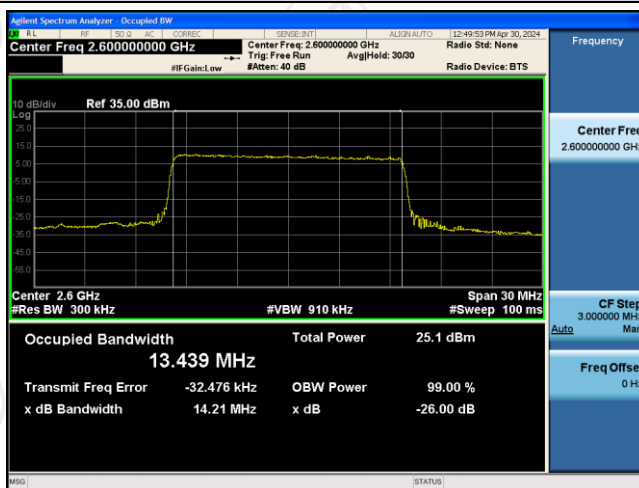
Band41-15MHz-16QAM-40690-75RB#0
