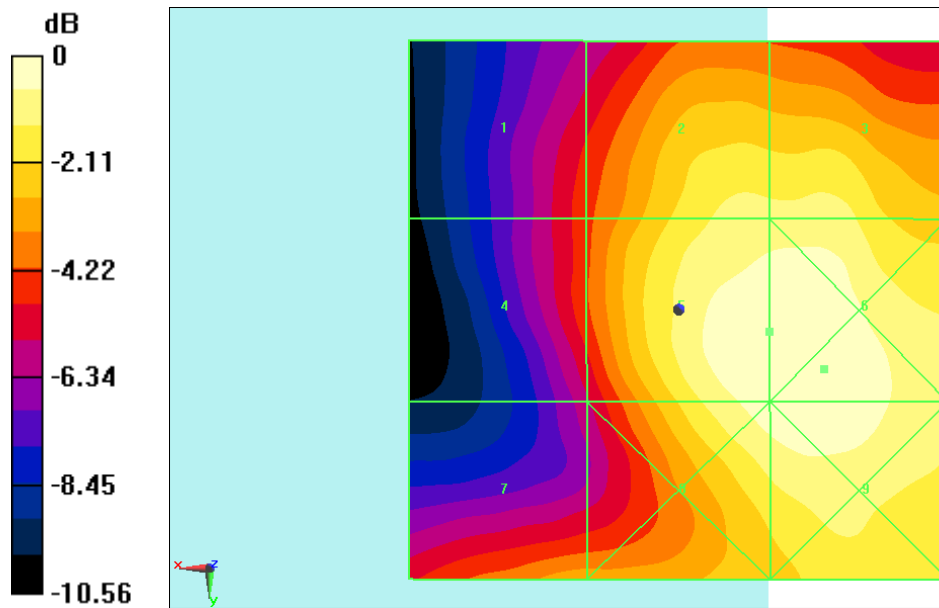
Fig B.2 HAC RF E-Field WIFI 2.4G
