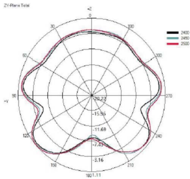
(2) Y-Z Plane(unit:dBi):
