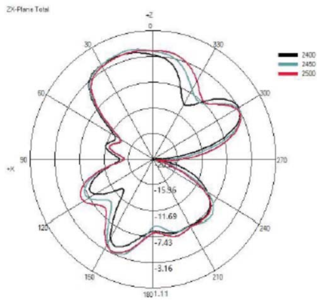
(1) X-Z Plane(unit:dBi):
