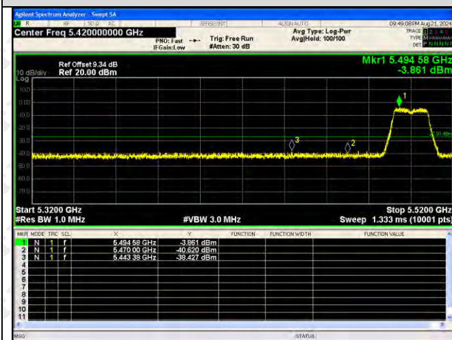
802.11ac(VH20)-5500
