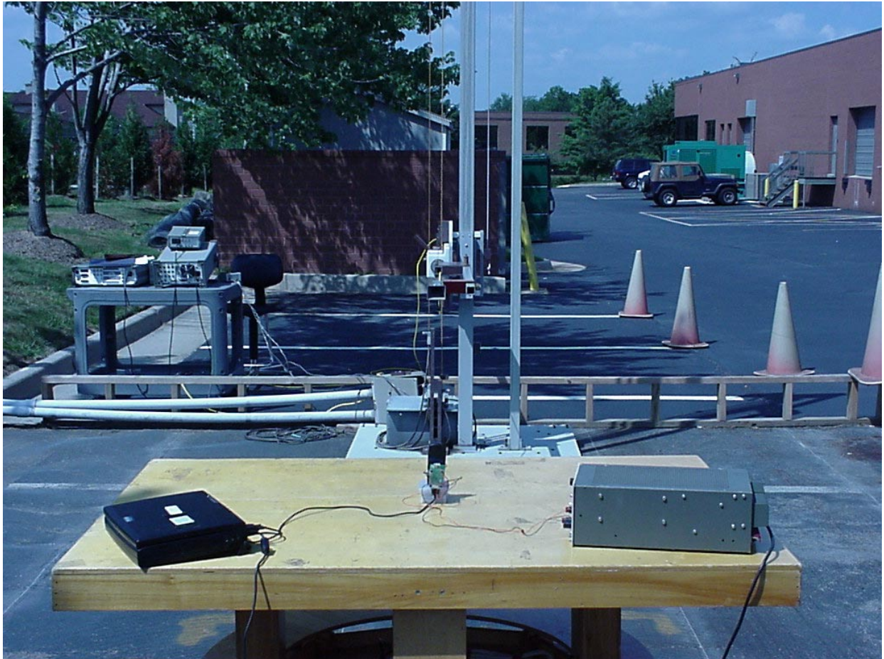
PHOTOGRAPH 2: RADIATED REAR VIEW
