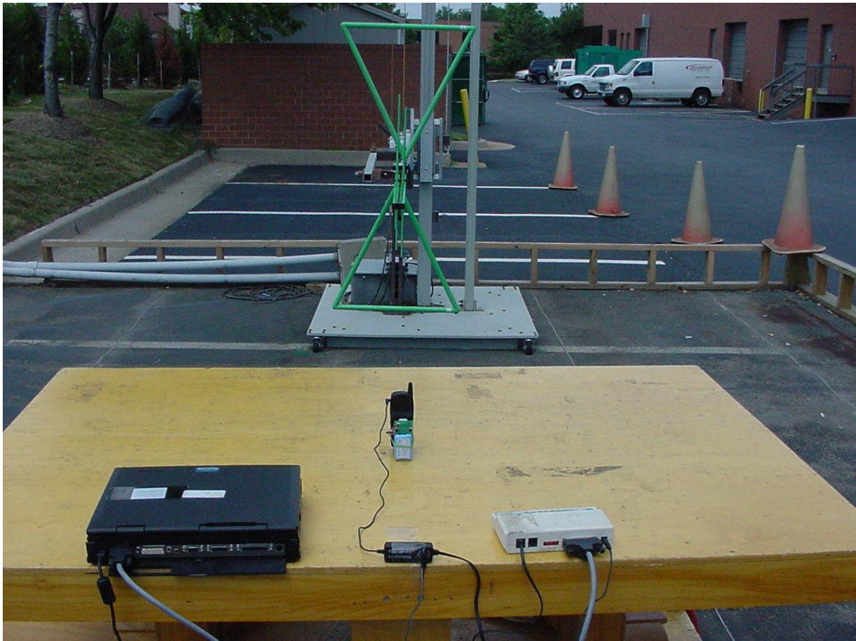
PHOTOGRAPH 4: RADIATED/DIGITAL WITH DATA TRANSFER CABLE BACK SIDE
