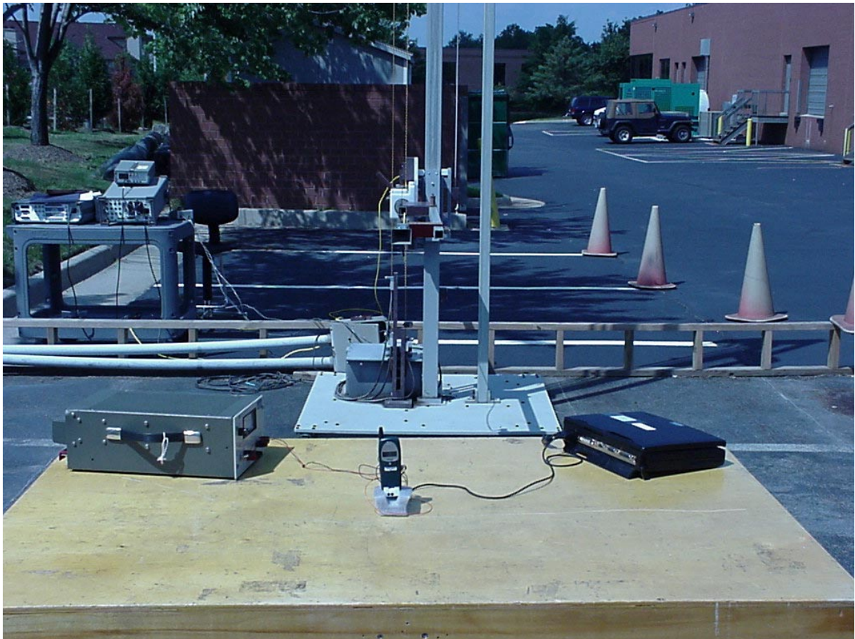
PHOTOGRAPH 3: RADIATED FRONT VIEW
