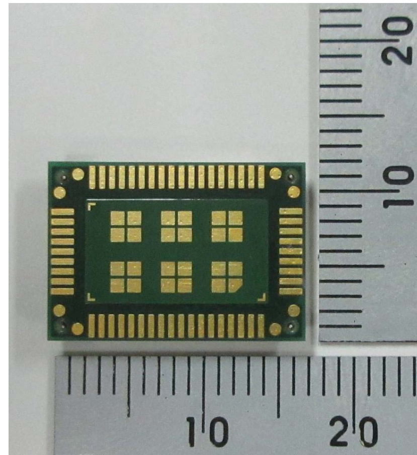
Bottom view
