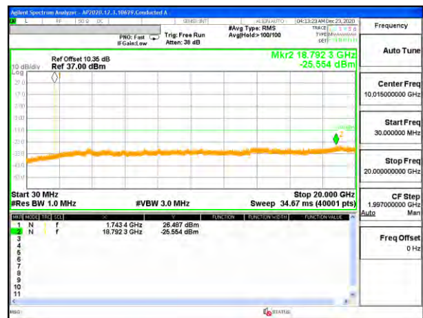
5G NR Band n66 5MHz 16QAM Middle Channel RB1-1
