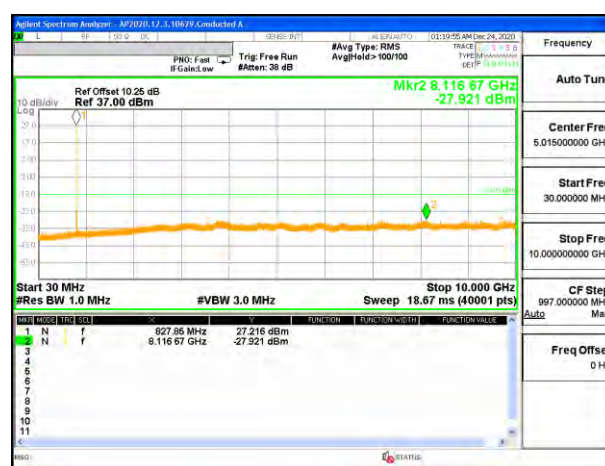
5G NR Band n5 20MHz BPSK Middle Channel RB1-1
