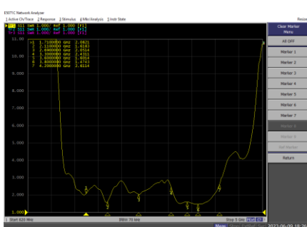
P10 ANT3 VSWR/Return Loss
