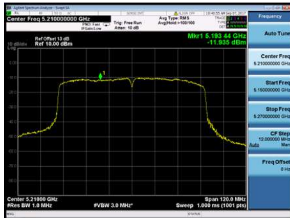
Channel 42 (5210MHz)
