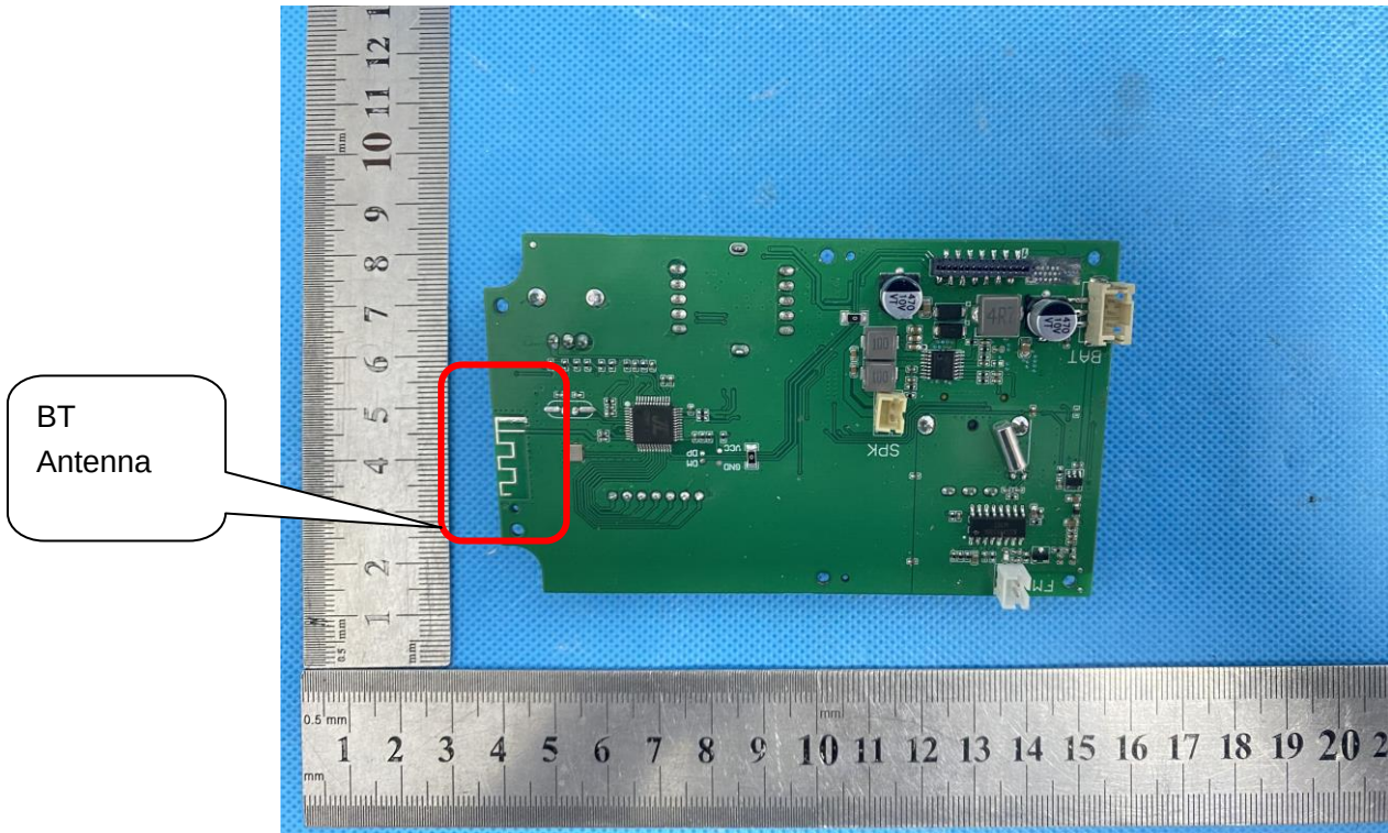
INTERNAL VIEW OF EUT (FIGURE 3)
