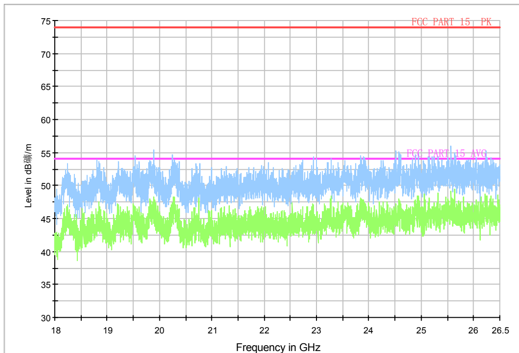
Fig.A.6.2.38 Transmitter Spurious Emission - Radiated (802.11n-HT40, Ch6, 18GHz –
