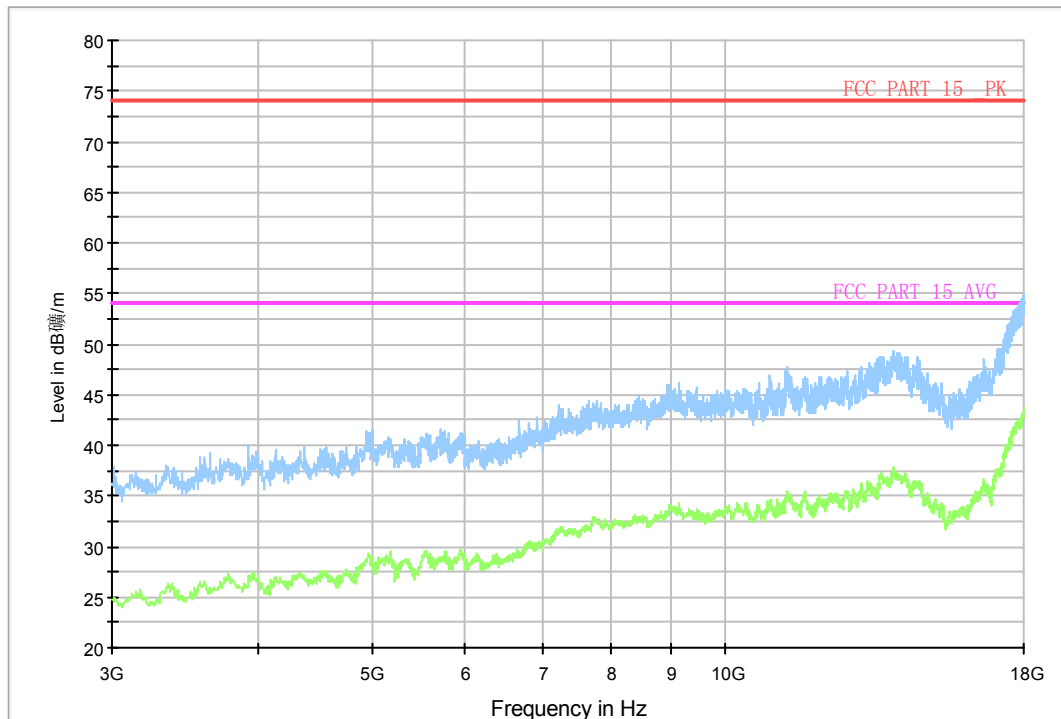
Normal RE_3G-18GHz
