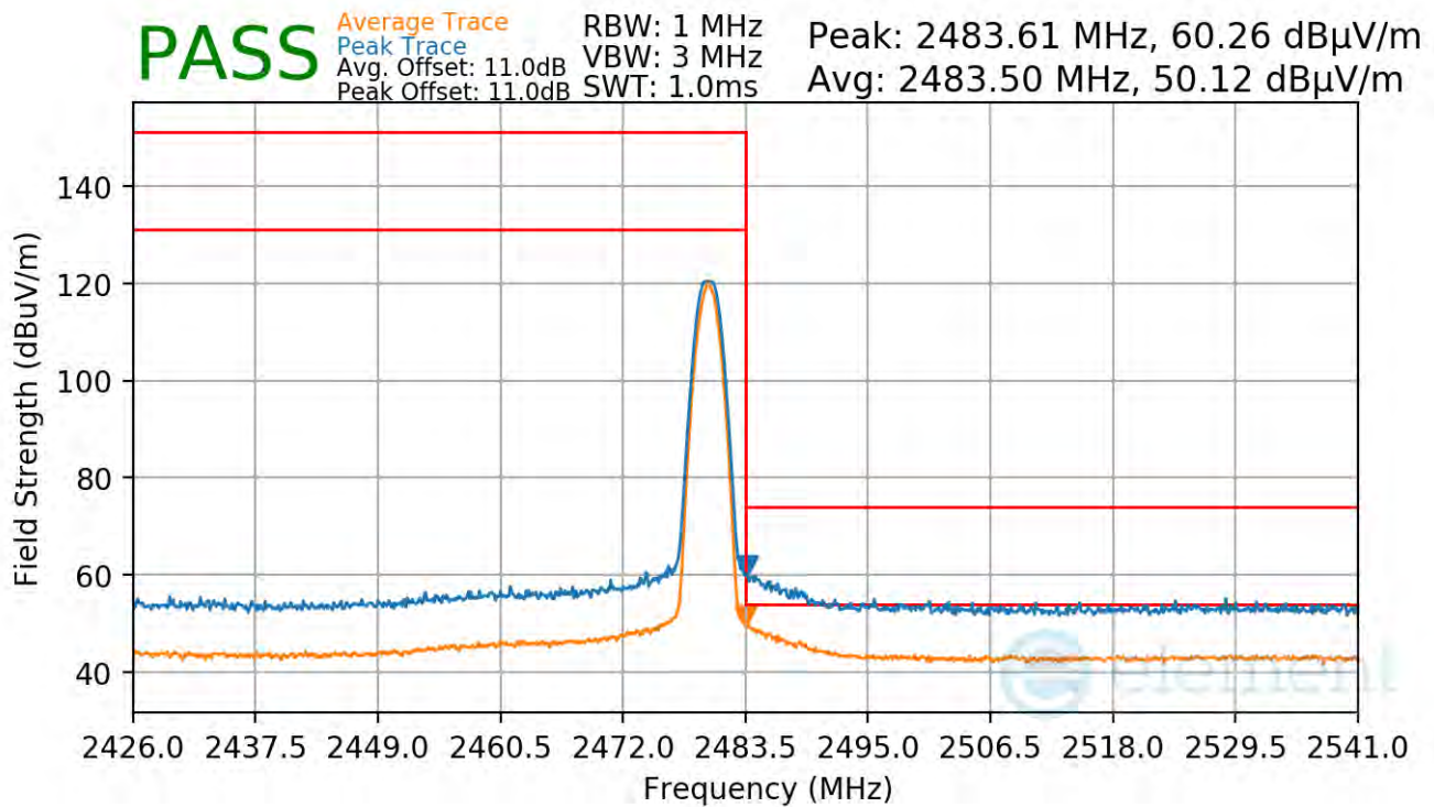
Plot 7-100. Radiated Restricted Upper Band Edge Measurement TxBF (Average & Peak)
