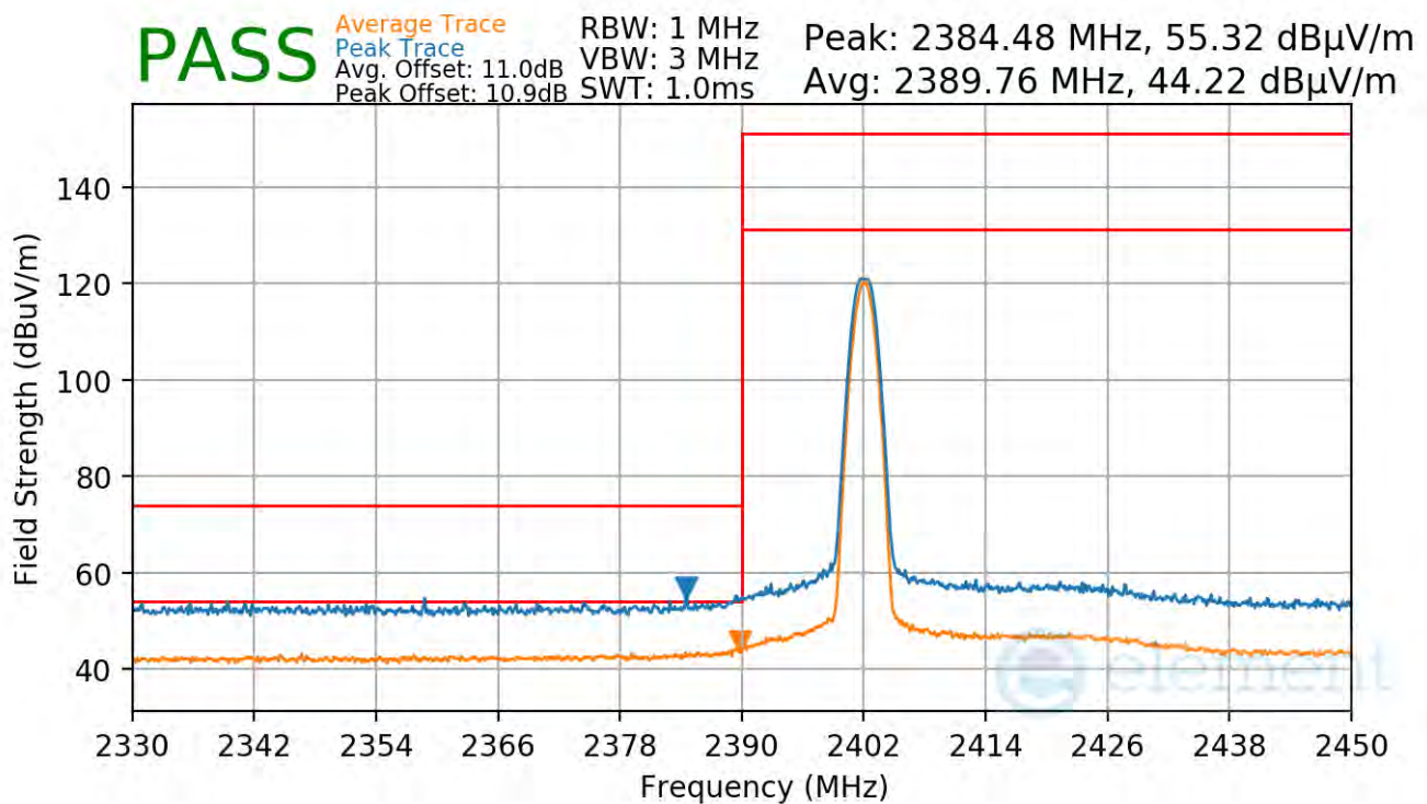
Plot 7-99. Radiated Restricted Lower Band Edge Measurement TxBF (Average & Peak)
