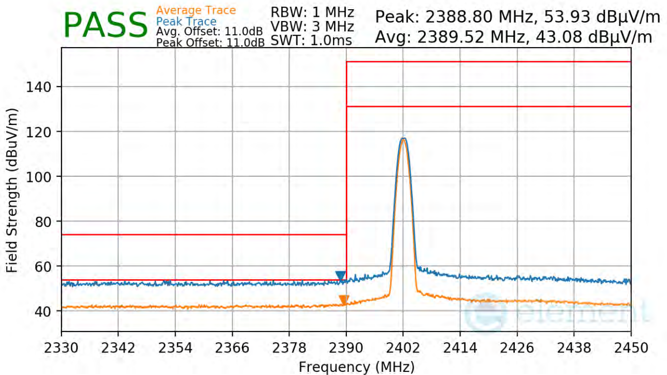
Plot 7-95. Radiated Restricted Lower Band Edge Measurement Antenna 2a (Average & Peak)
