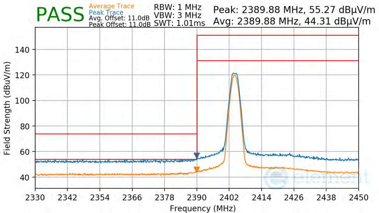
Plot 7-101. Radiated Restricted Lower Band Edge Measurement TxBF (Average & Peak)
