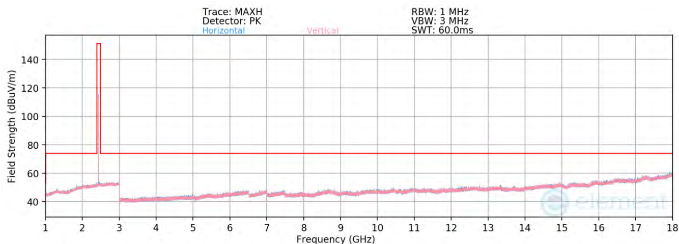
Plot 7-85. Radiated Spurious Emissions 1-18GHz Antenna 2a (1Mbps, ePA – Ch. 19)
