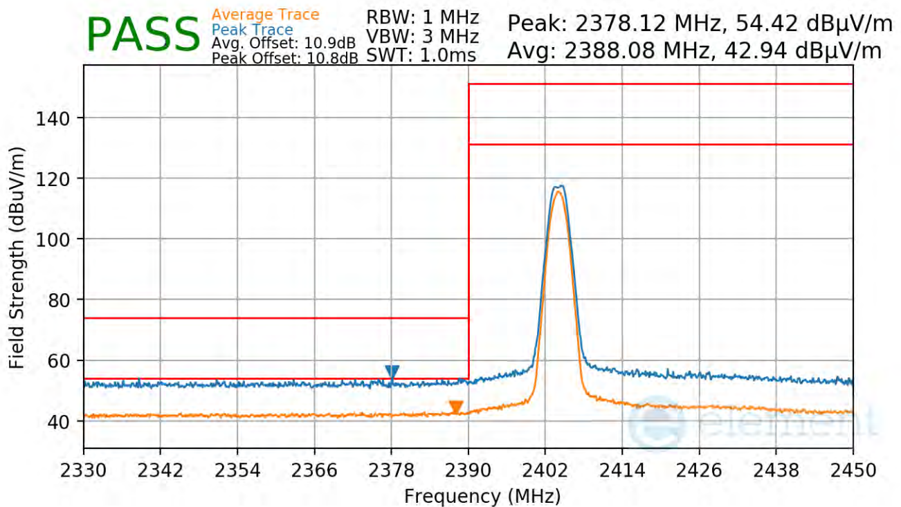
Plot 7-97. Radiated Restricted Lower Band Edge Measurement Antenna 2a (Average & Peak)
