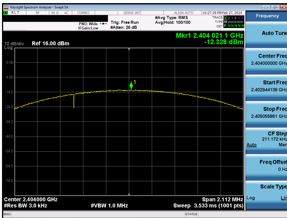
Plot 7-34. Power Spectral Density Plot Antenna 2a (Bluetooth (LE), 2Mbps, iPA – Ch. 1)
