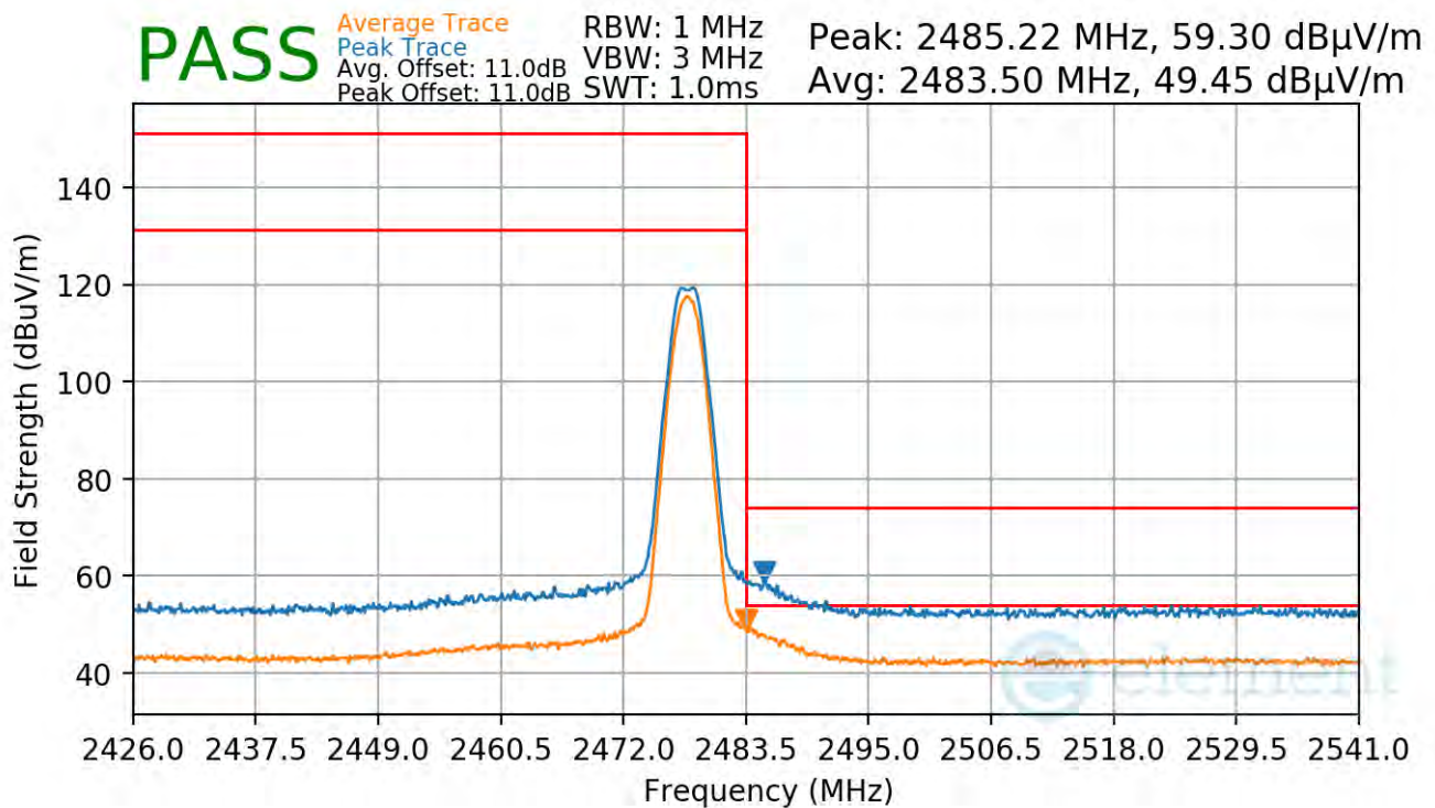
Plot 7-94. Radiated Restricted Upper Band Edge Measurement Antenna 4a (Average & Peak)
