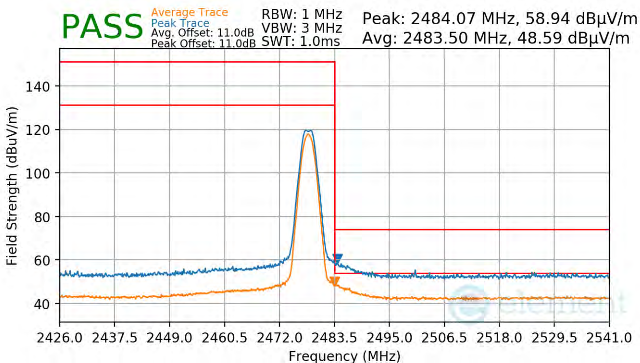
Plot 7-102. Radiated Restricted Upper Band Edge Measurement TxBF (Average & Peak)
