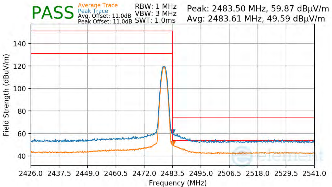
Plot 7-92. Radiated Restricted Upper Band Edge Measurement Antenna 4a (Average & Peak)
