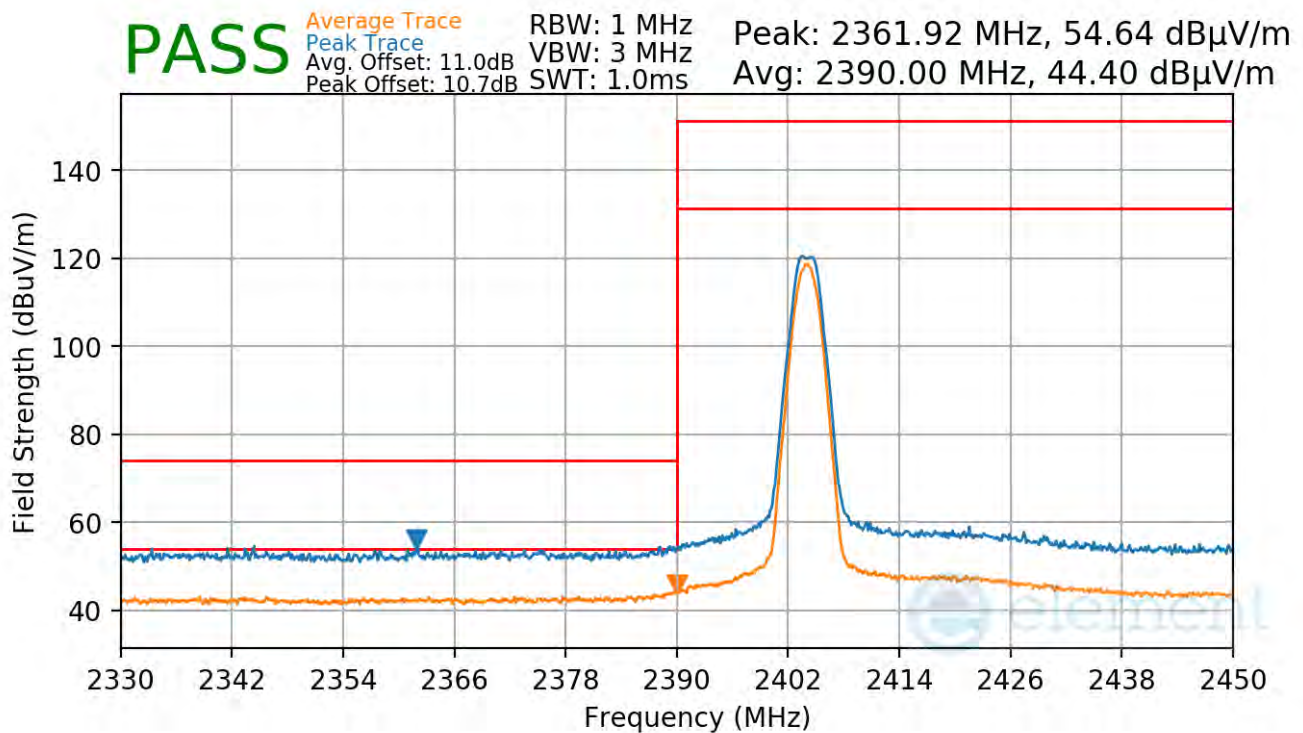
Plot 7-93. Radiated Restricted Lower Band Edge Measurement Antenna 4a (Average & Peak)
