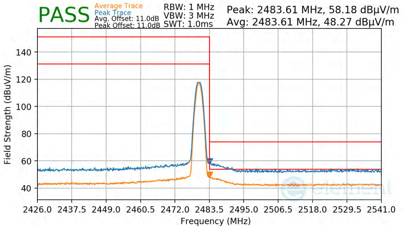
Plot 7-96. Radiated Restricted Upper Band Edge Measurement Antenna 2a (Average & Peak)
