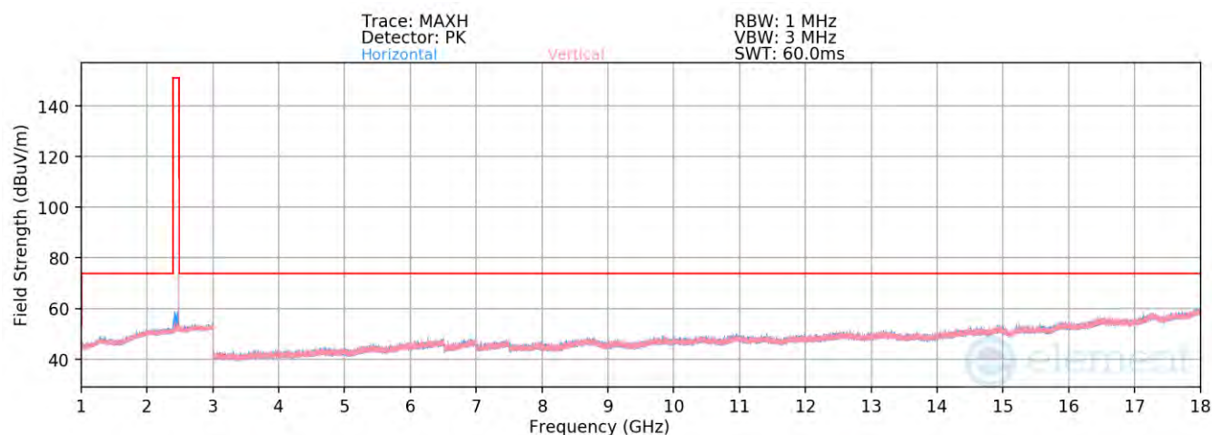
Plot 7-90. Radiated Spurious Emissions 1-18GHz TxBF (1Mbps ePA – Ch. 39)
