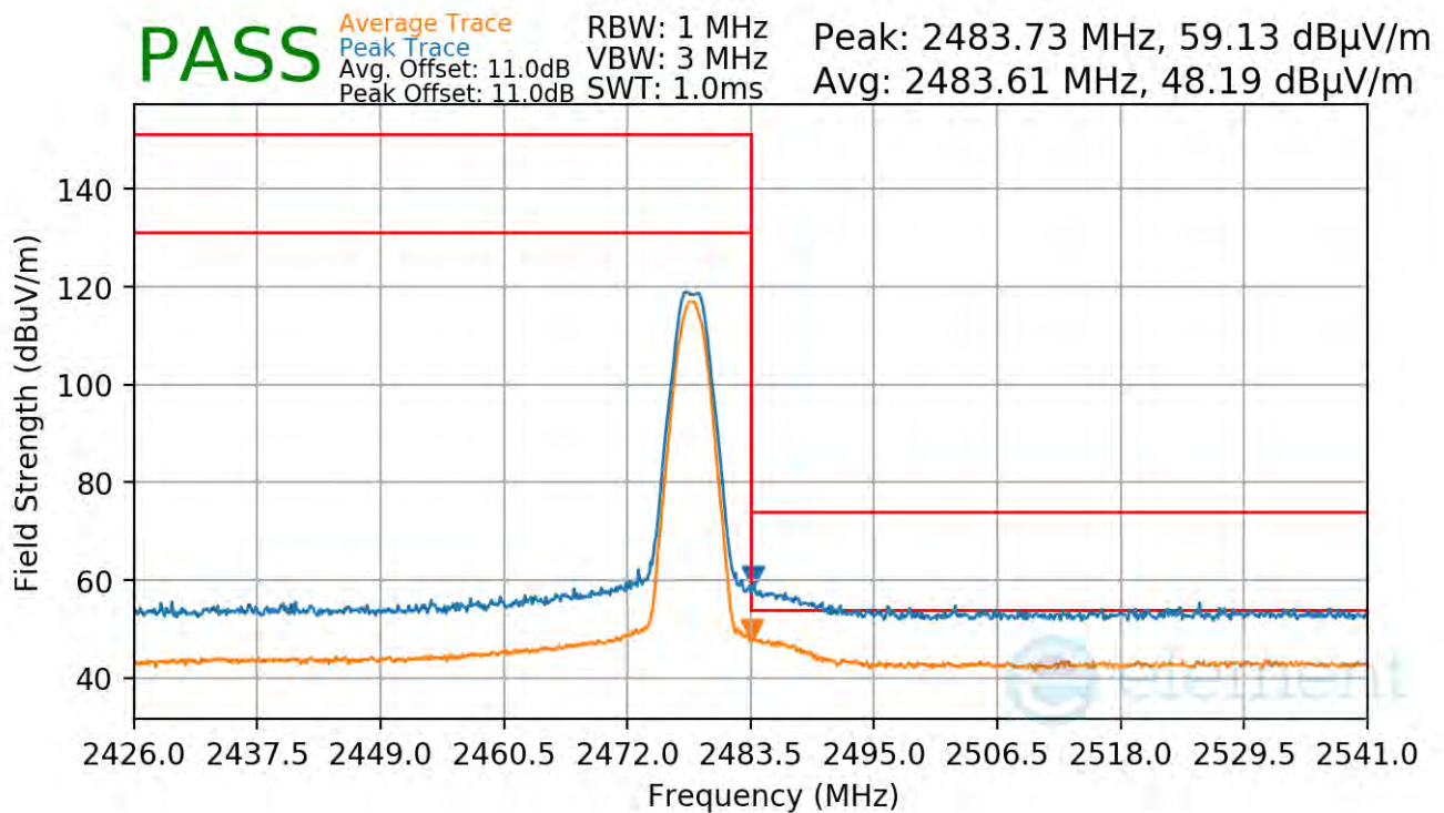
Plot 7-98. Radiated Restricted Upper Band Edge Measurement Antenna 2a (Average & Peak)
