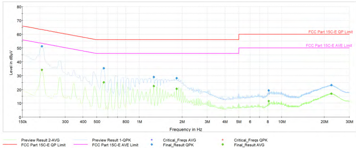
Plot 7-104. AC Line Conducted Plot with Bluetooth LE Tx BF (L1, 1Mbps ePA – Ch.19 with AC/DC Adapter)
