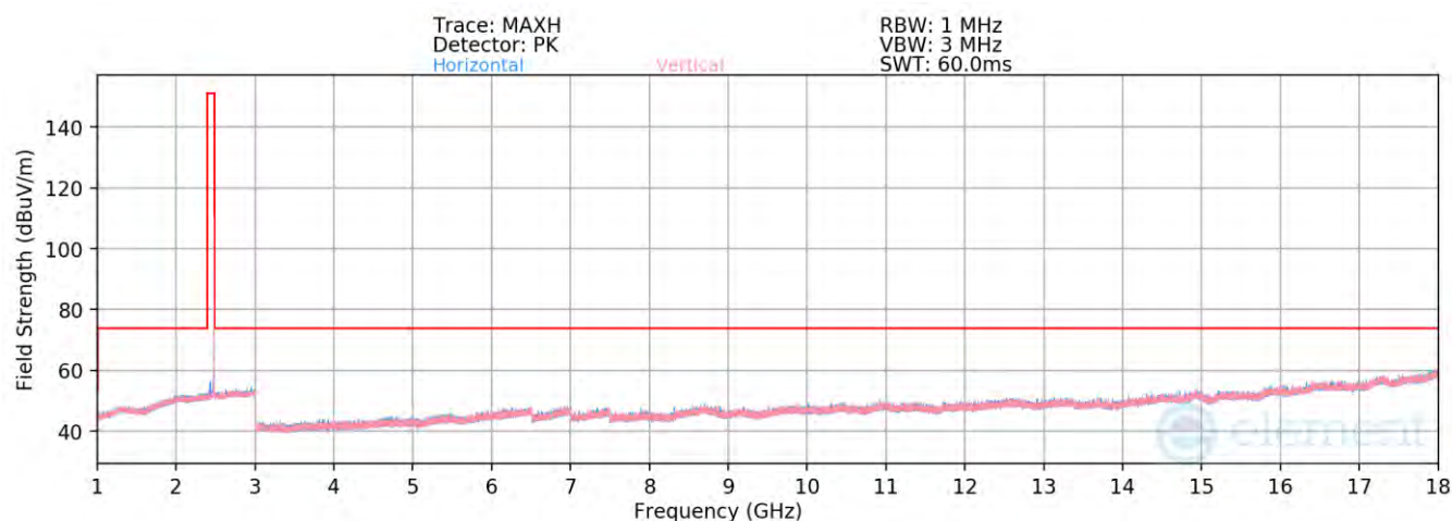
Plot 7-83. Radiated Spurious Emissions 1-18GHz Antenna 4a (1Mbps ePA – Ch. 39)
