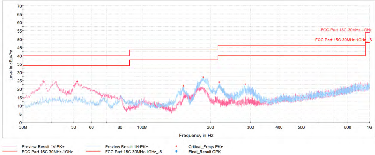
Plot 7-103. Radiated Spurious Emissions Below 1GHz TxBF (1Mbps, ePA – Ch.19, Pol. H & V, with AC/DC Adapter)
