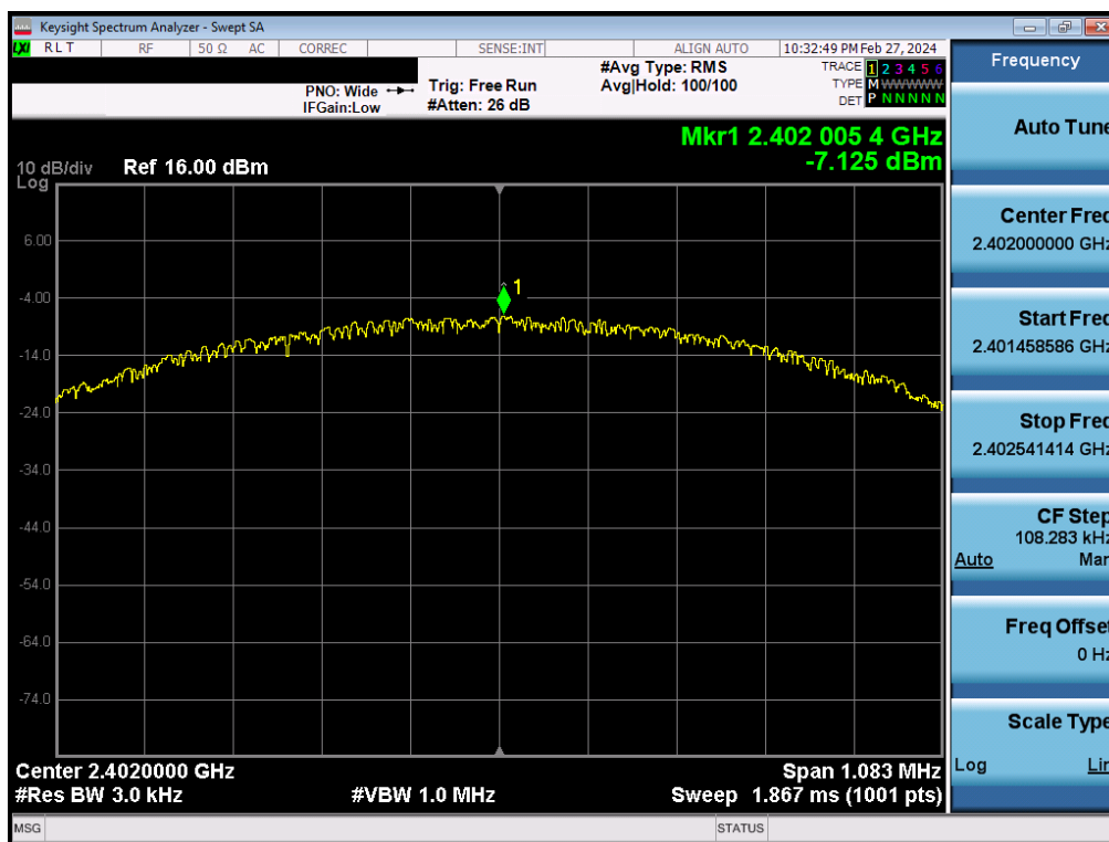
Plot 7-44. Power Spectral Density Plot Antenna 2a (Bluetooth (LE), 1Mbps, iPA – Ch. 0)
