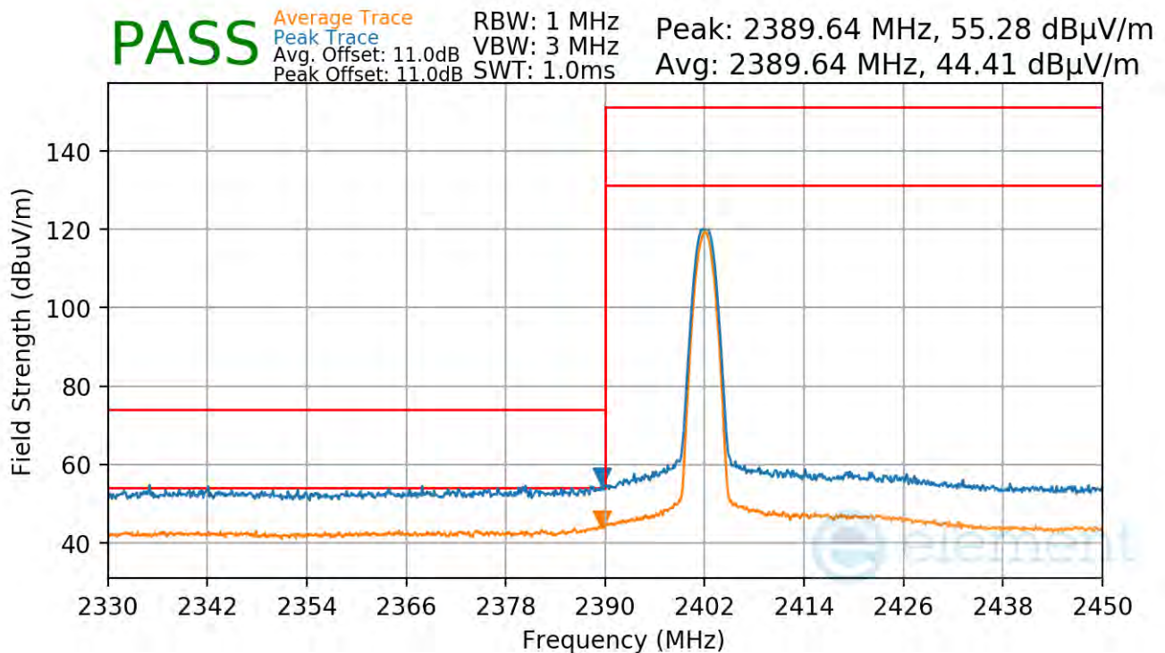
Plot 7-91. Radiated Restricted Lower Band Edge Measurement Antenna 4a (Average & Peak)
