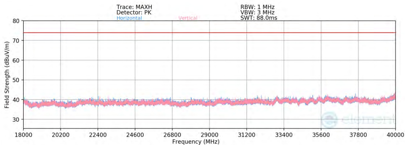
Plot 7-89. Radiated Spurious Emissions Above 18GHz TxBF (1Mbps, ePA – Ch. 19)
