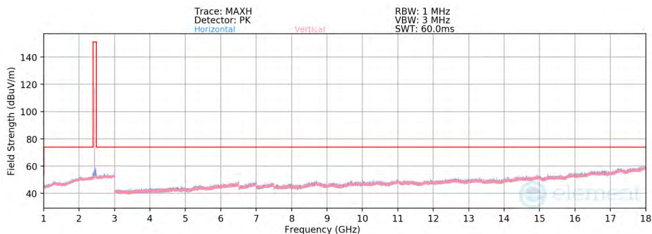
Plot 7-88. Radiated Spurious Emissions 1-18GHz TxBF (1Mbps, ePA – Ch. 19)
