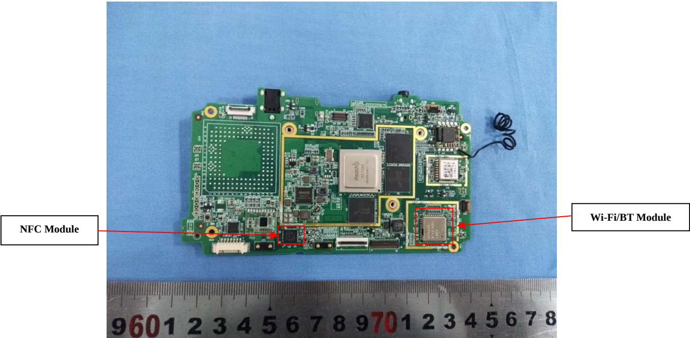
EUT – Mainboard Top Uncovered View
