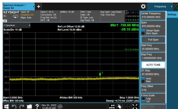
CH78 (2480MHz) 3-DH5(3Mbps)
