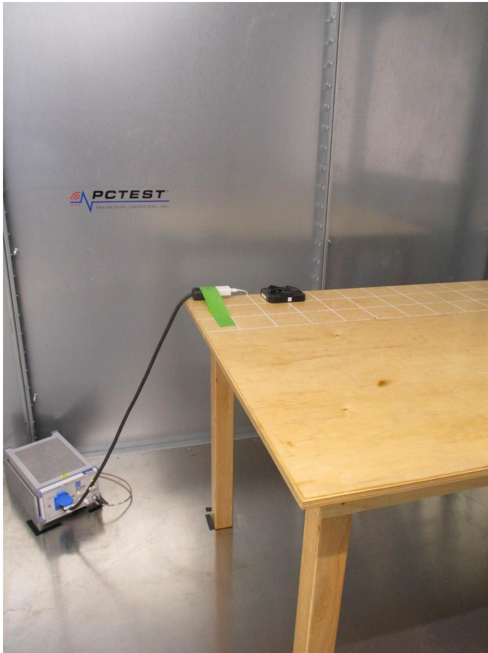
Figure 1: AC Line Conducted Emissions (Front View)
