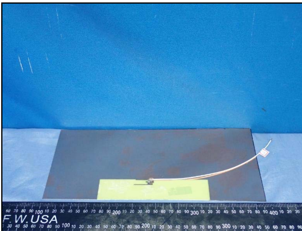
Antenna 3 (Model: 260-25084)
