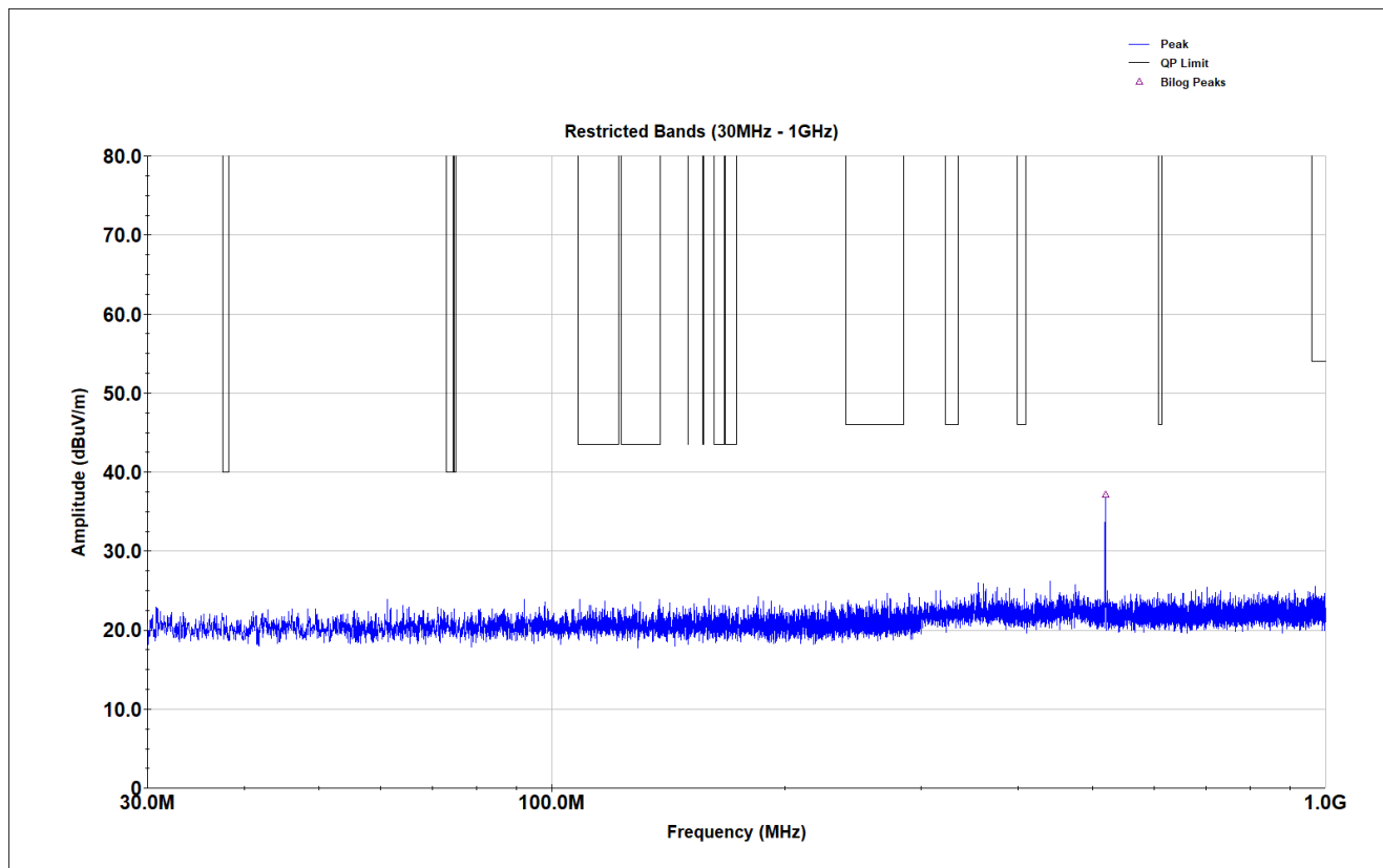
Figure 15. High Channel, 30MHz – 1GHz Restricted Band Spurious Emissions (2Mbps)
