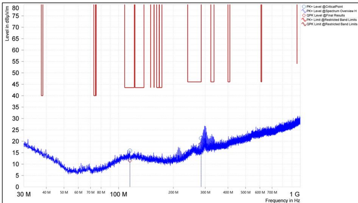
Figure 25. Worst Case Cabinet Radiation, 30MHz – 1GHz, Horizontal Polarity (2MBps)
