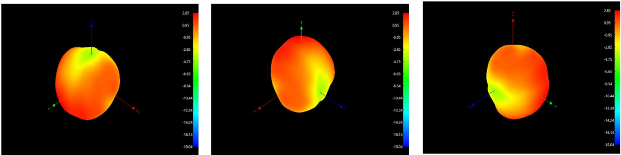
Antenna 3D 5200MHz:
